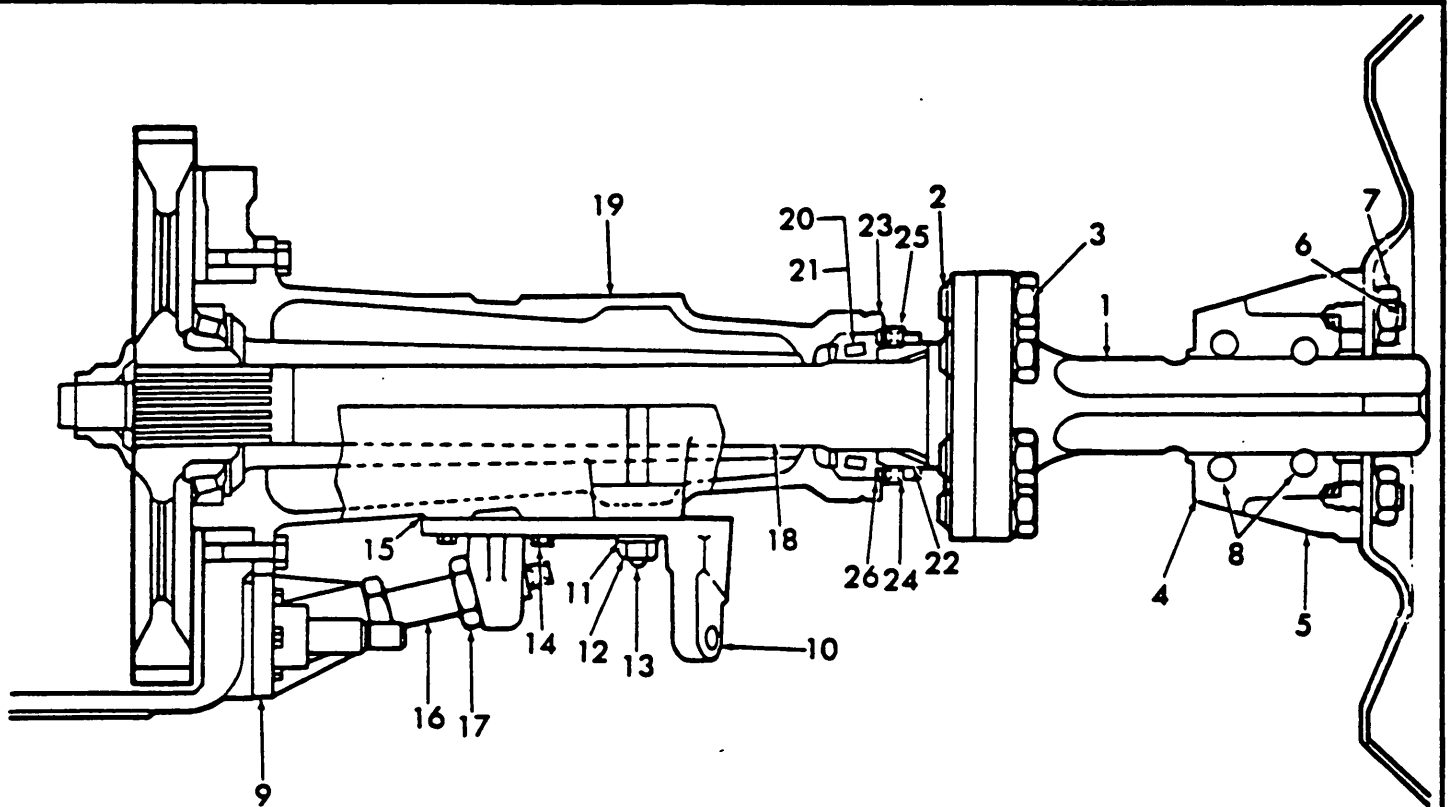
Fig. 25 - Rowcrop Rear Axle Extension
