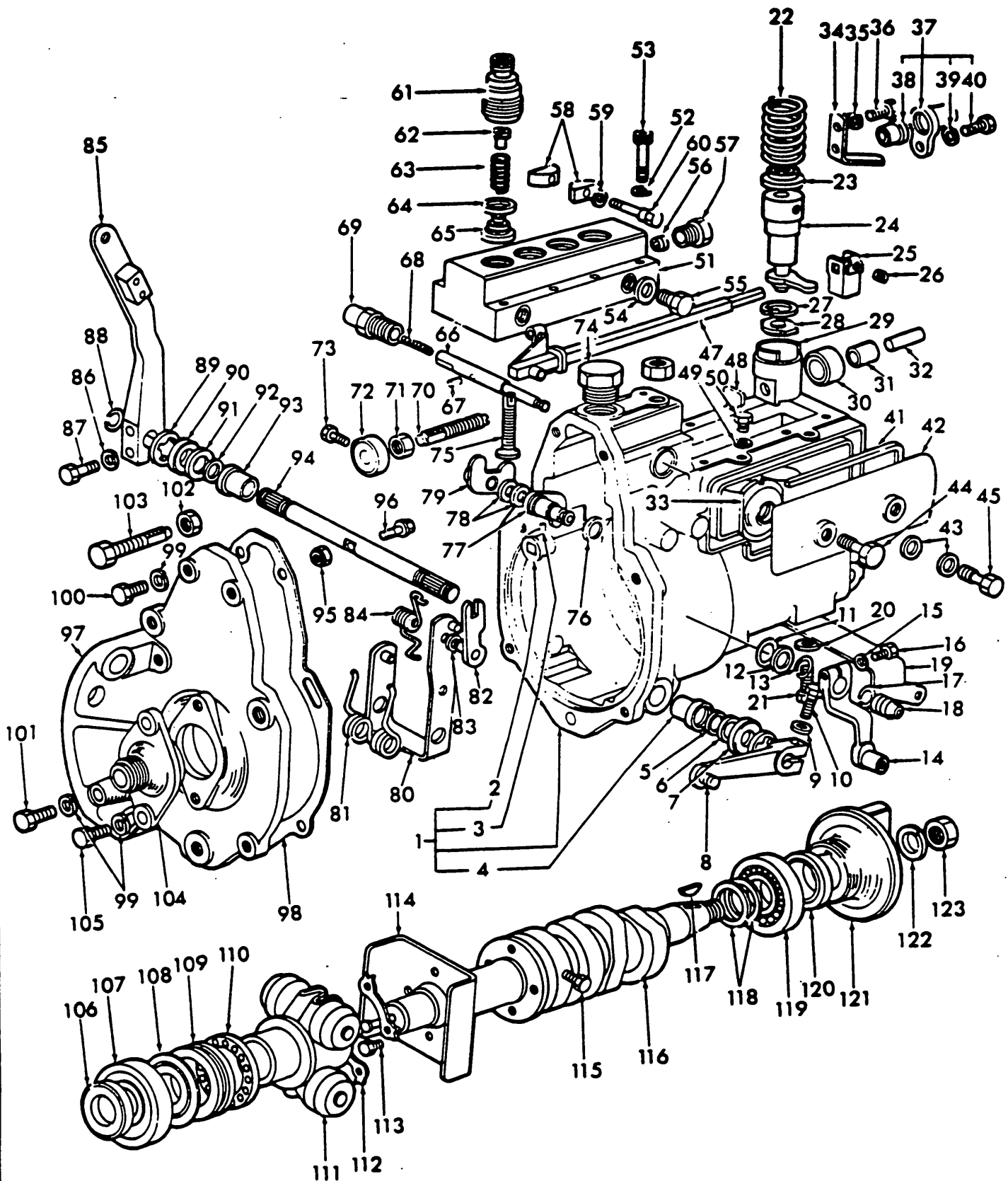
Fig. 70 - Fuel Injection Pump w/Mechanical Gov. 4-62/64
