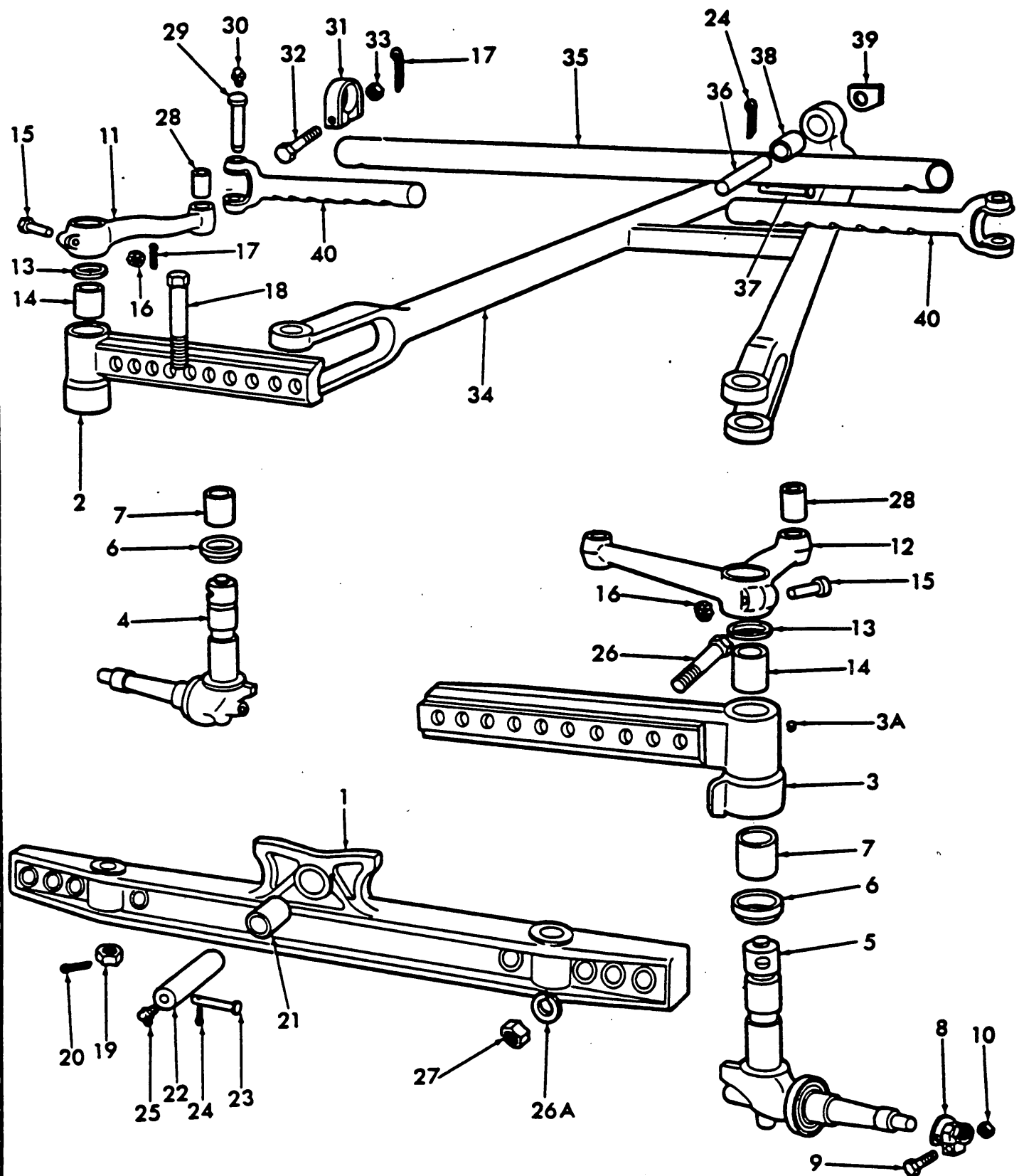
Fig. 11 - Front Axle
