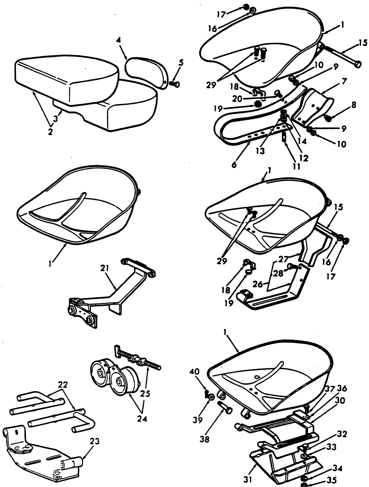
Fig. 88 - Seat Assemblies
