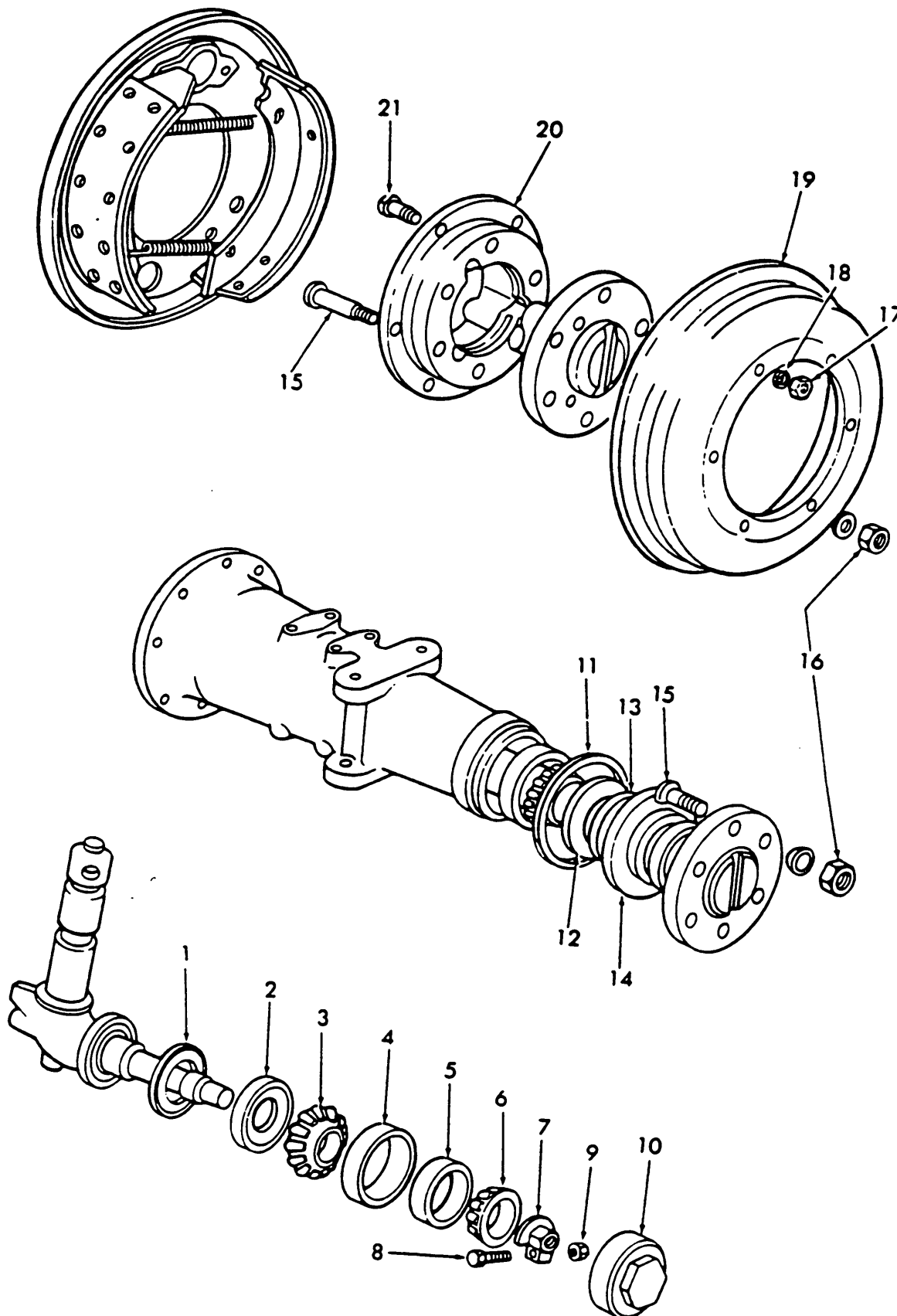
Fig. 4 - Hub & Drums
