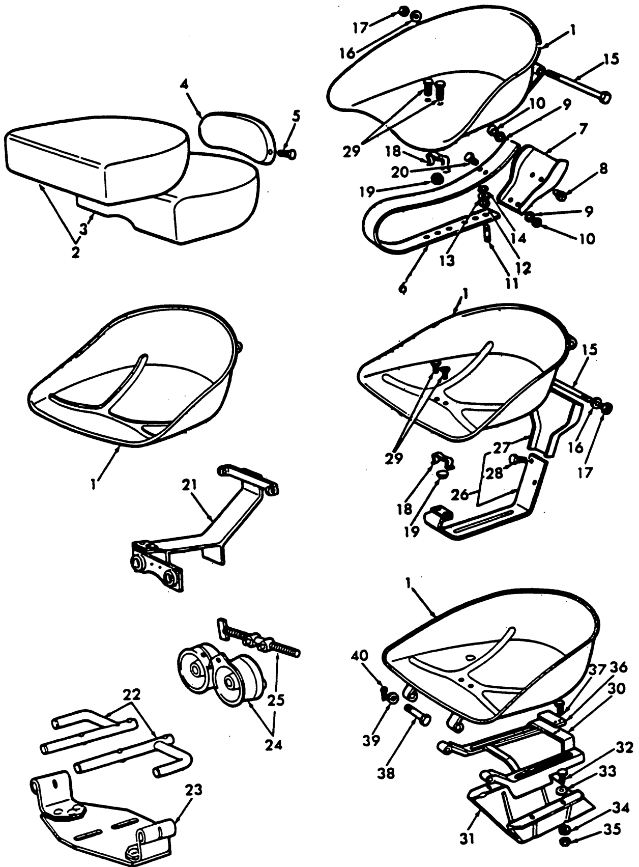
Fig. 88 - Seat Assemblies
