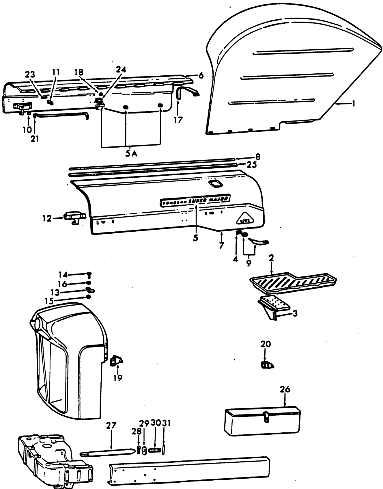
Fig. 89 - Mudguards & Bonnets
