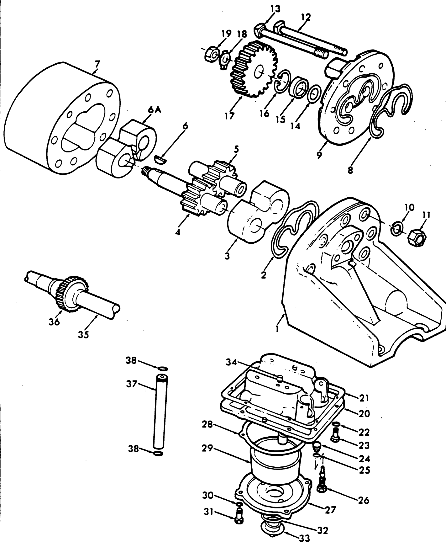
Fig. 38 - Hydraulic Pump Assy.
