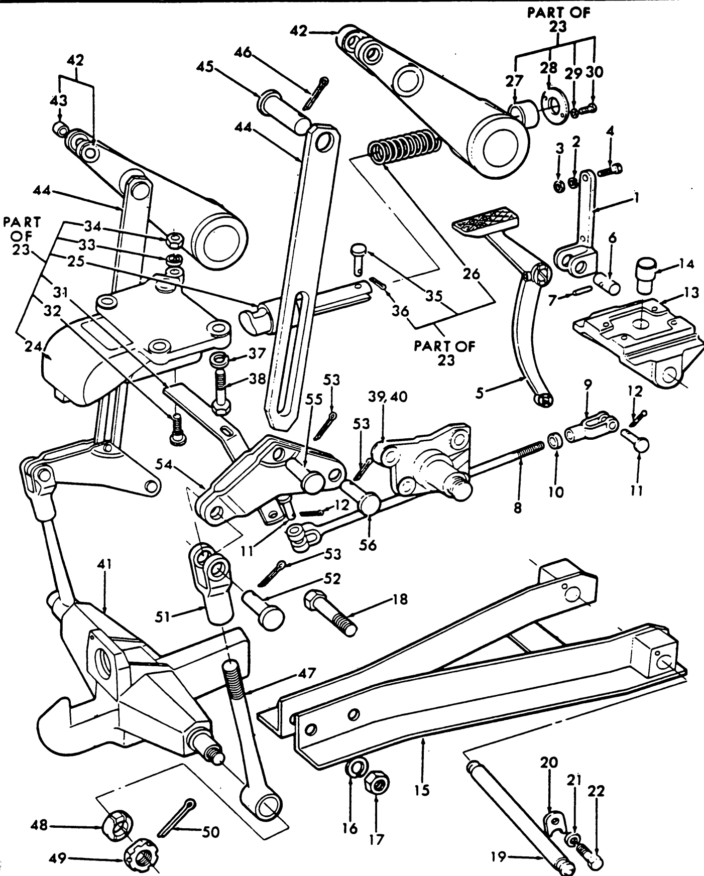
Fig. 34 - Automatic Hitch 11-60/64
