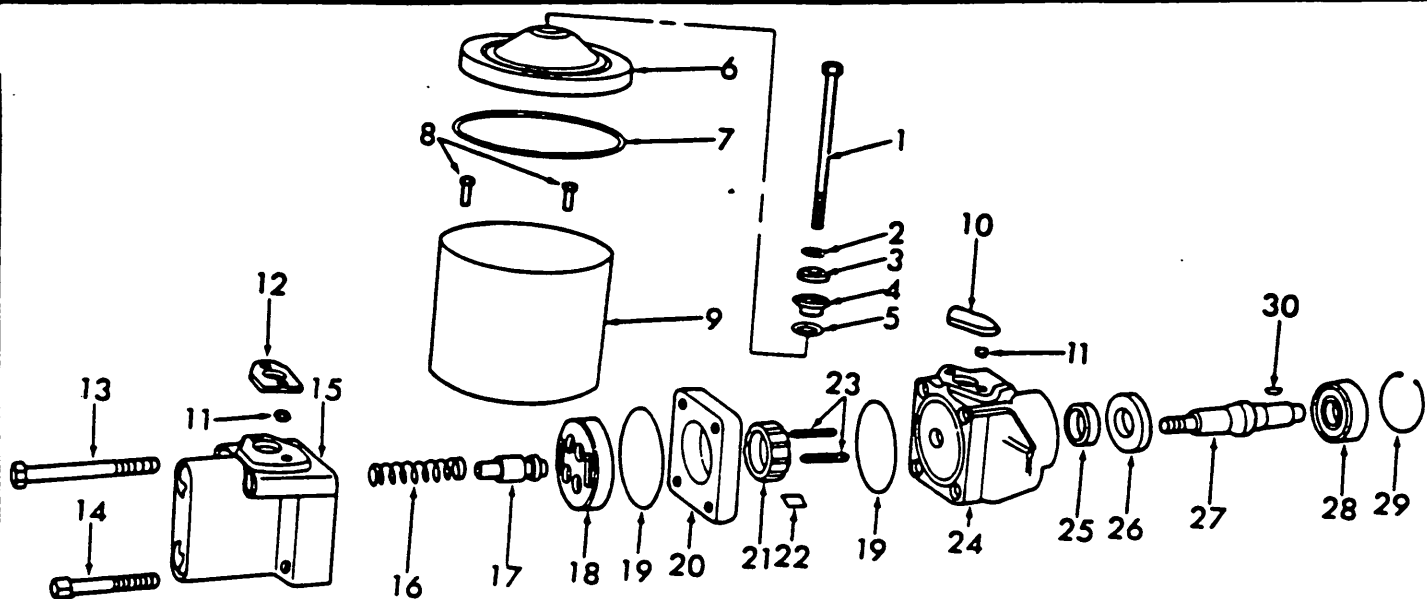
Fig. 17 — Power Steering Pump D415
