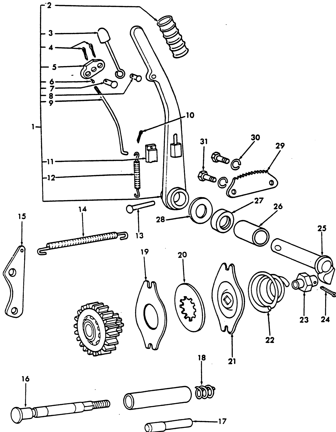
Fig. 10— Transmission Handbrake
