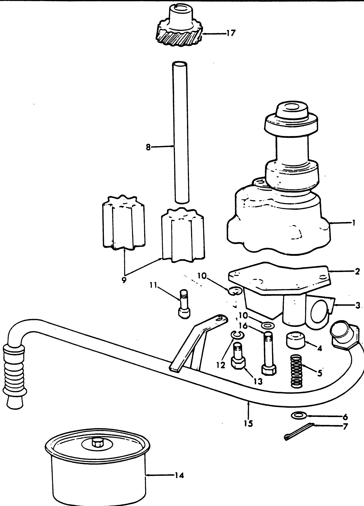
Fig. 45 - Oil Pump Assy. & Related Parts
