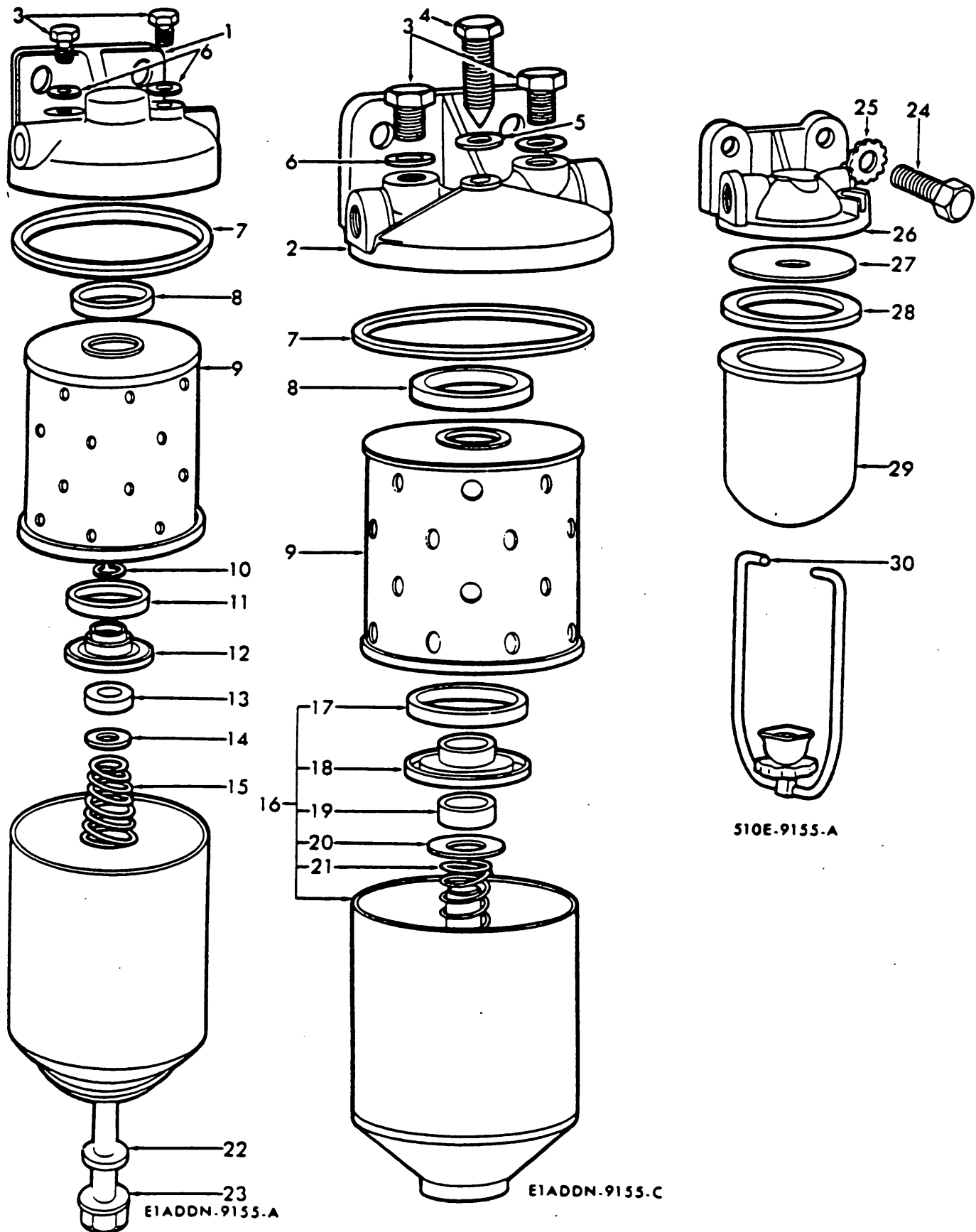
Fig. 62 - Fuel Oil Filters
