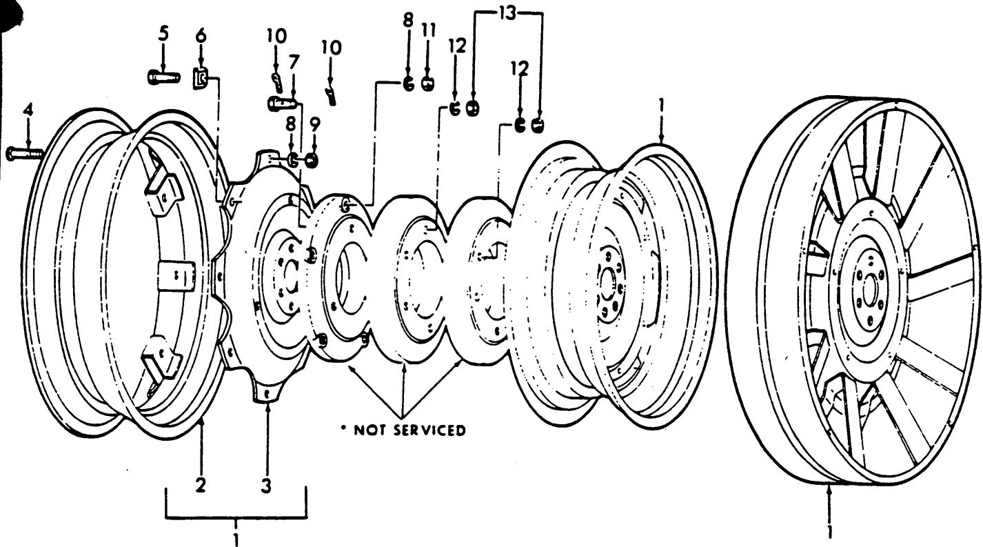
Fig. 2 — Rear Wheels
