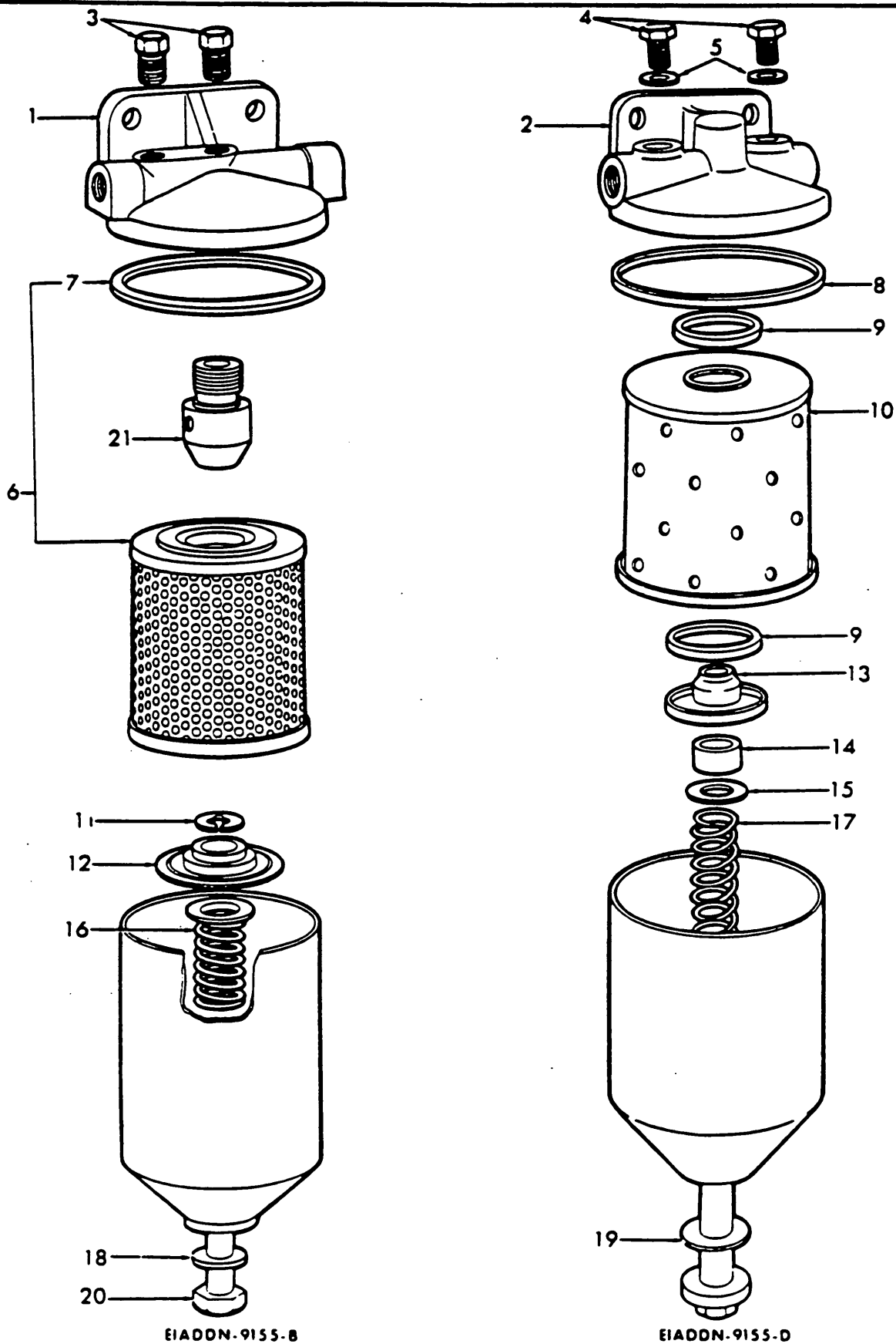
Fig. 61 - Fuel Oil Filters
