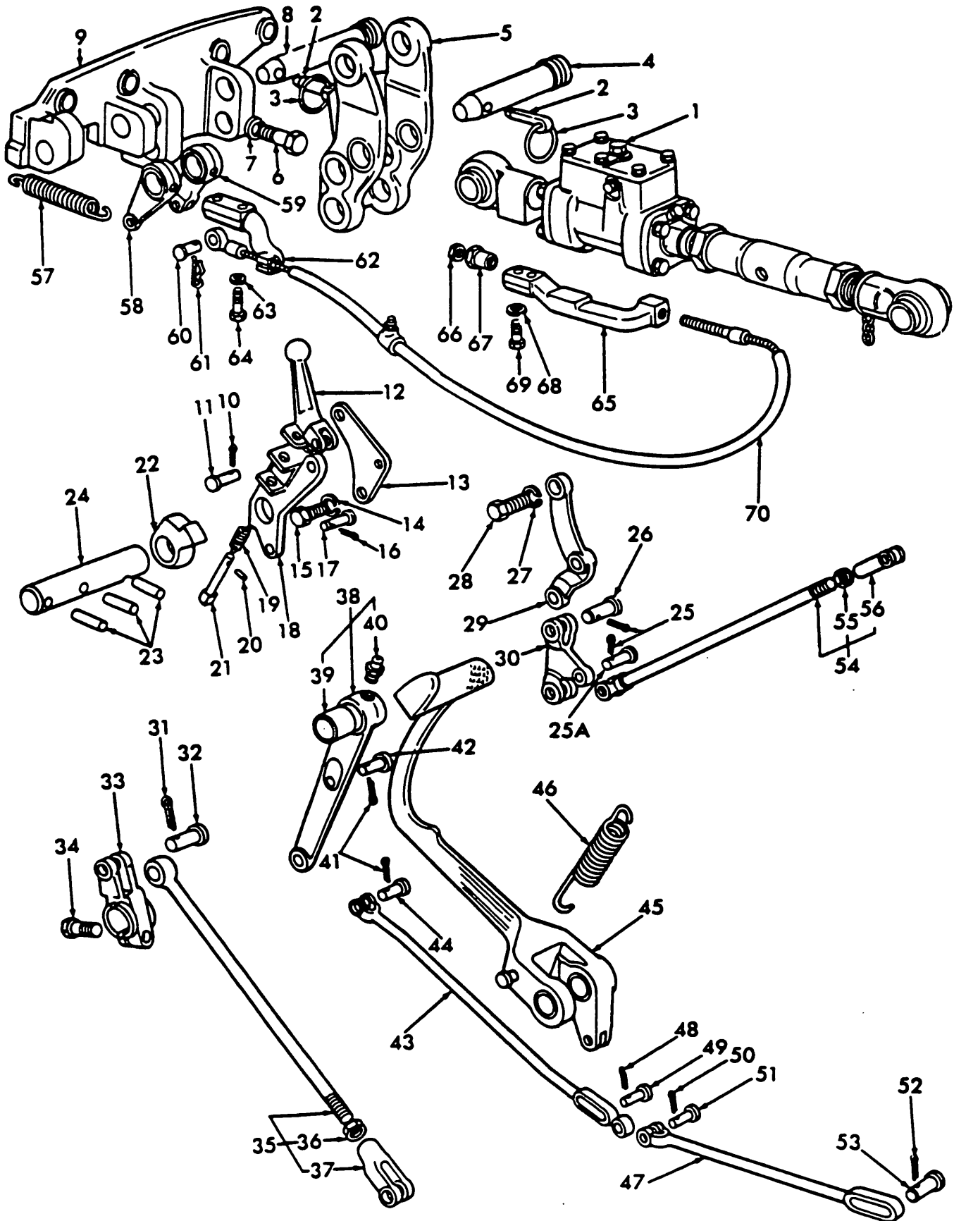
Fig. 36 - Automatic Clutch Release
