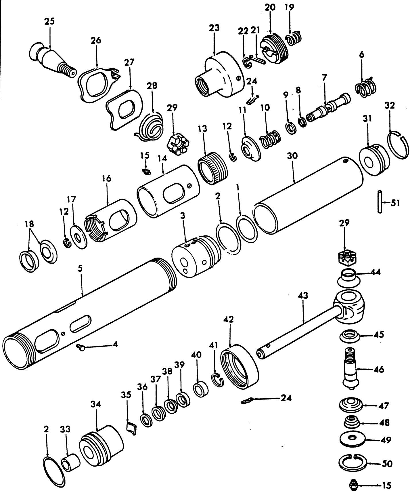
Fig. 18 - Power Steering Cylinder Booster D502
