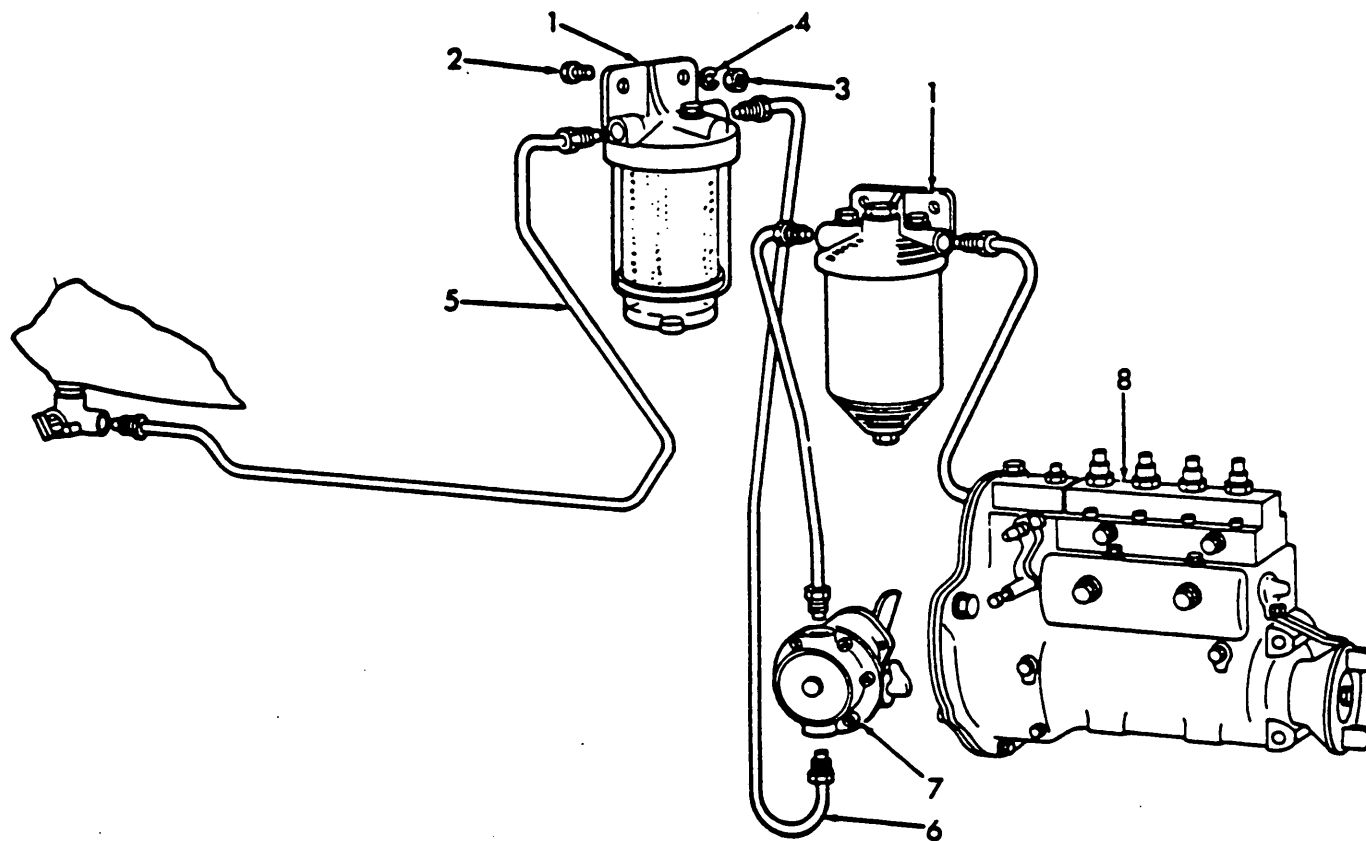
Fig. 63 - Dual Fuel Oil Filters
