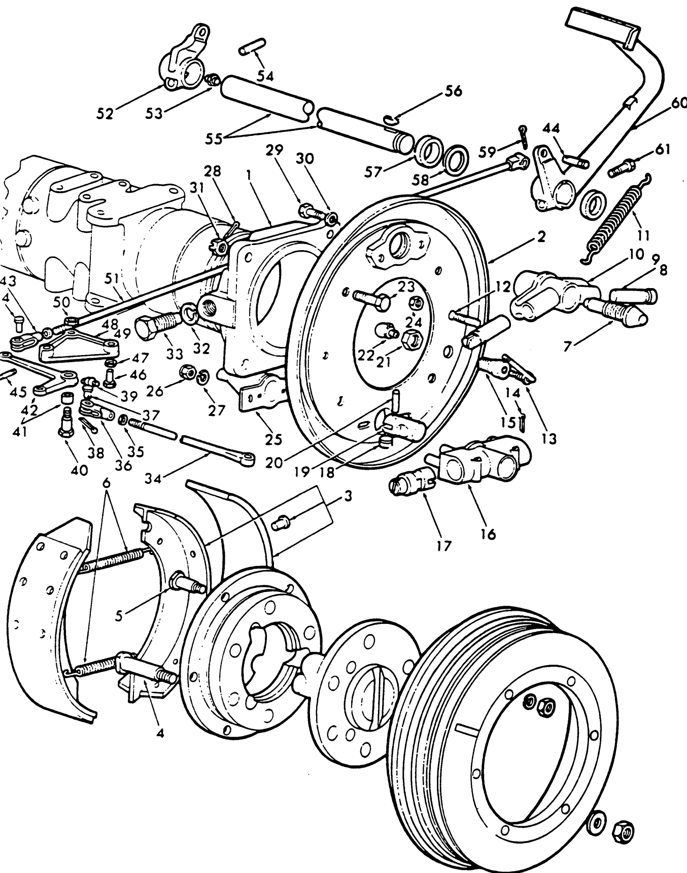
Fig. 5 - Rear Wheel Brakes - Industrial Tractor
