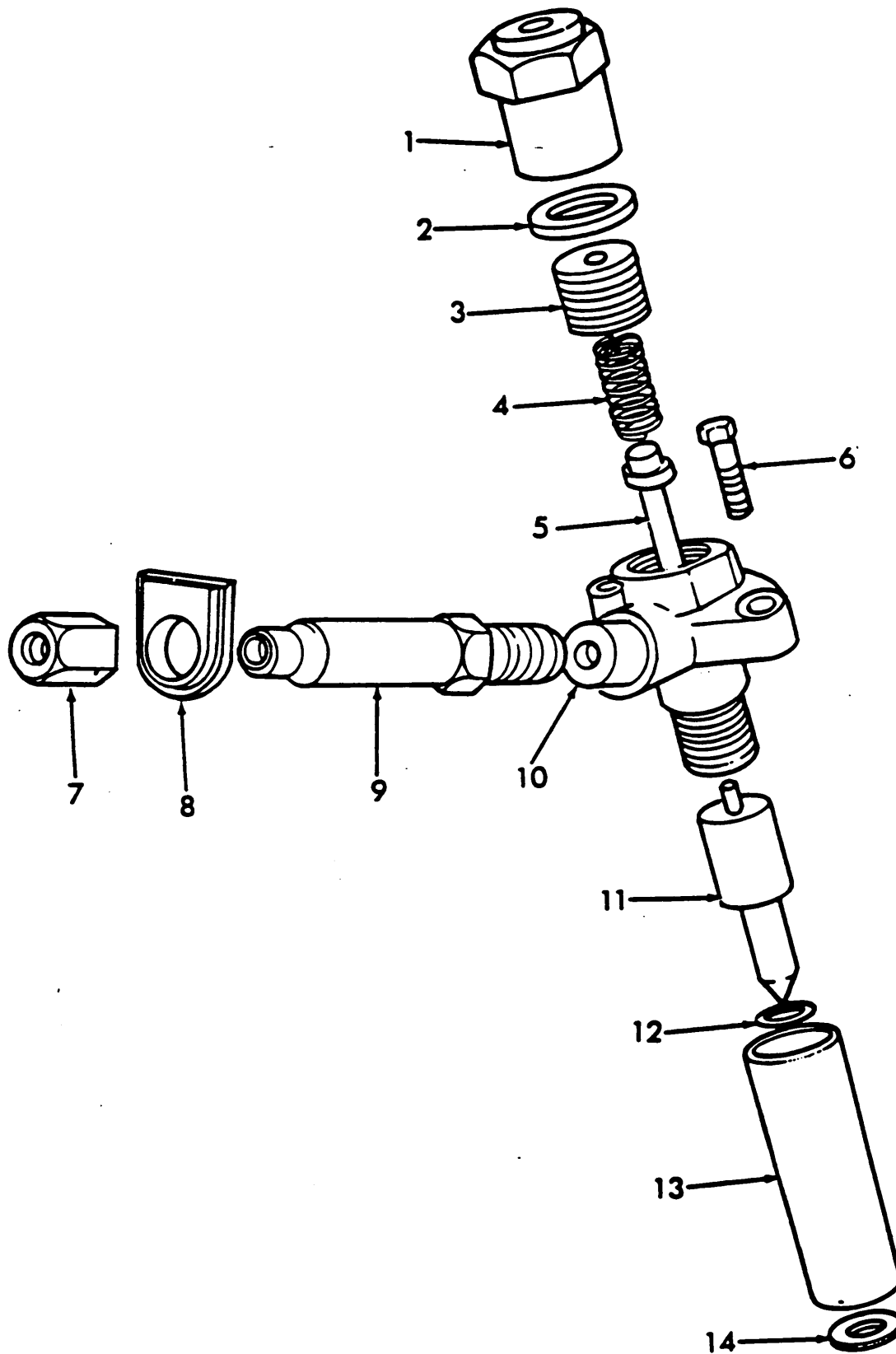
Fig. 72 - Fuel Injector
