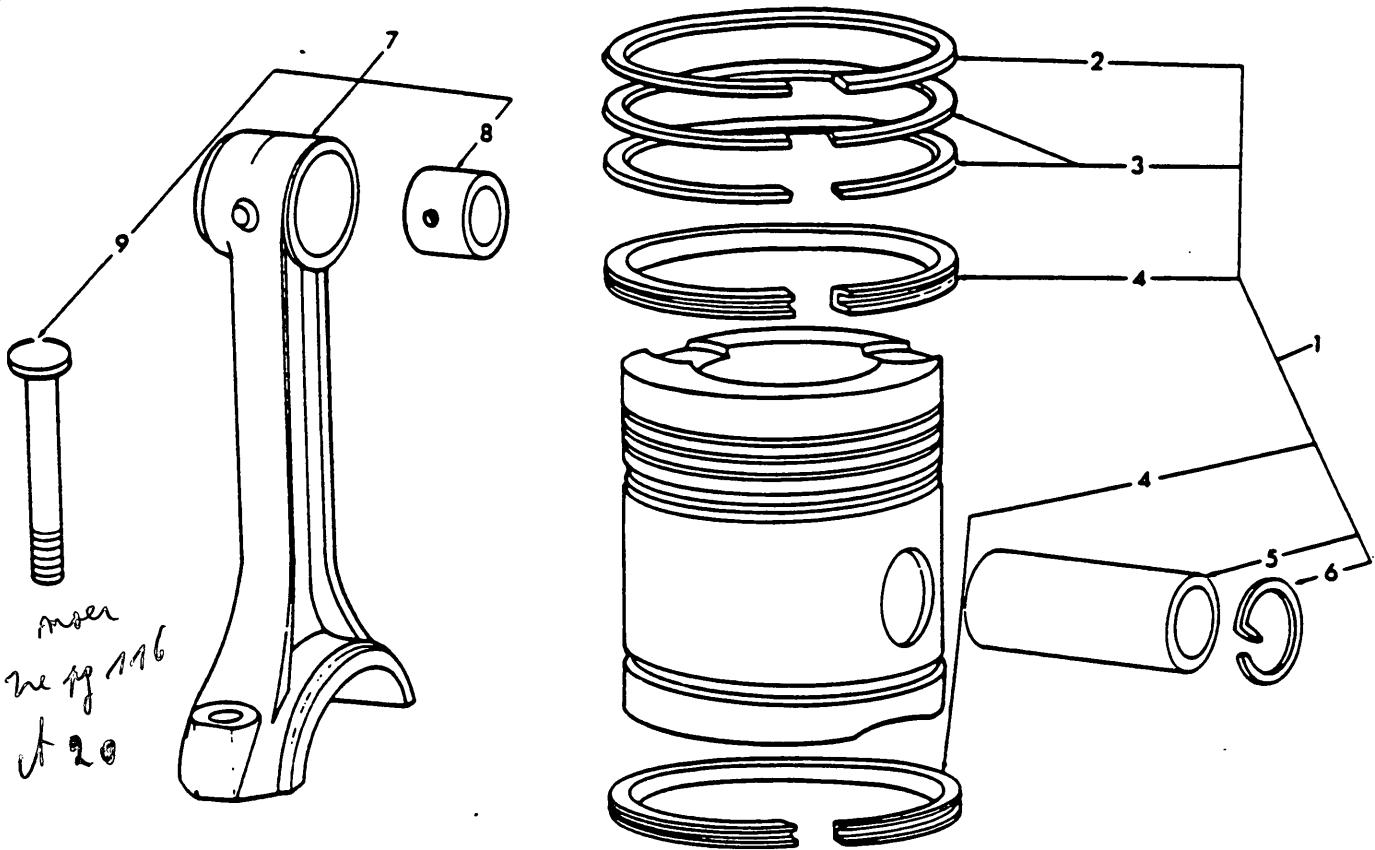
Fig. 44 — Pistons & Connecting Rods
