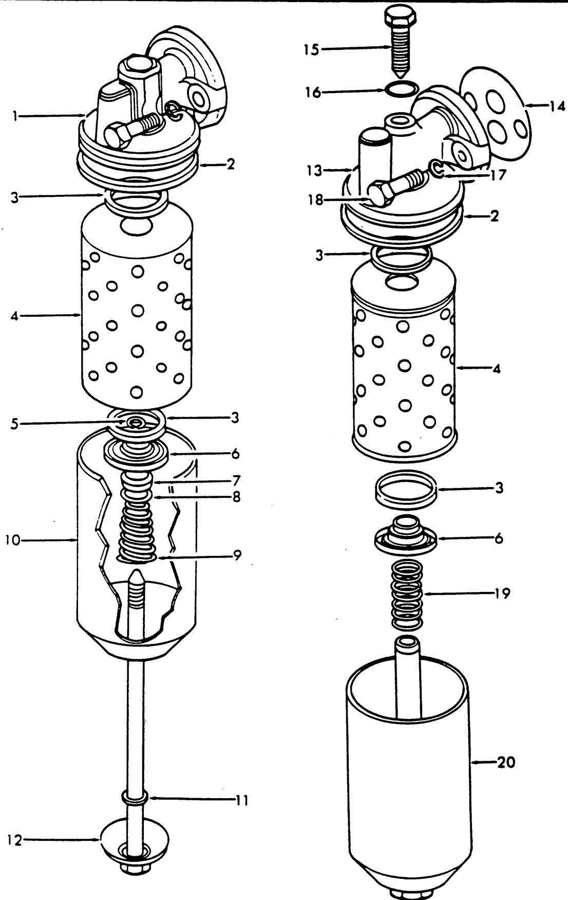
Fig. 46 - Engine Oil Filters
