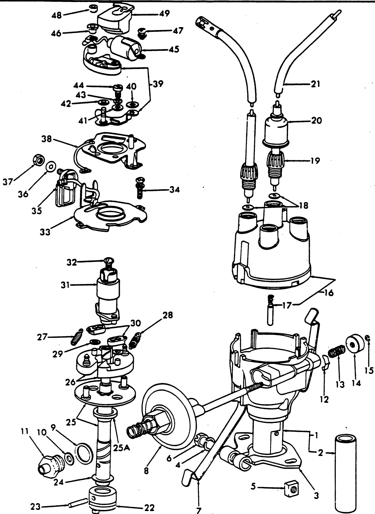
Fig. 81 - Distributor
