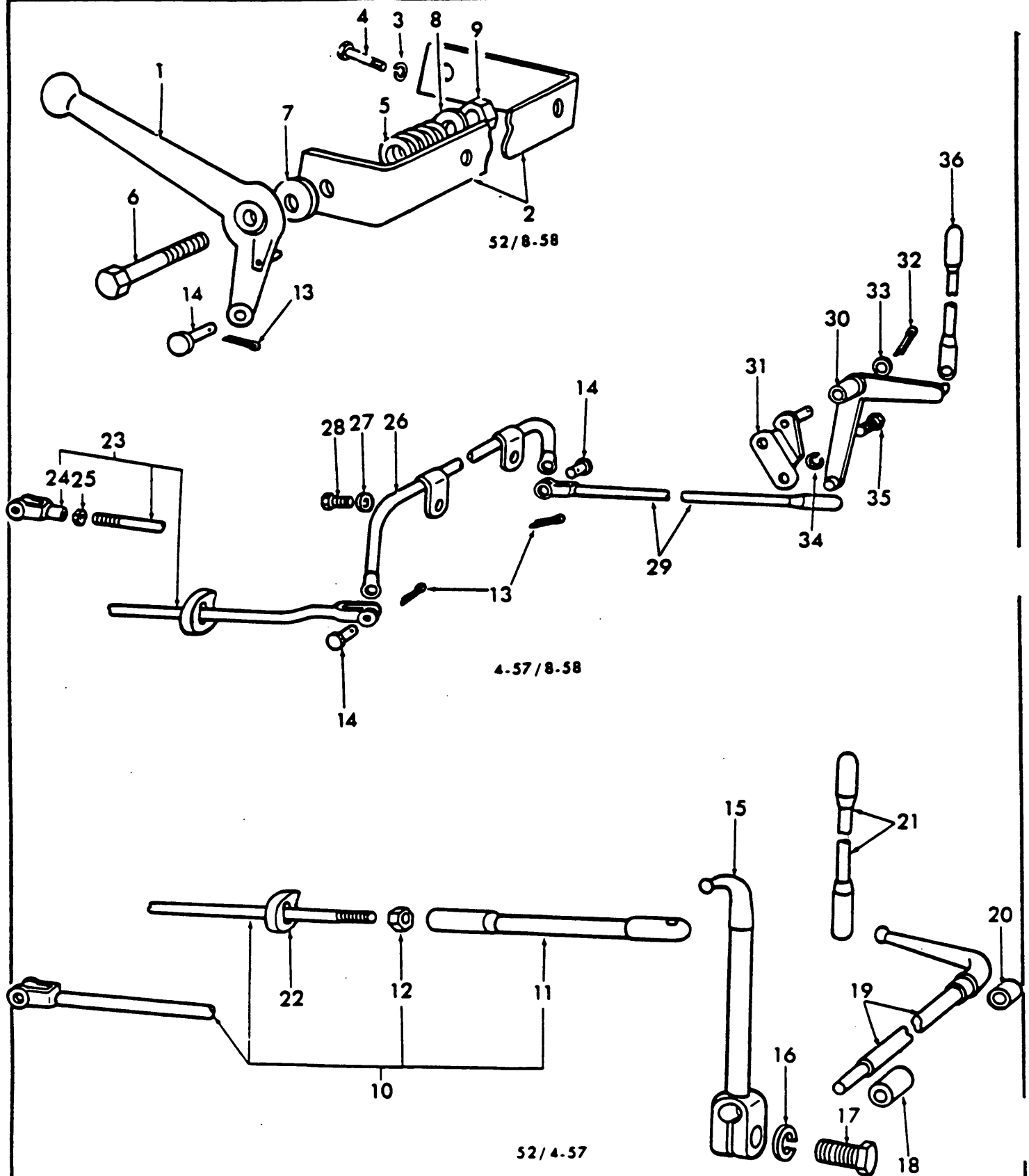
Fig. 65 - Throttle Linkage 52/8-58
