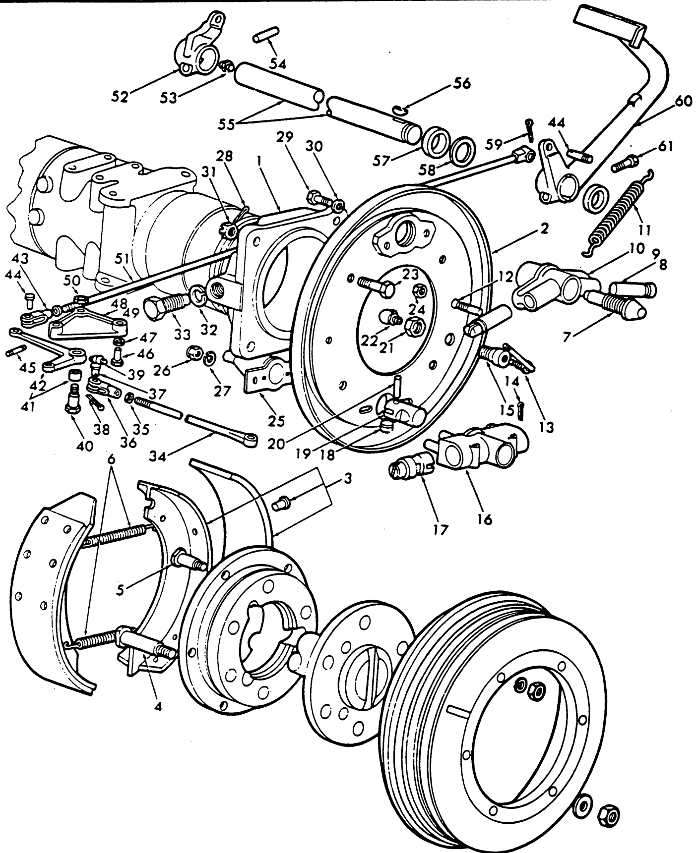
Fig. 5 — Rear Wheel Brakes - Industrial Tractor
