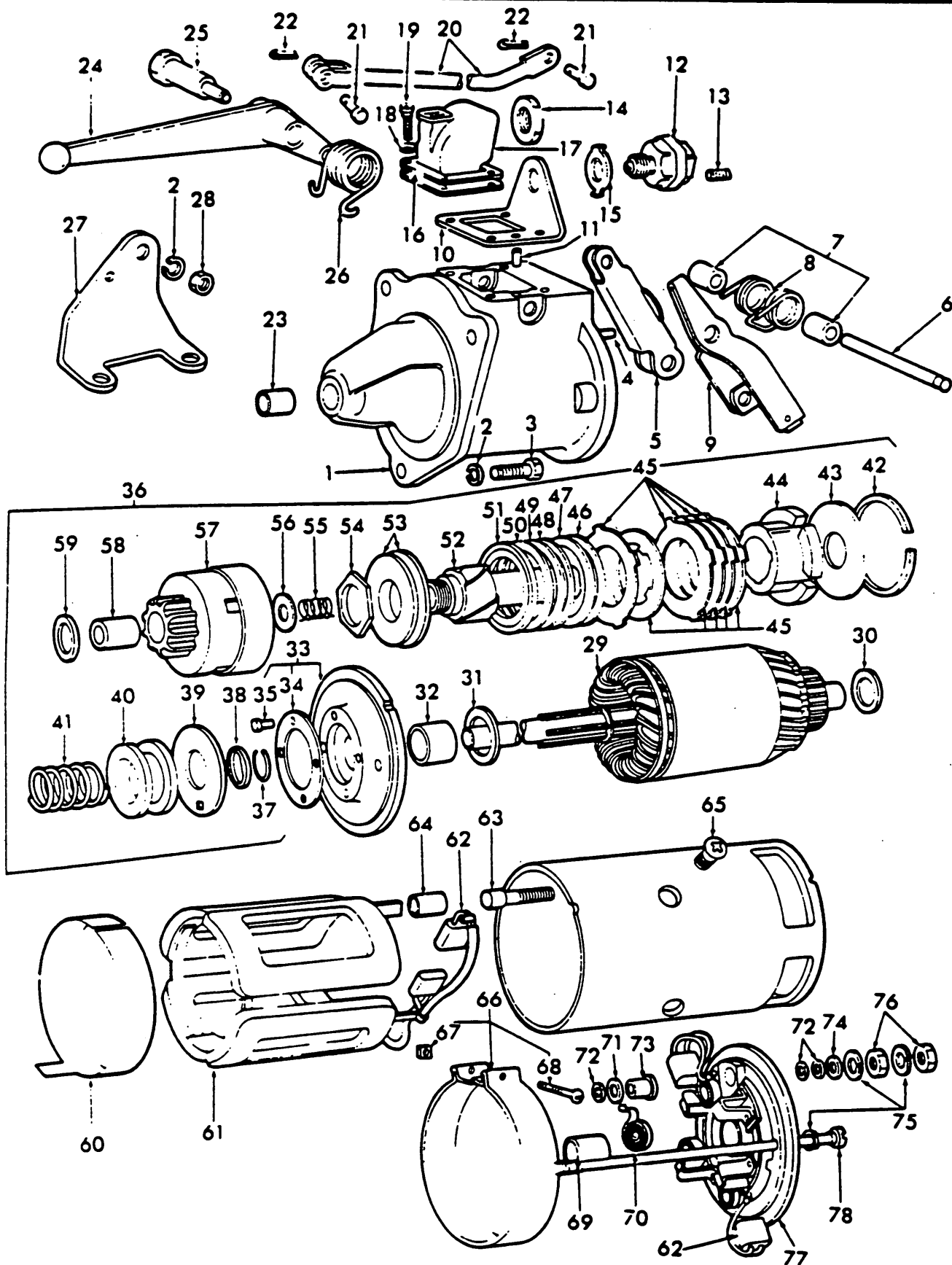
Fig. 83 - Starter Motor - Diesel Engine
