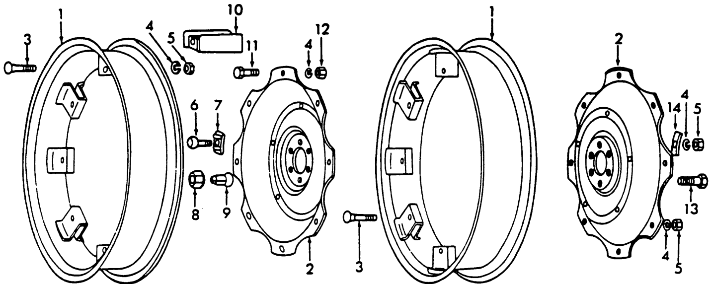
Fig. 3 — Dual Rear Wheels
