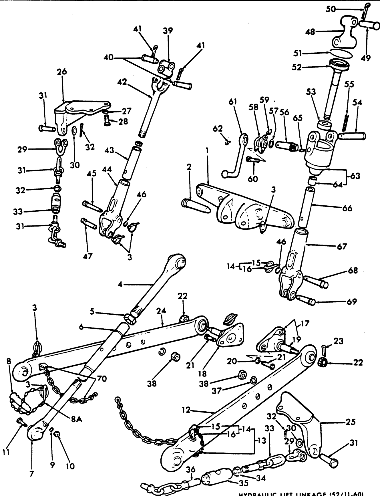
Fig. 32 - Hydraulic Lift Linkage 52/11-60
