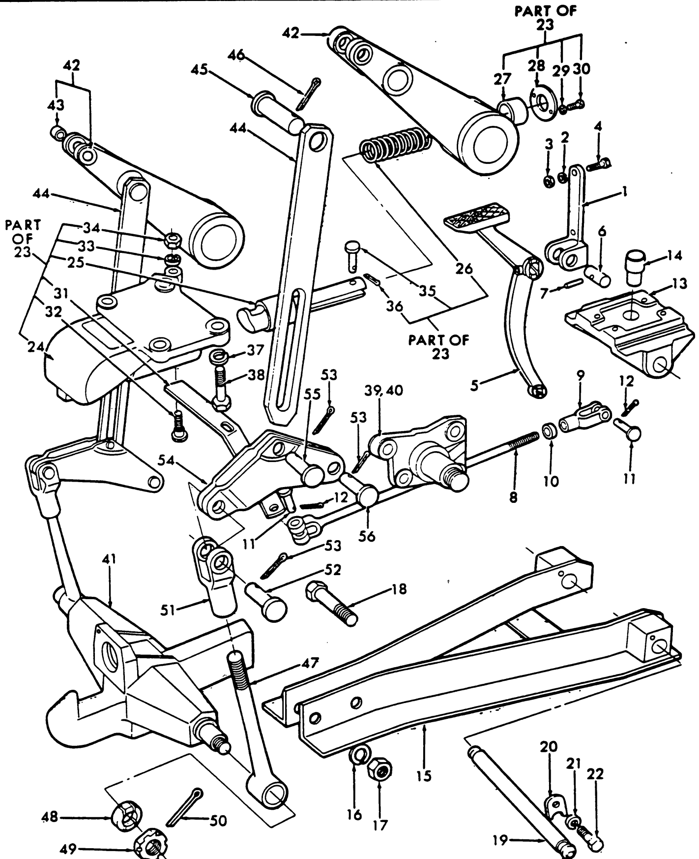
Fig. 34 - Automatic Hitch 11-60/64
