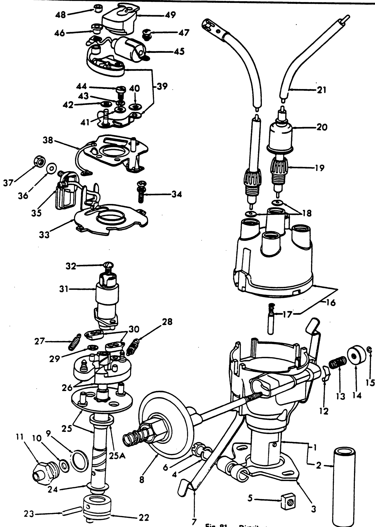
Fig. 81 - Distributor
