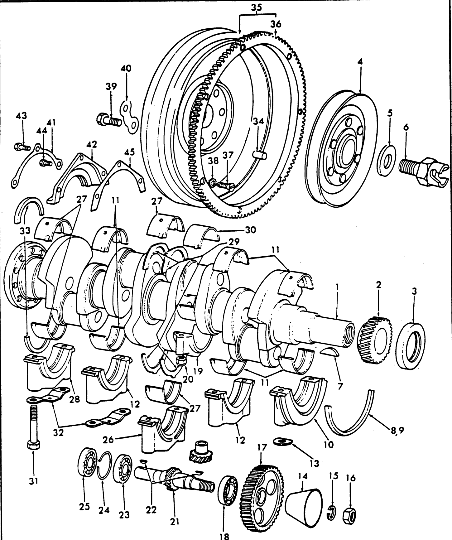
Fig. 42 - Crankshaft, Flywheel & Related Parts
