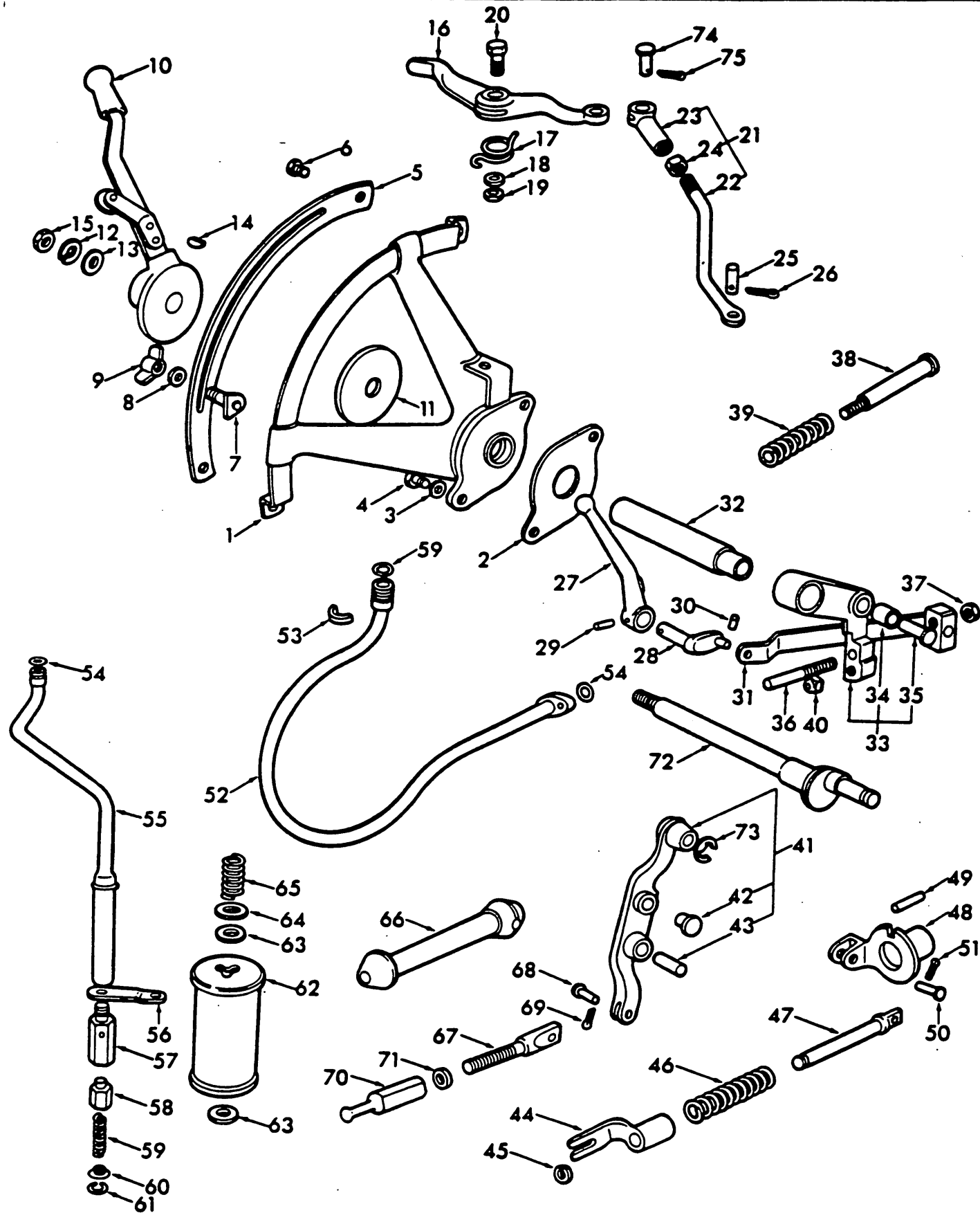
Fig. 29 - Hydraulic Linkage & Related Parts
