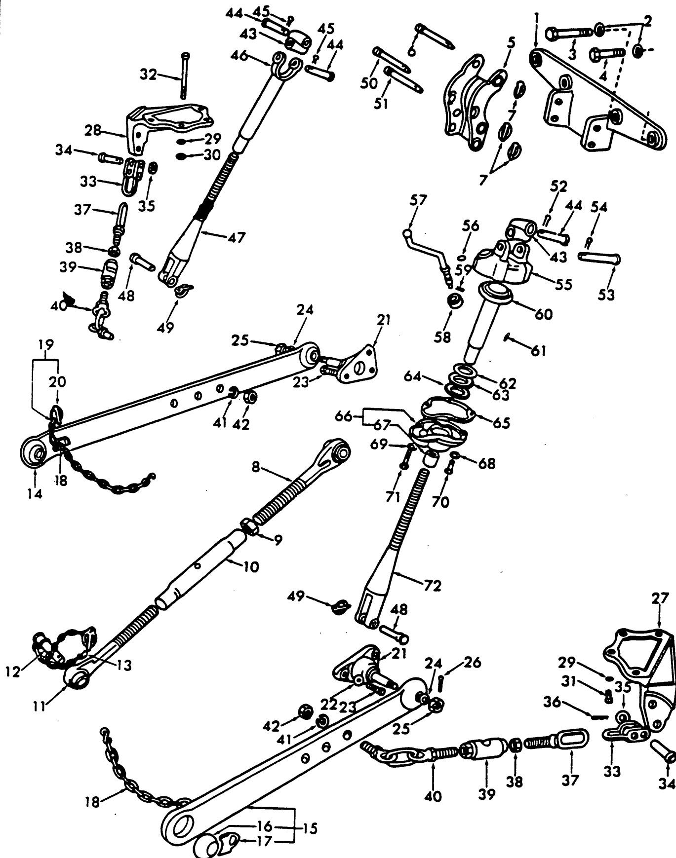
Fig. 31 - Hydraulic Lift Linkage 11-60/64
