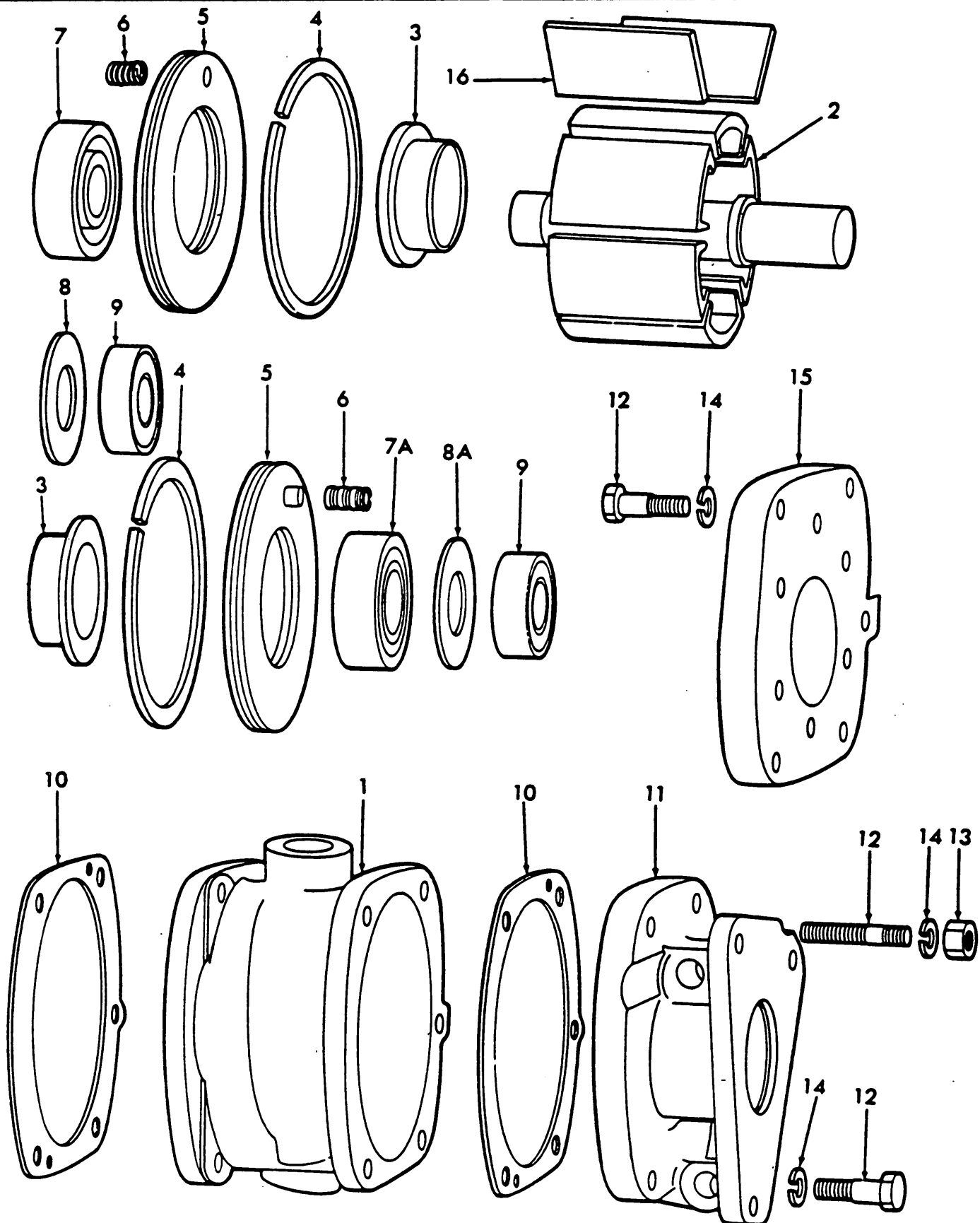
Fig. 9 - Vacuum Braking Exhauster - FTO-E
