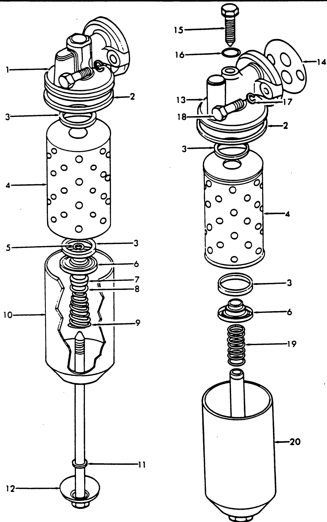
Fig. 46 - Engine Oil Filters
