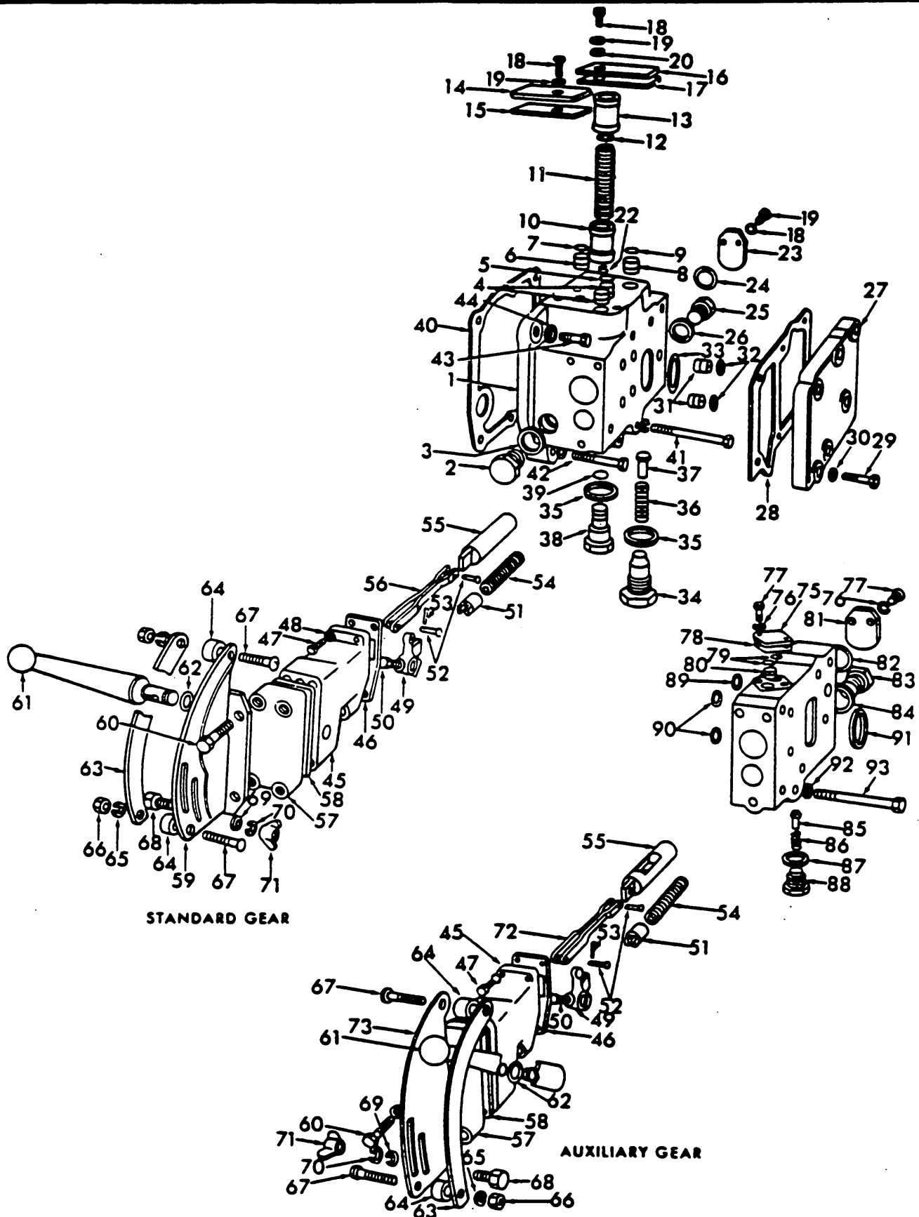
Fig. 39 - Valve Gear Assy. H.P.L.
