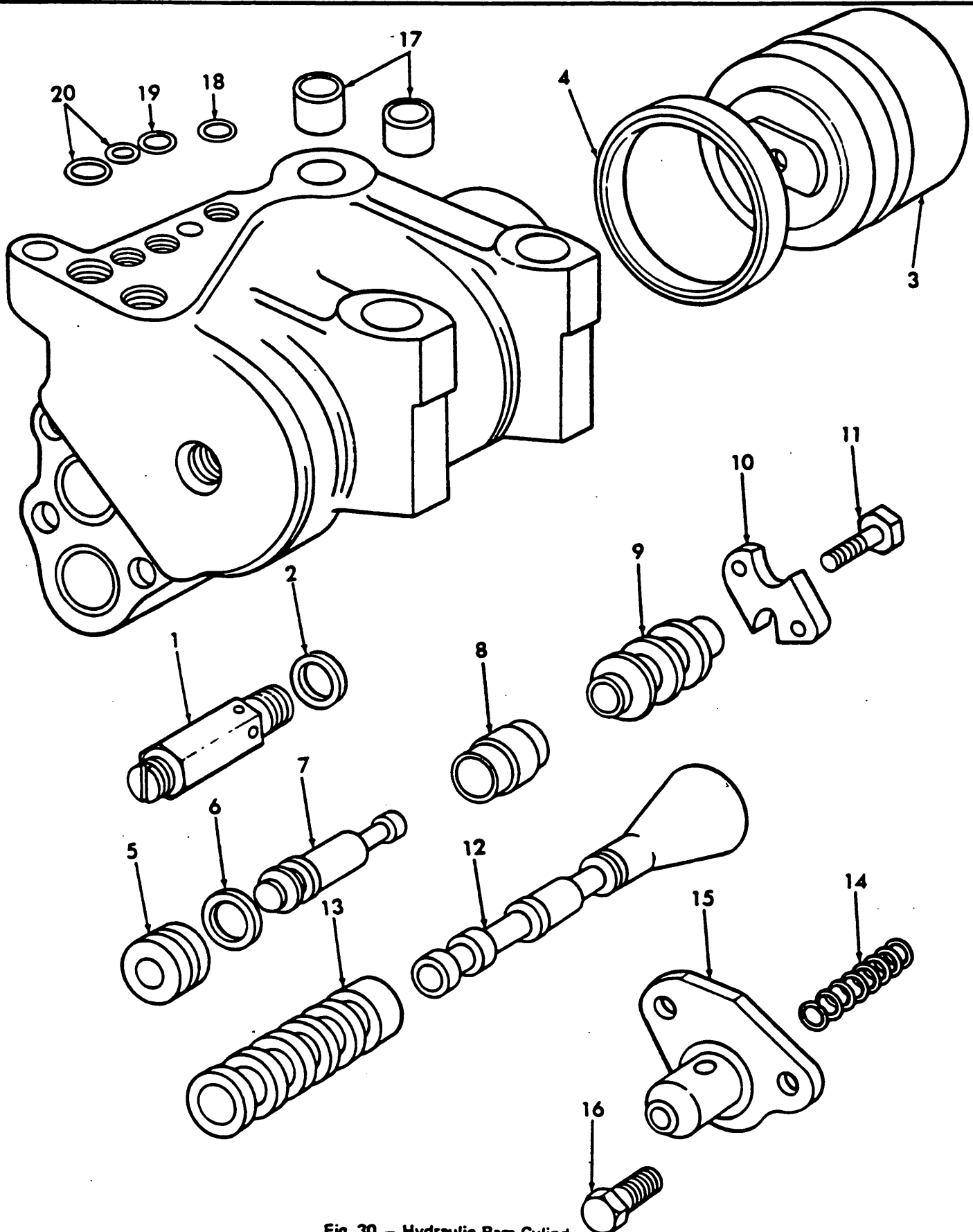
Fig. 30 - Hydraulic Ram Cylinder
