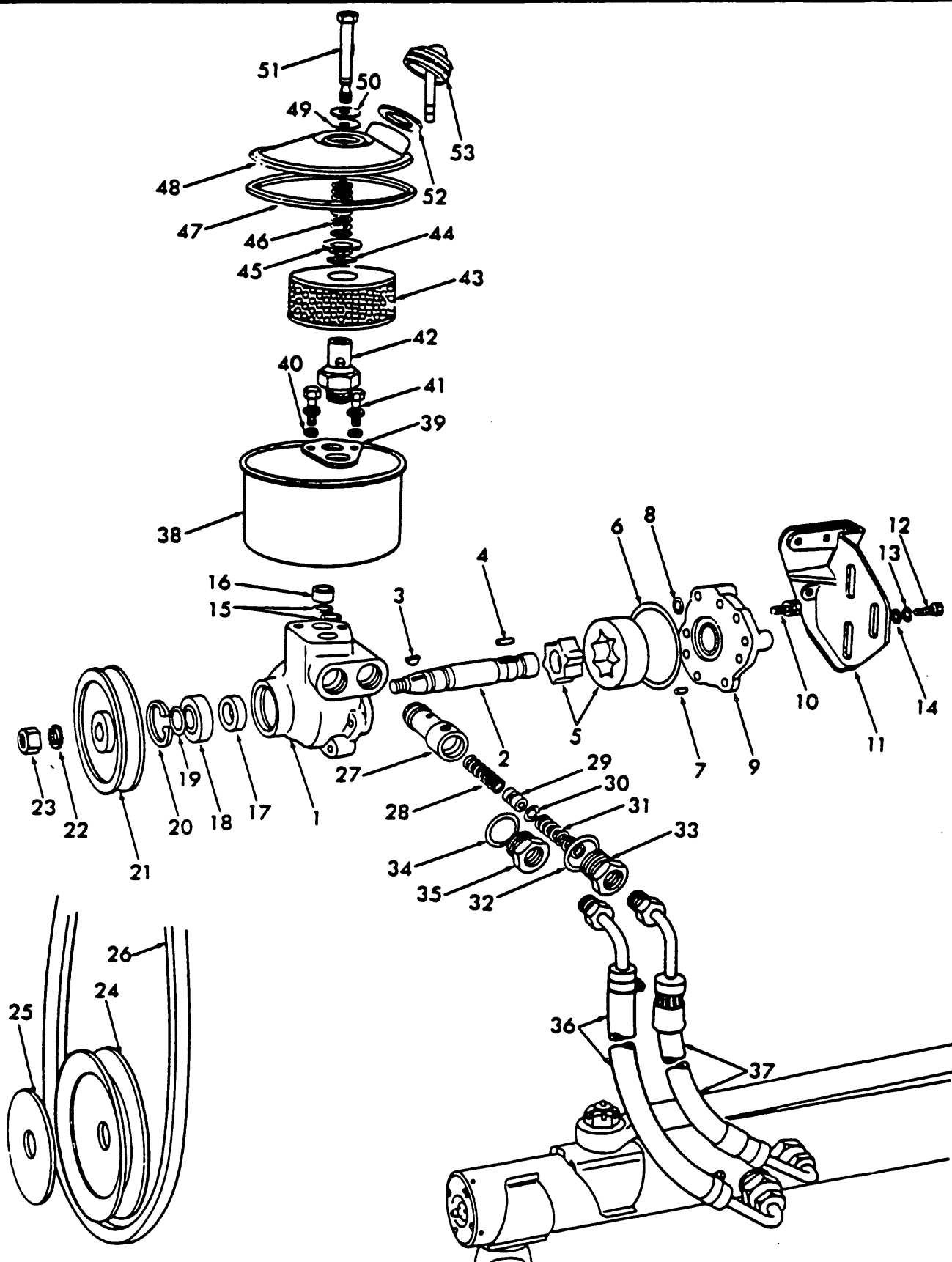
Fig. 16 - Power Steering Pump & Reservoir
