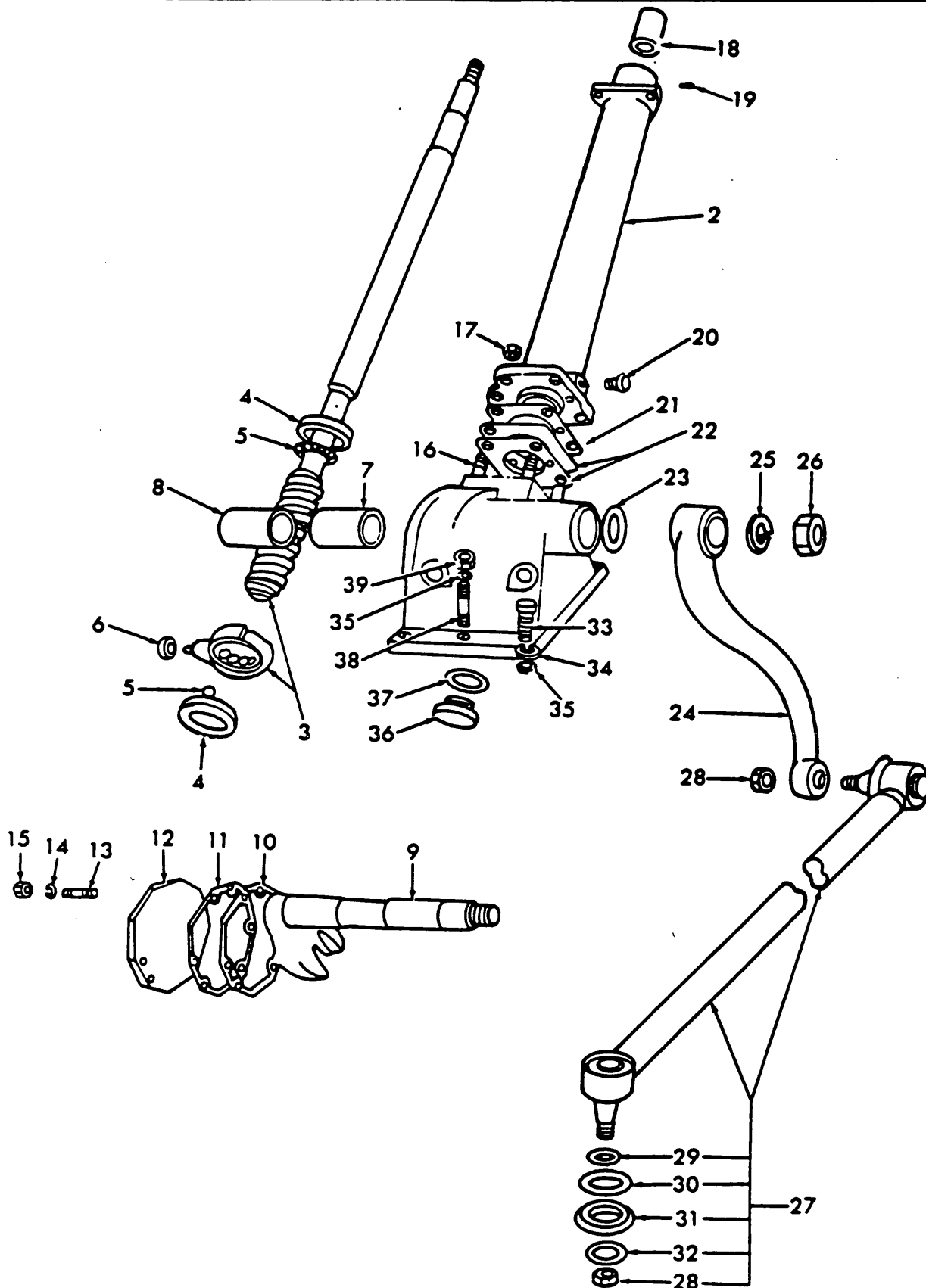
Fig. 14 - Steering Gear
