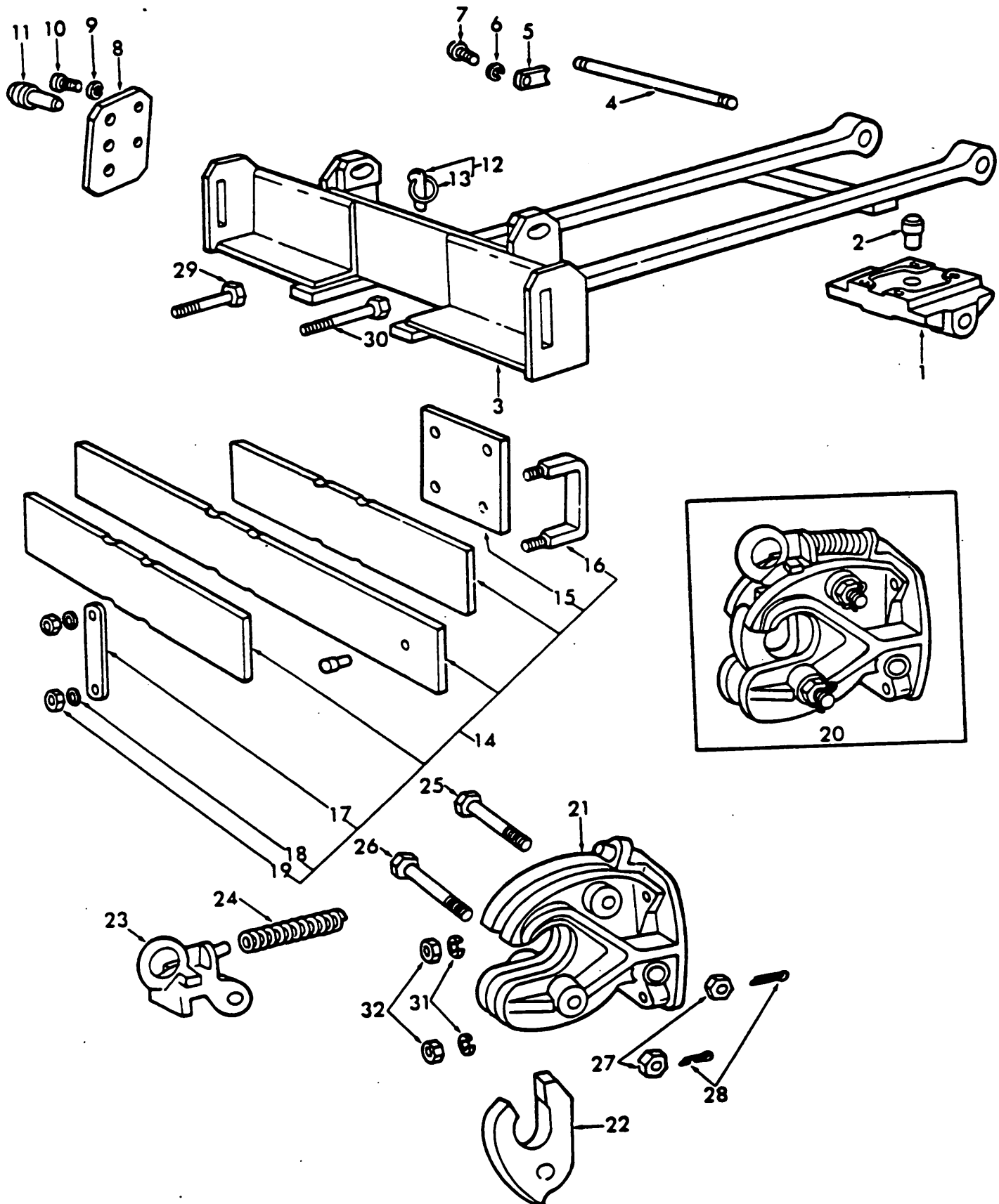
Fig. 90 - Rear Tow Attachment
