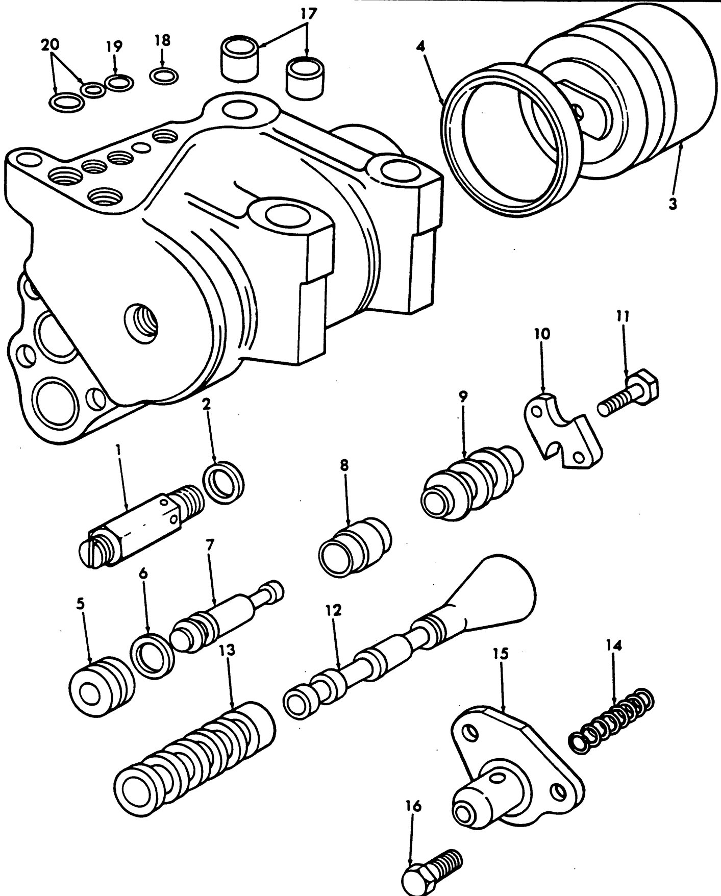
Fig. 30 - Hydraulic Ram Cylinder
