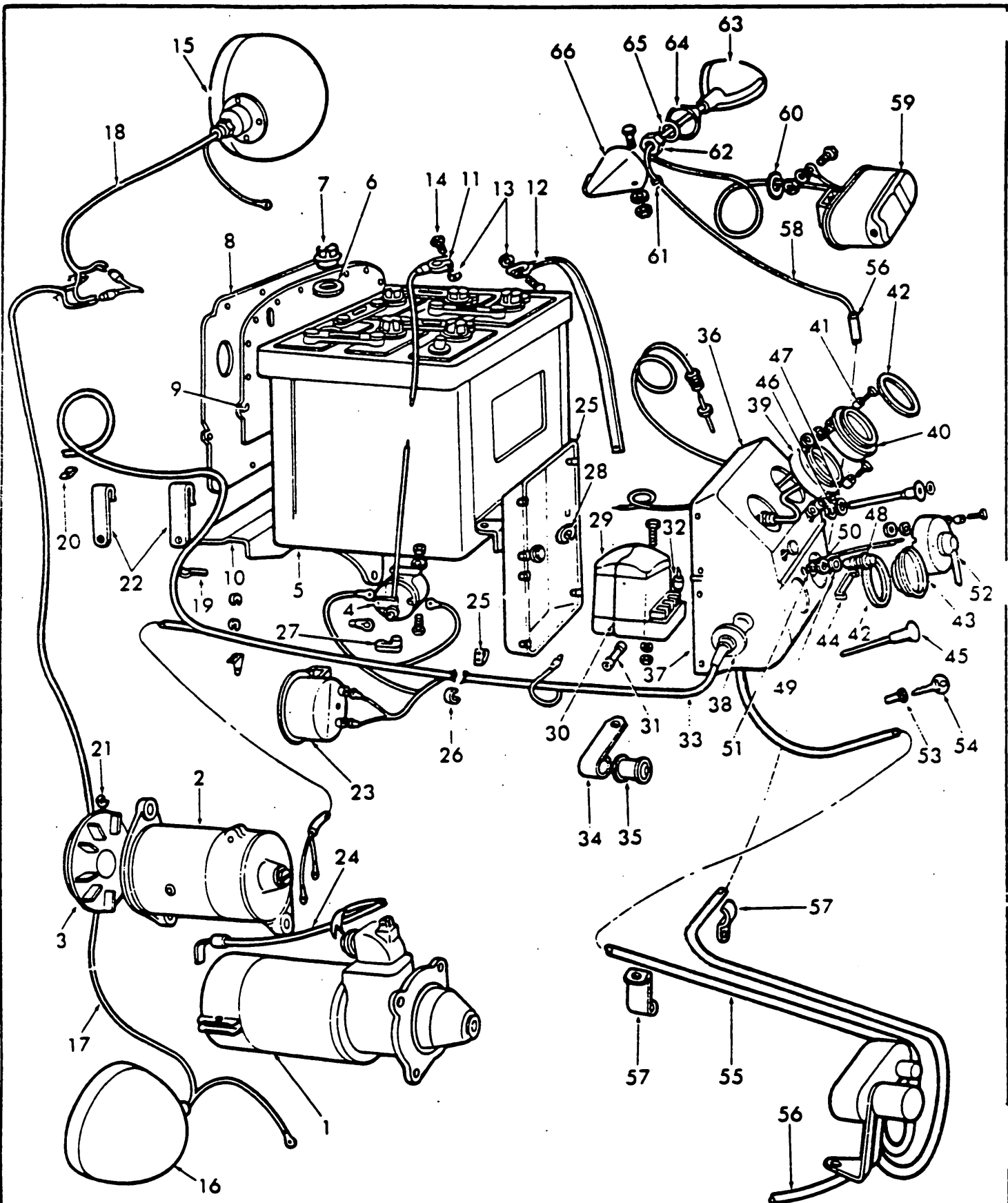
Fig. 76 - Electrical System 52/8-58
