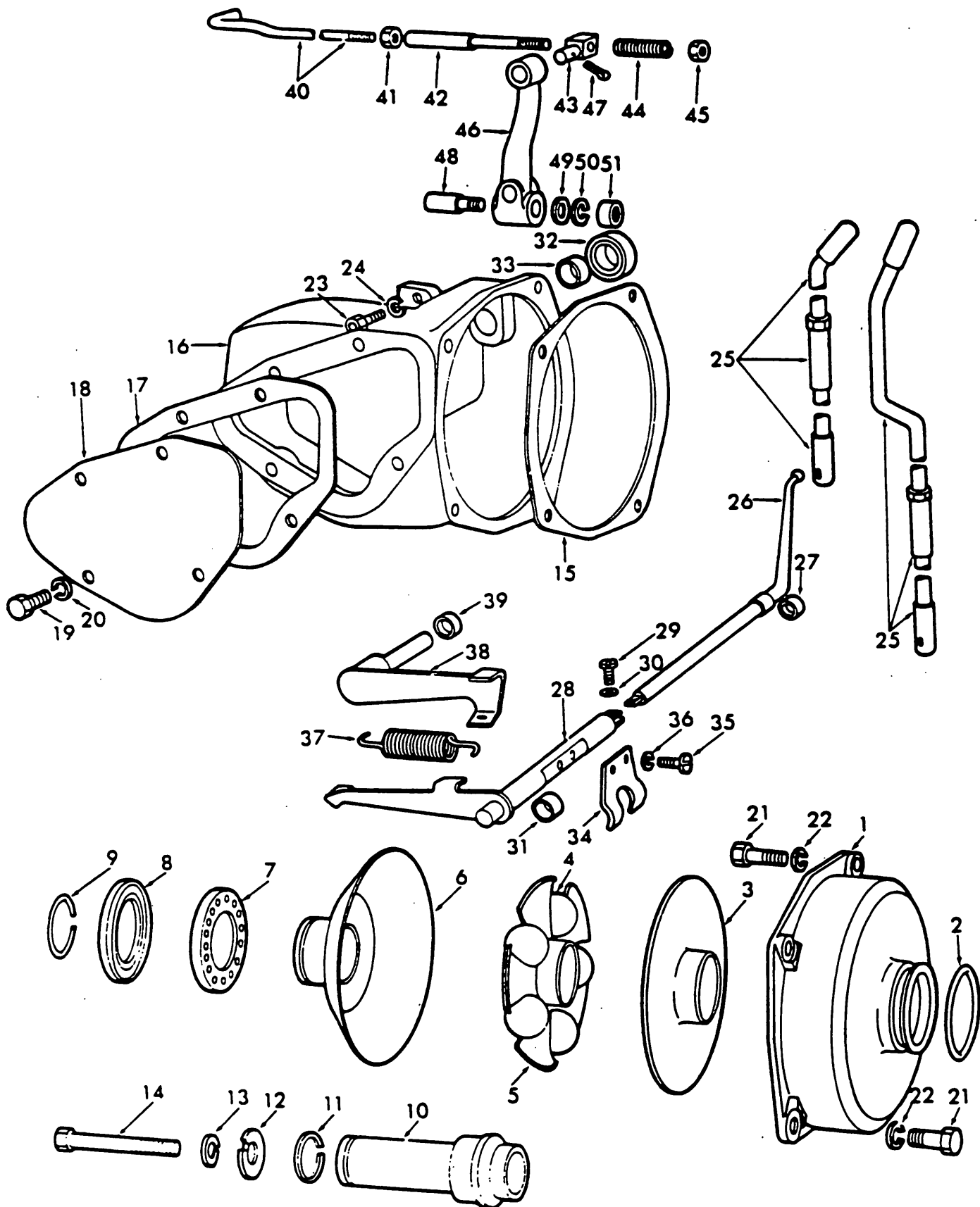
Fig. 49 - Governor & Control Linkage
