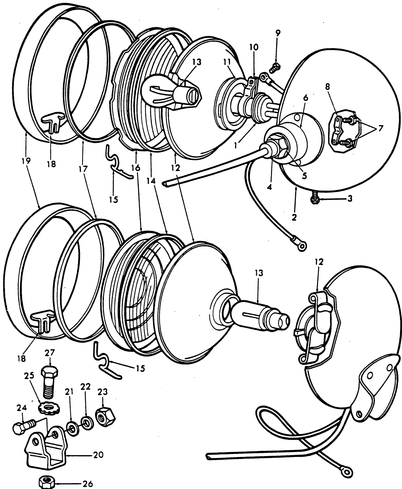
Fig. 78 - Headlamps
