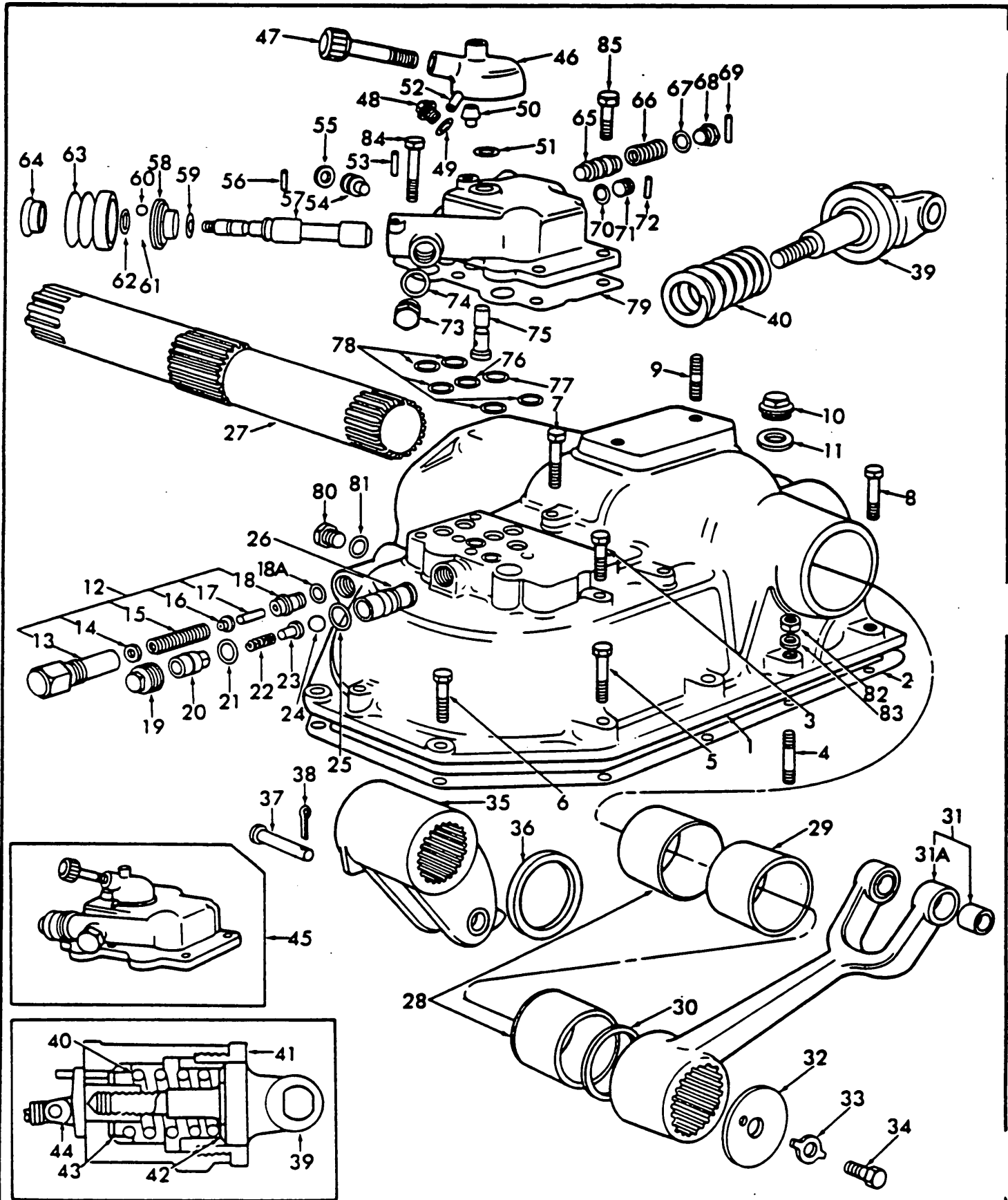
Fig. 28 - Hydraulic Lift Cover, Shaft & Related Parts 11-60/64
