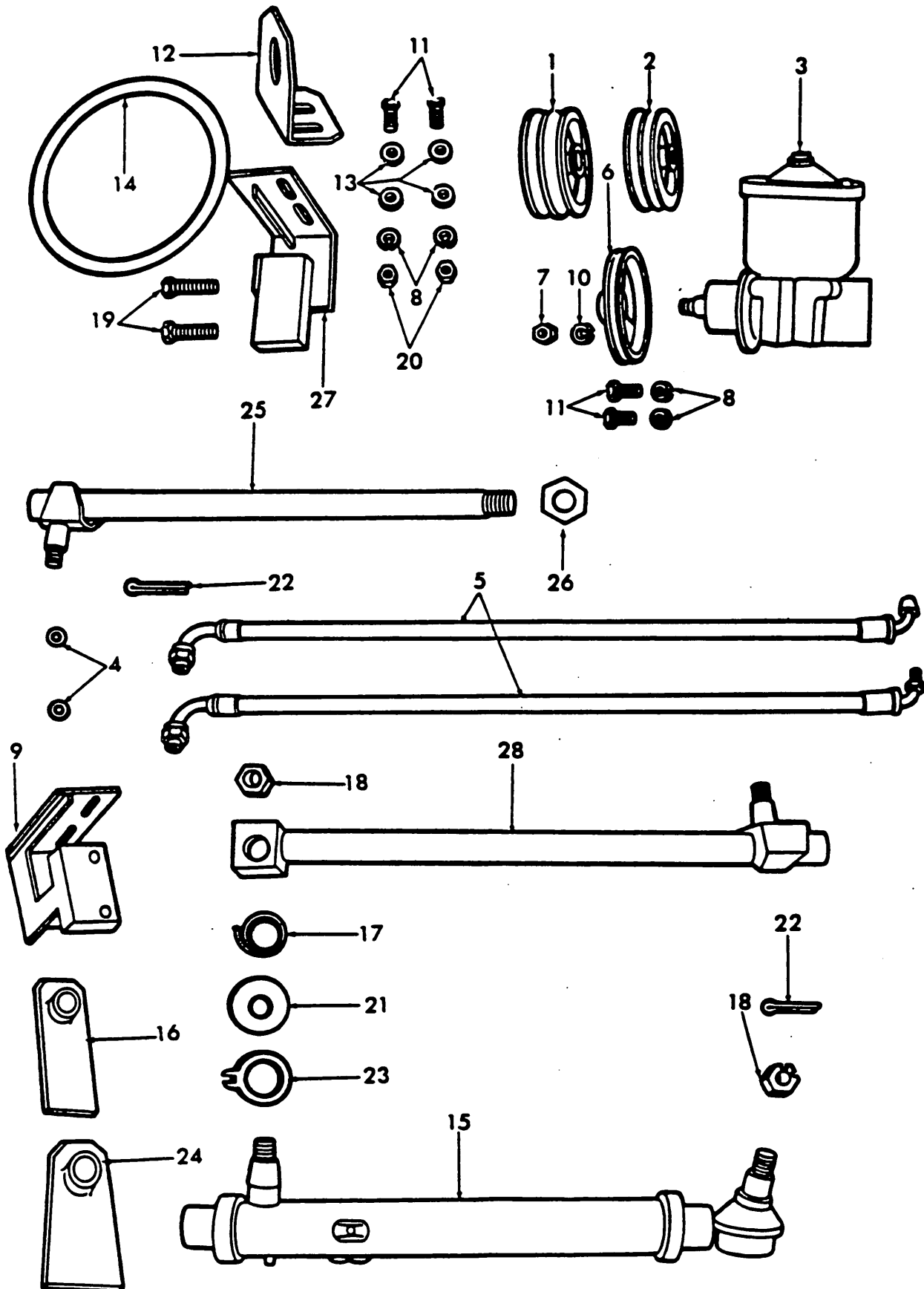
Fig. 19 — Power Steering U.S. 15A-1000
