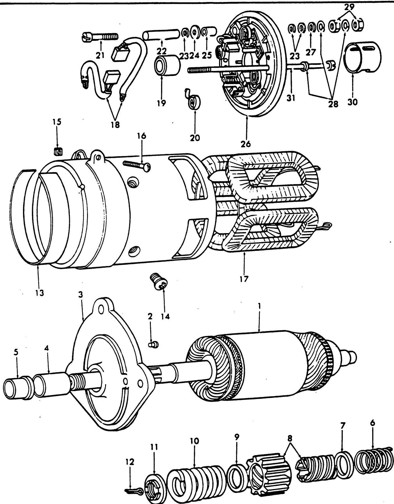
Fig. 84 - Starter Motor - Petrol Engine
