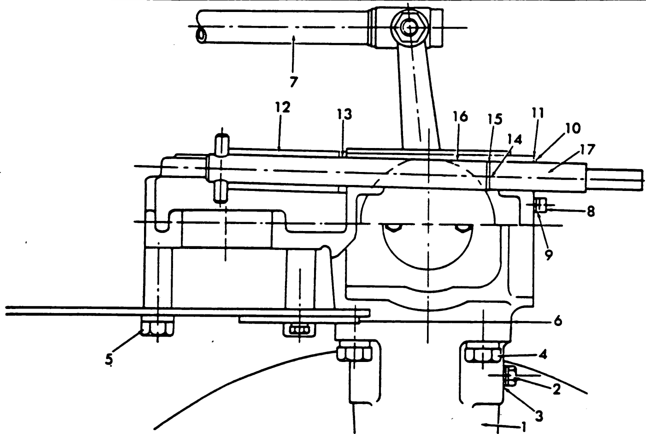
Fig. 13 - Rowcrop Eng. Turning Handle & Related Parts 72 & 96
