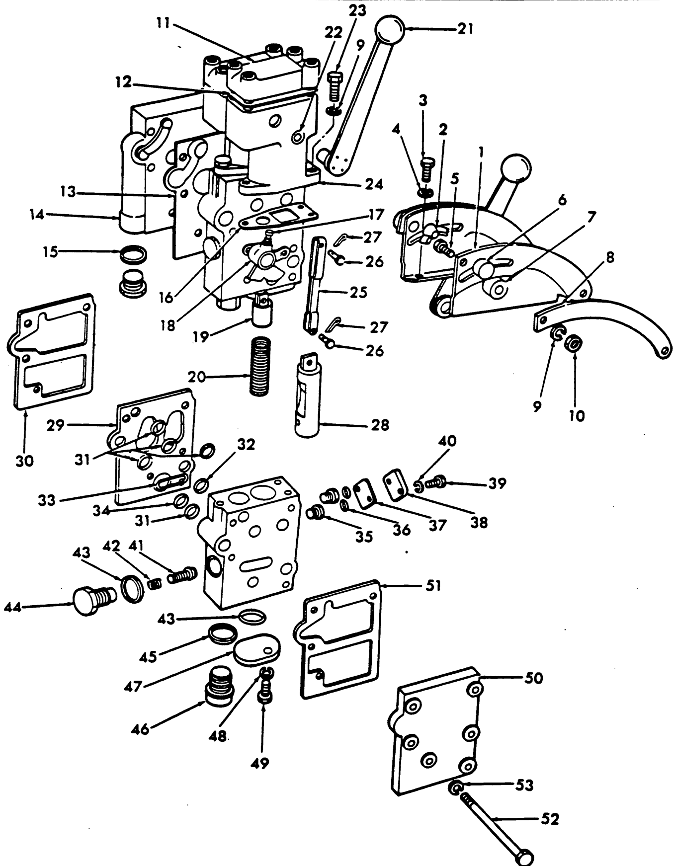
Fig. 40 - Dual Auxiliary Valve
