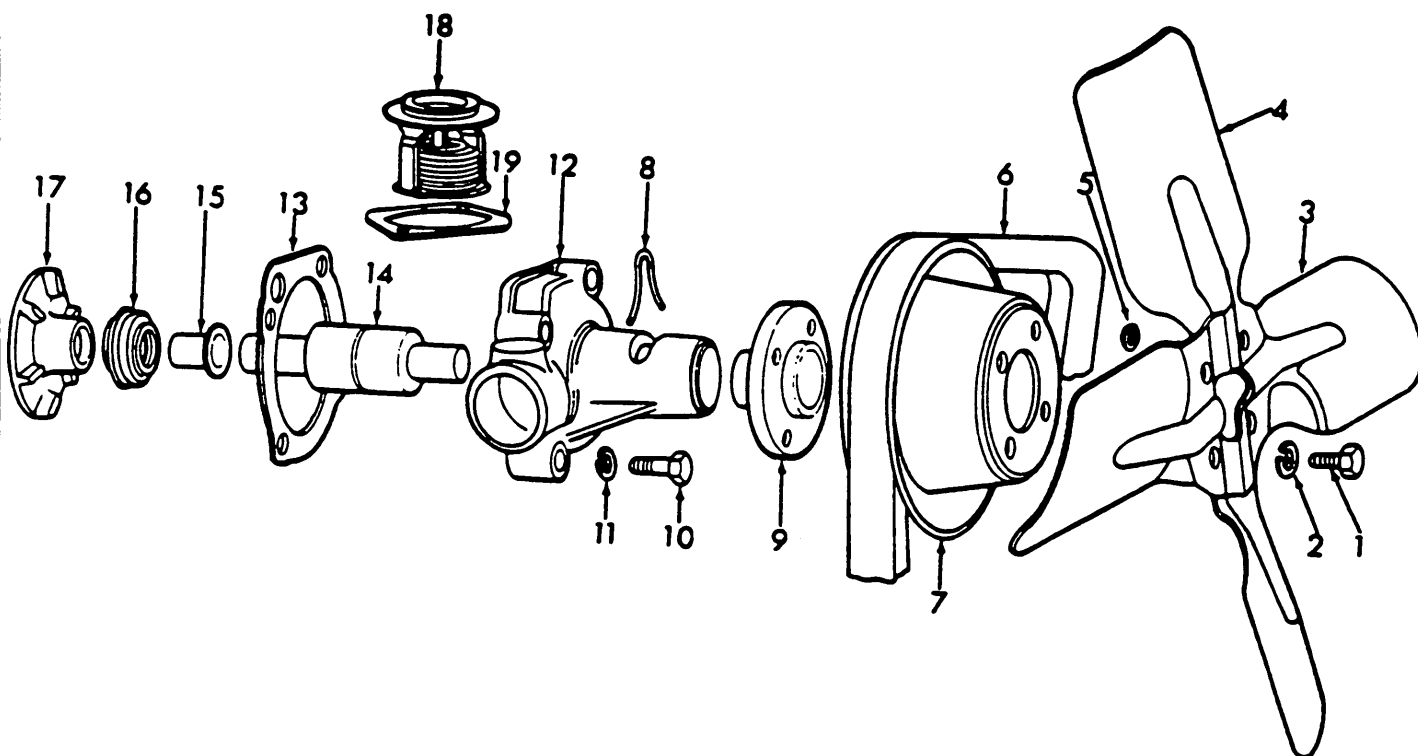
Fig. 57 - Water Pump & Thermostat
