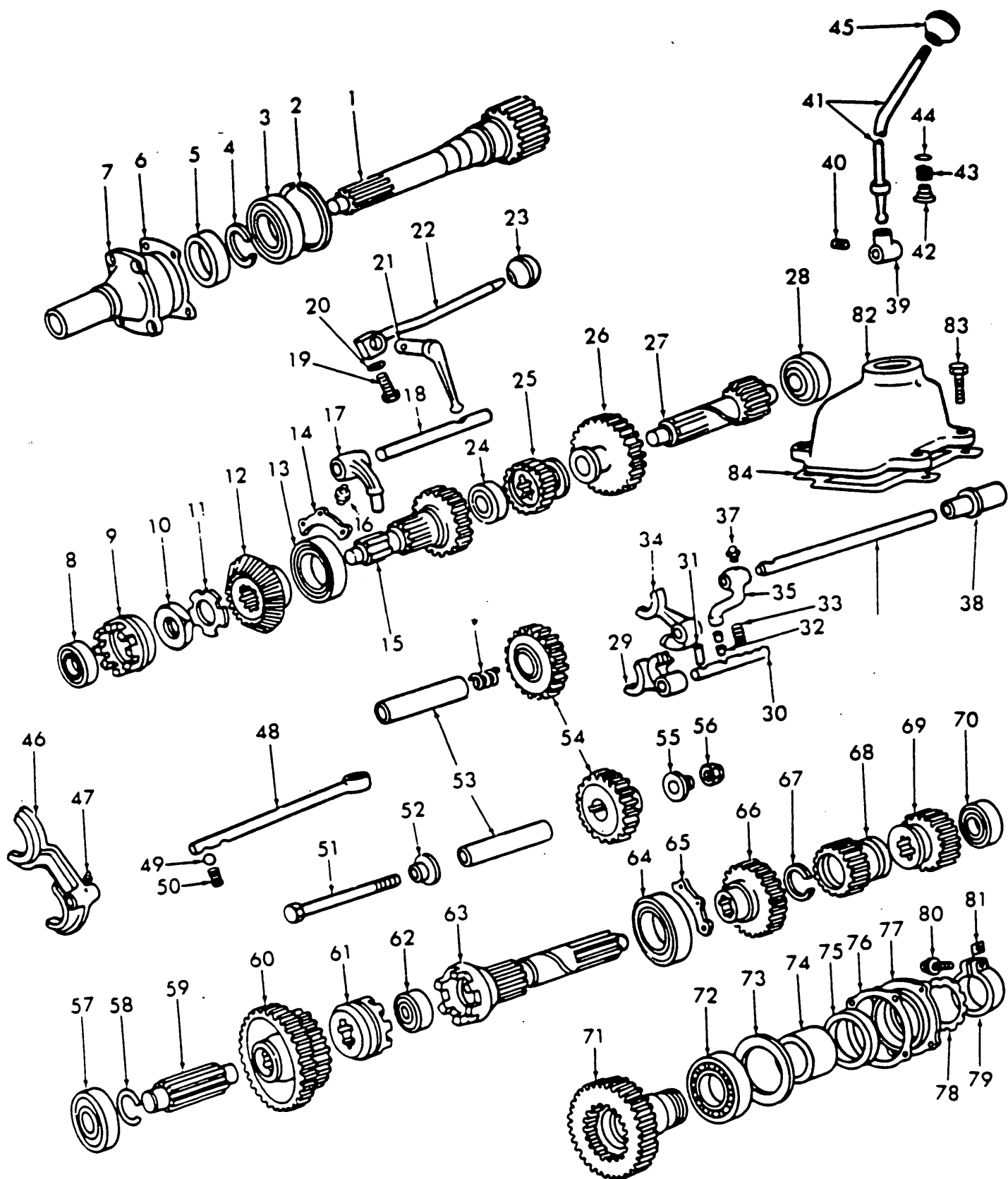
Fig. 51 - Front Transmission Internal
