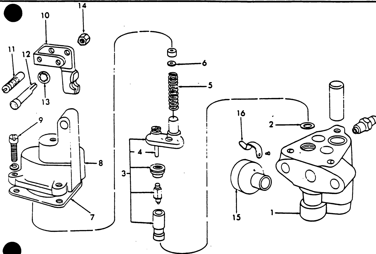
Fig. 68 — Starter Carburetor - Used in 1952 Only - FTO-E
