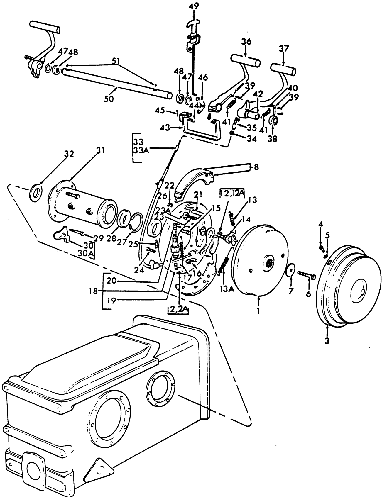
Fig. 6 - Steering Brakes 52/11-60
