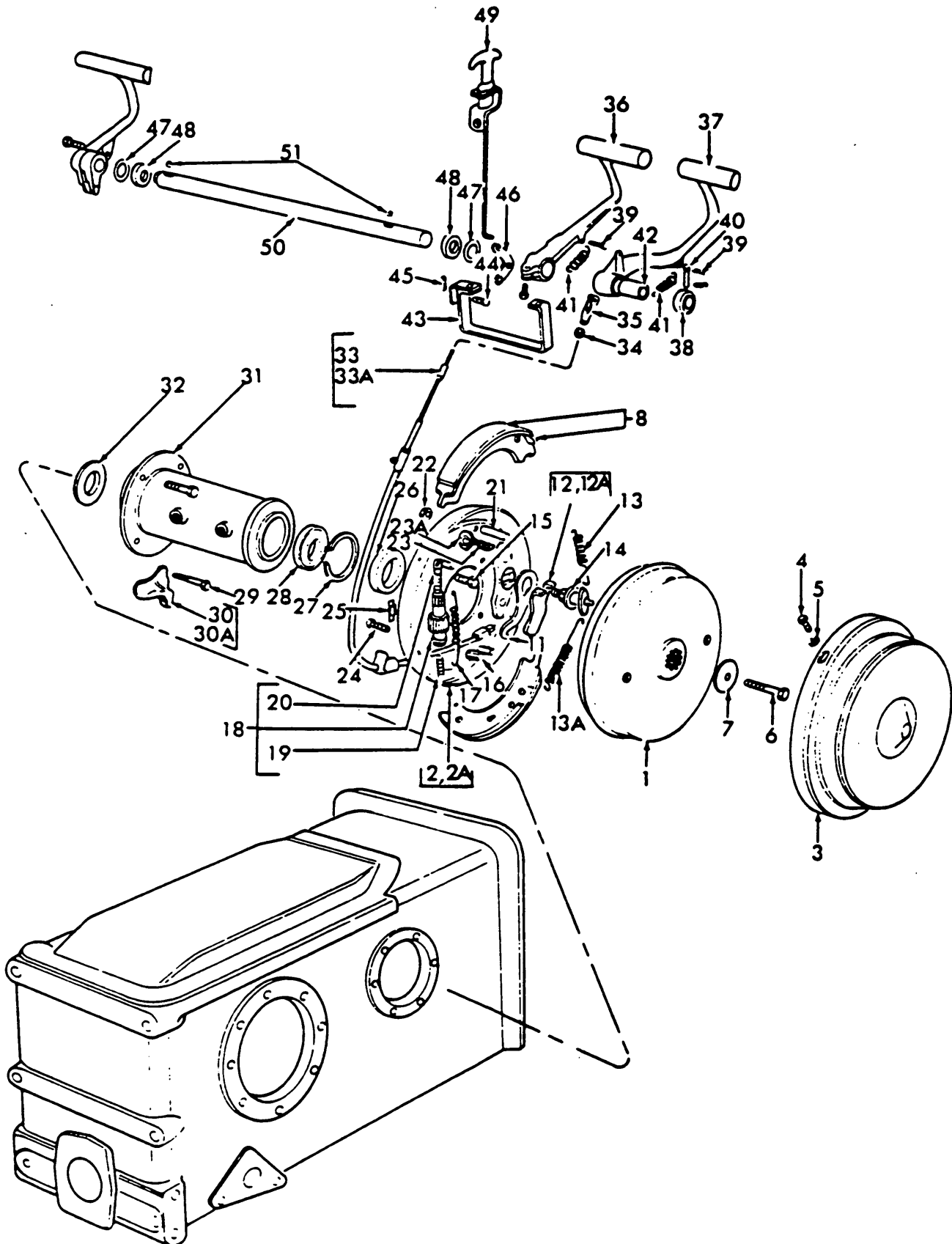
Fig. 6 - Steering Brakes 52/11-60
