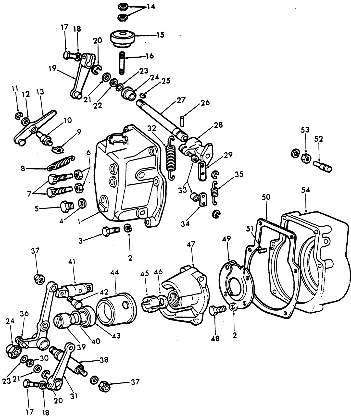
Fig. 71 - Mechanical Governor - Fuel Inj. Pump
