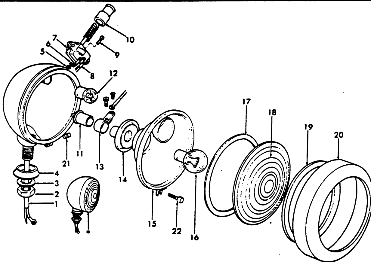
Fig. 80 - Ploughing Lamp
