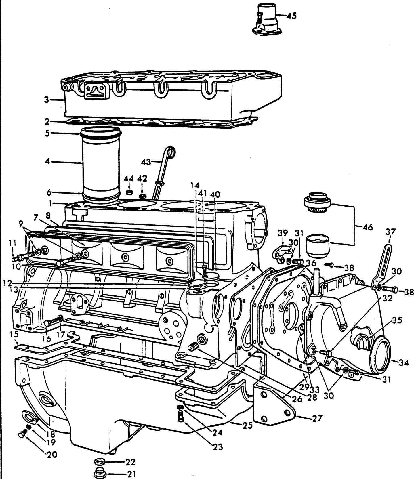
Fig. 41 - Cylinder Block, Head & Related Parts
