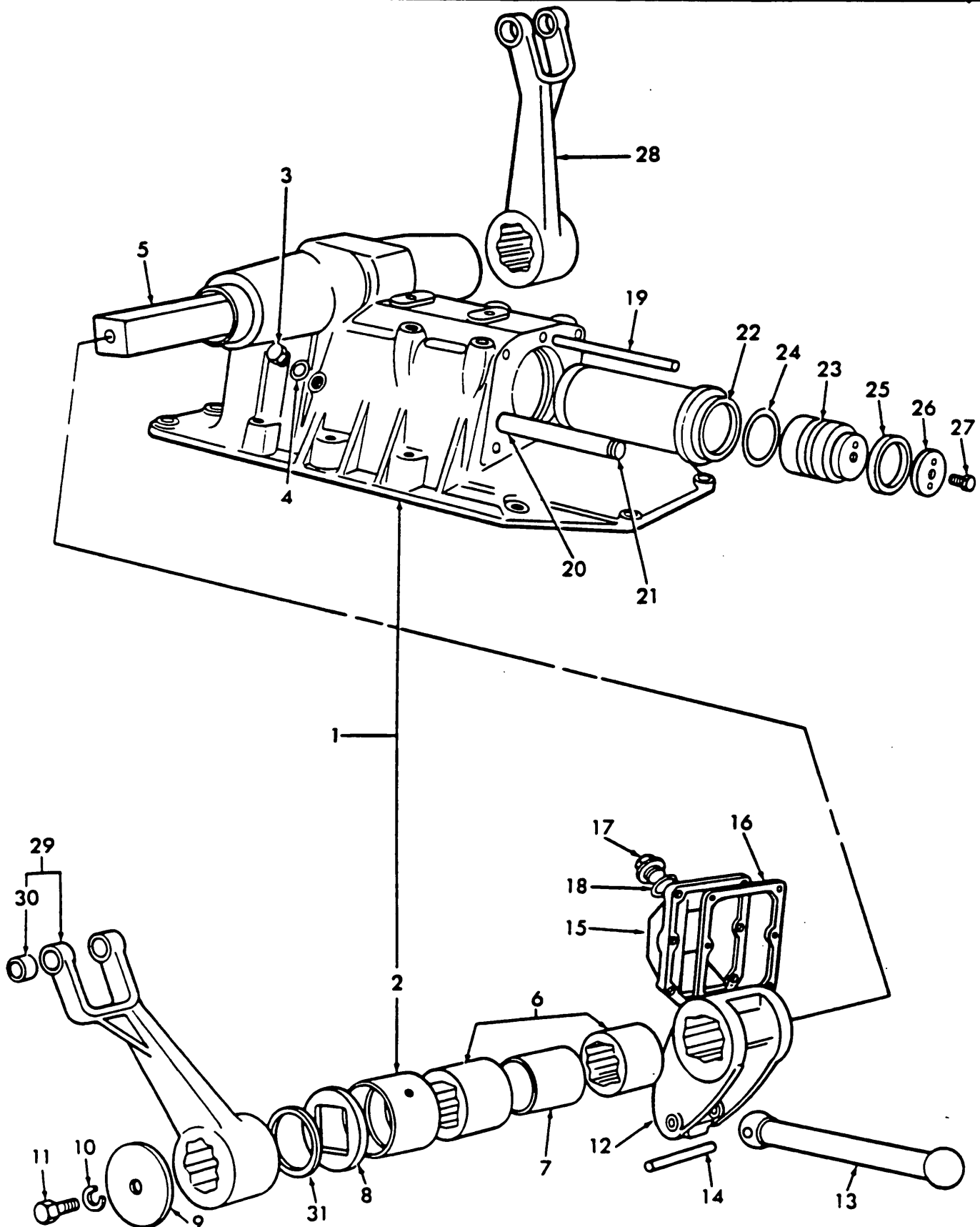
Fig. 27 - Hydraulic Lift Cover, Shaft & Related Parts 52/11-60
