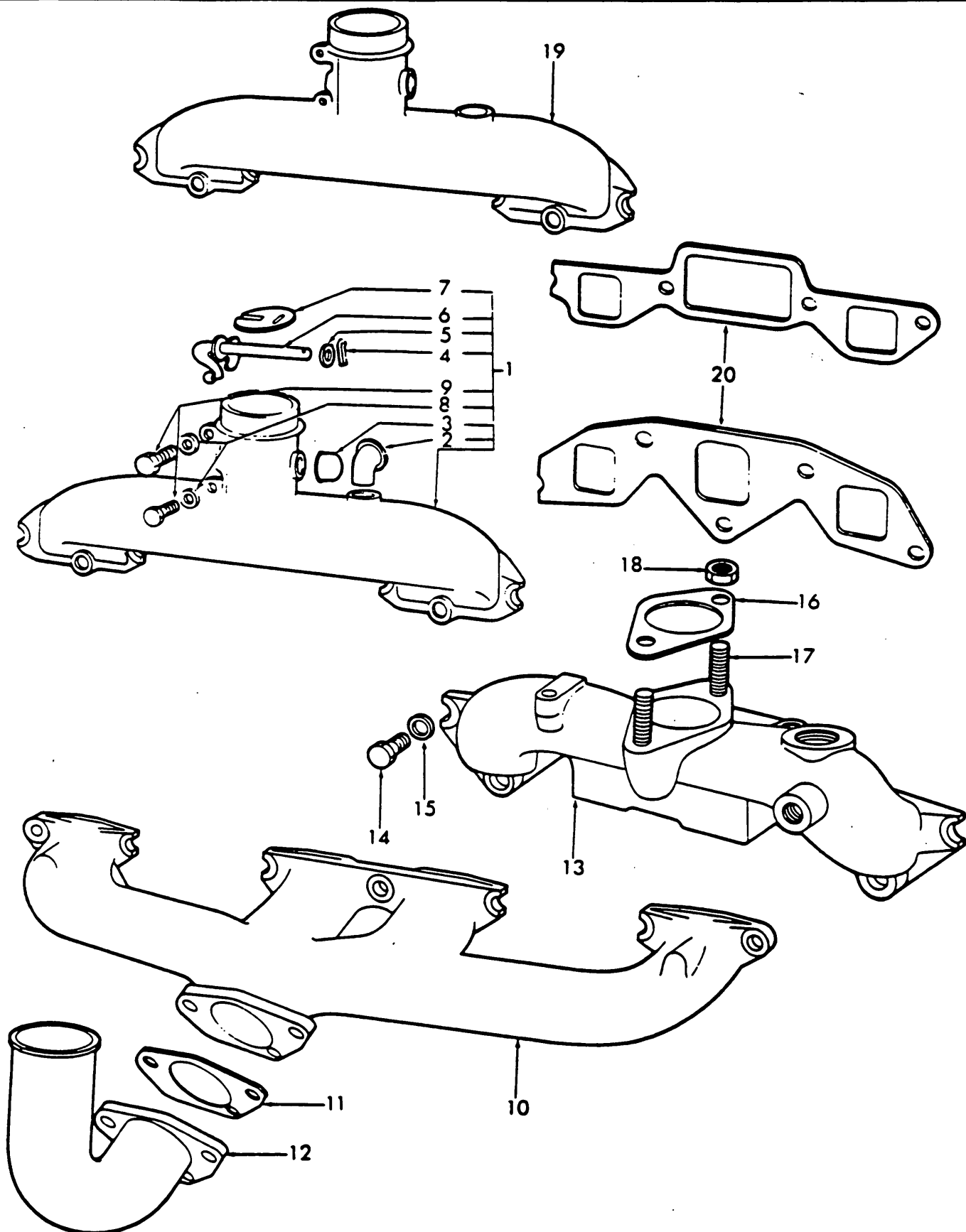
Fig. 47 - Inlet & Exhaust Manifolds
