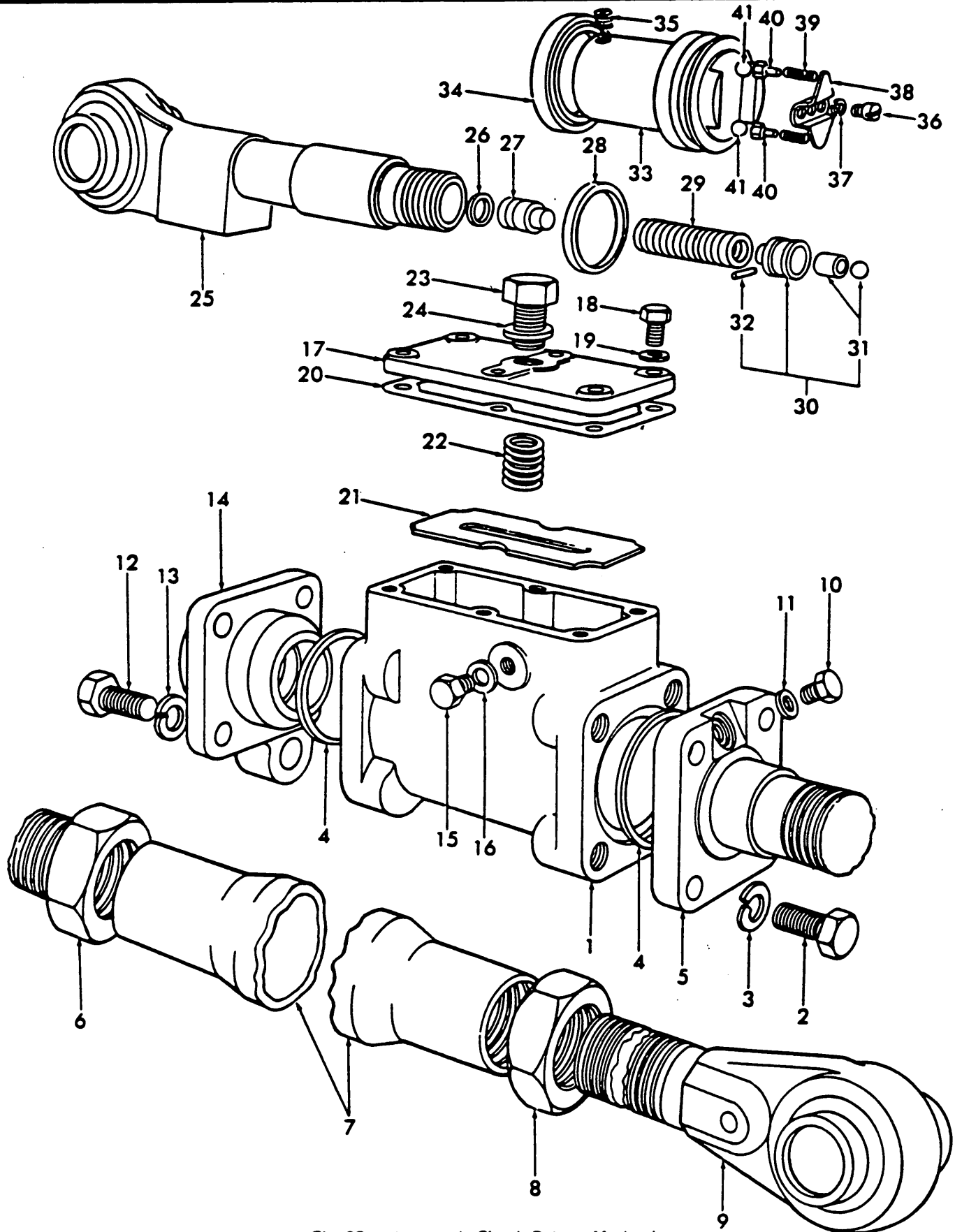
Fig. 35 - Automatic Clutch Release Mechanism
