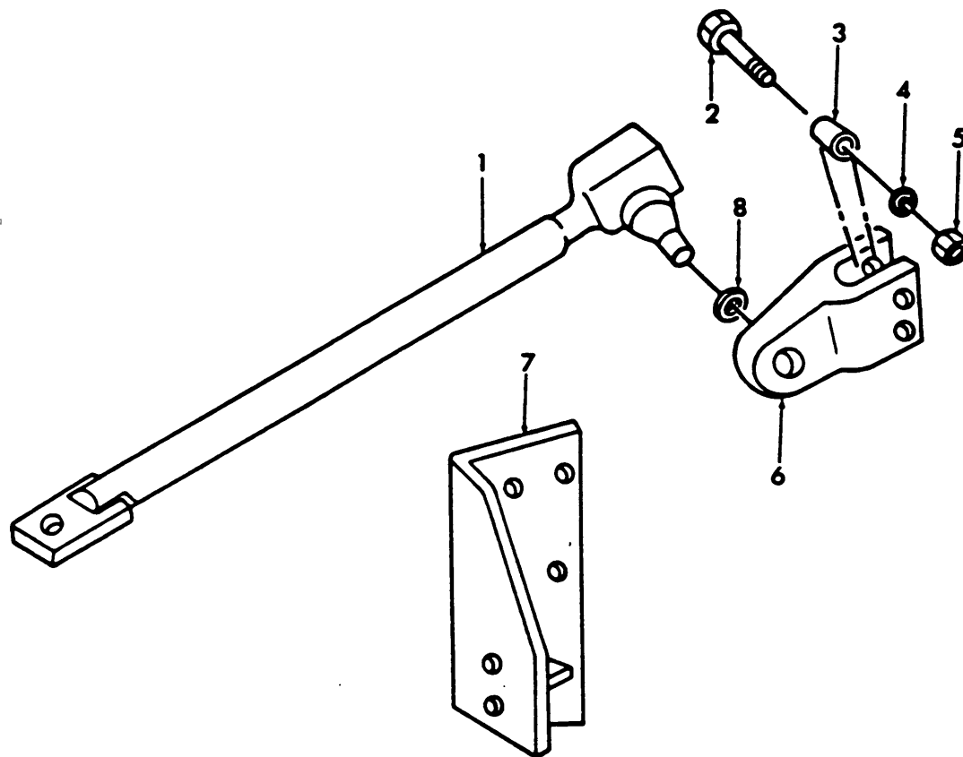
Fig. 23 — Steering Kit Used w/Ford Power Steering 1257
