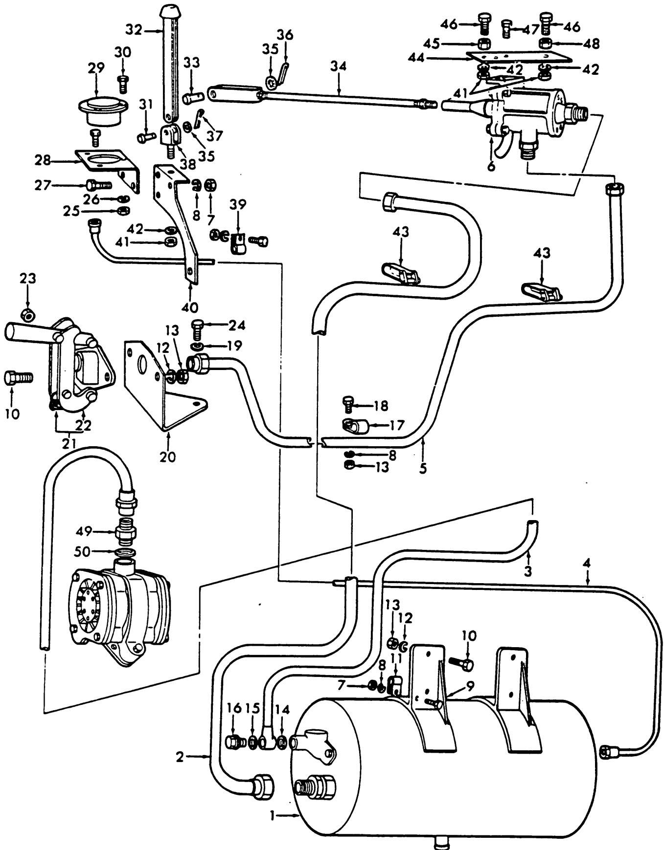
Fig. 8 - Vacuum Braking System
