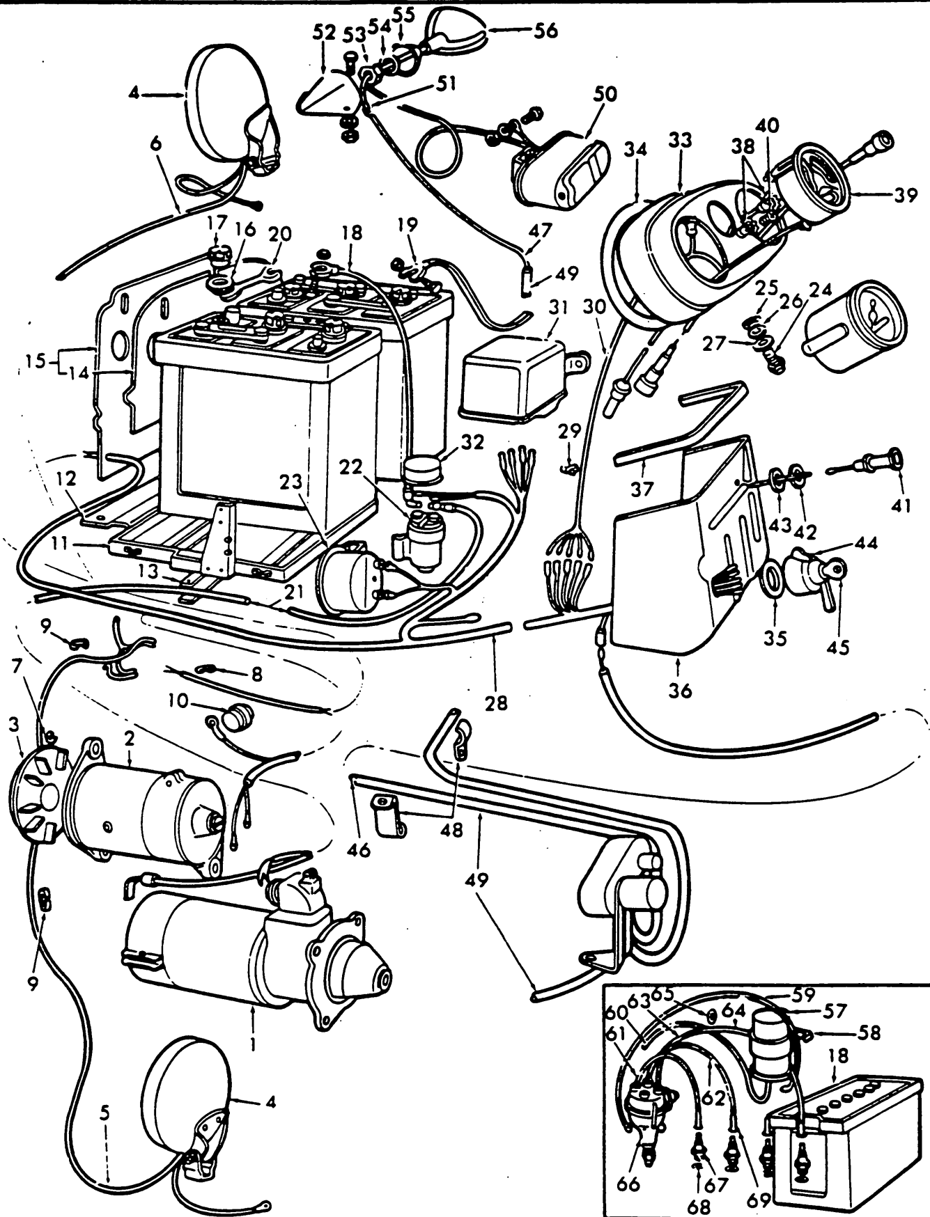
Fig. 77 - Electrical System
