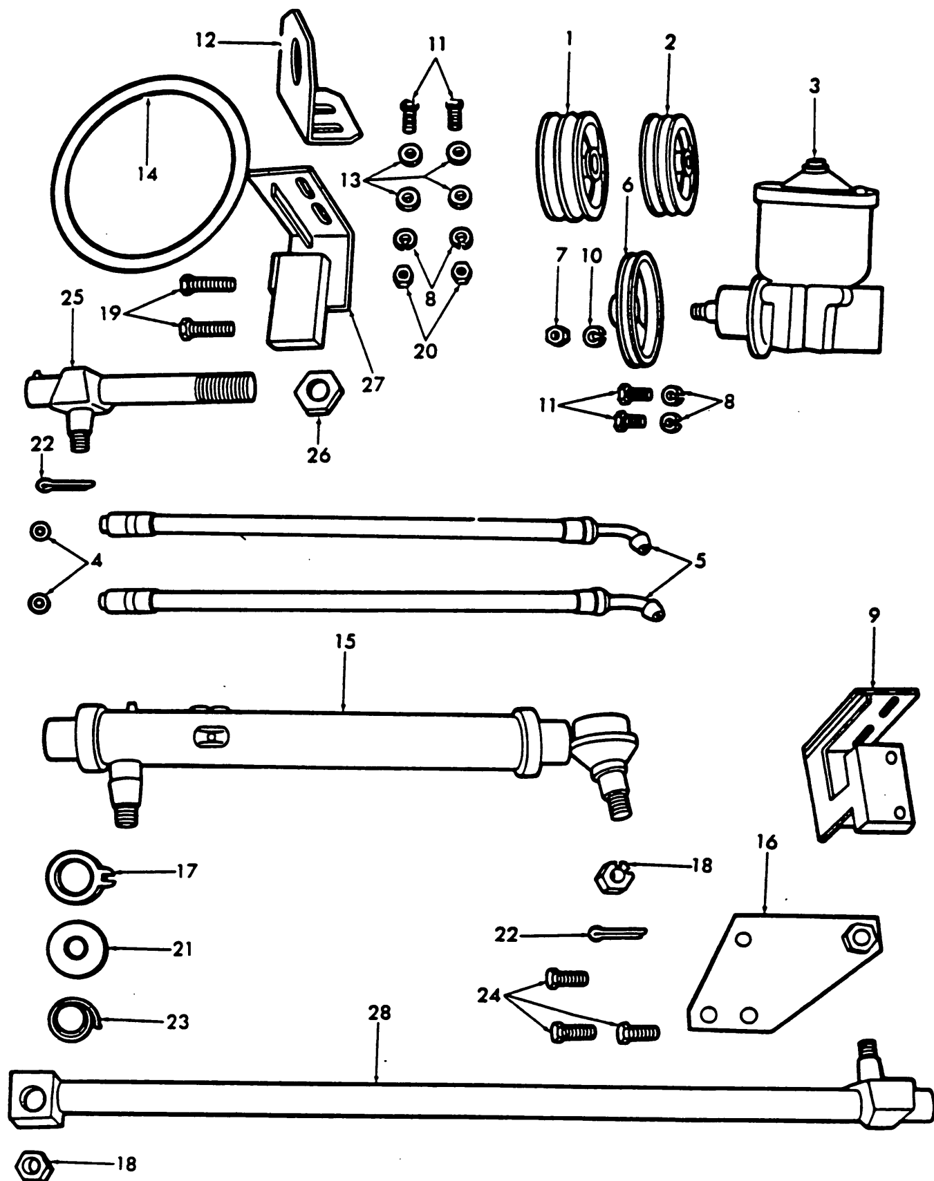
Fig. 20 - Power Steering U.S. 15A-1100
