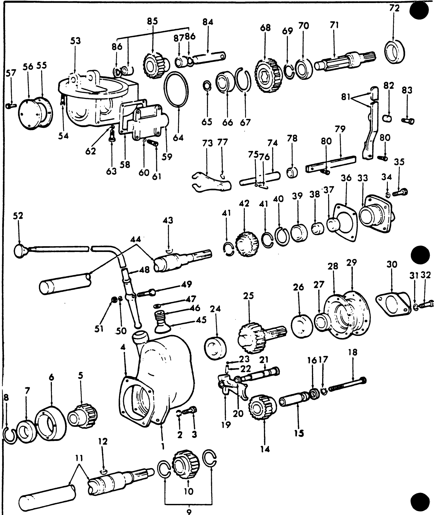
Fig. 54 - Power Take-Off - Standard & Raised
