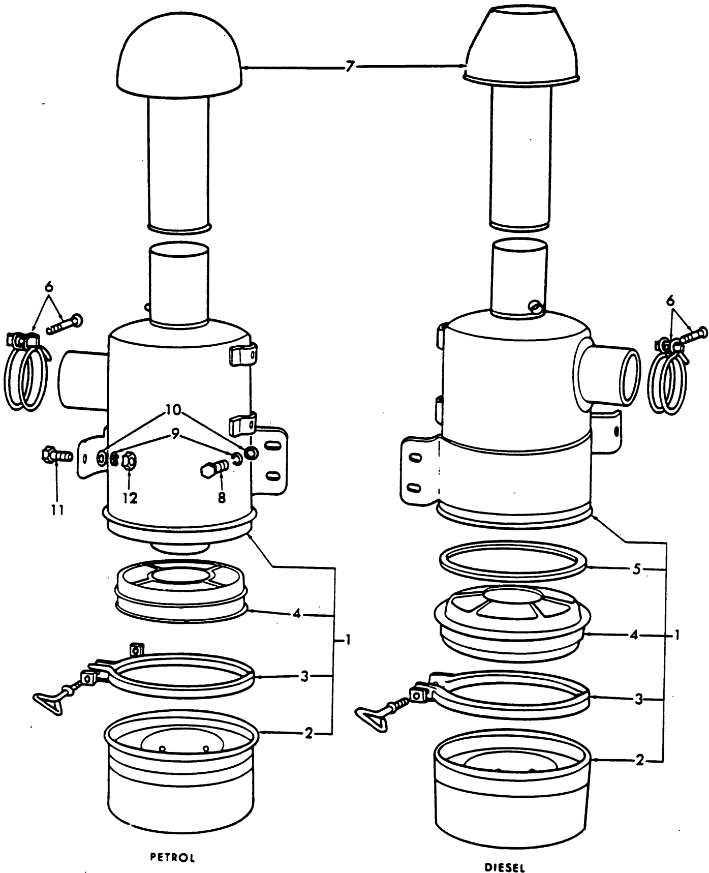
Fig. 64 - Air Cleaner
