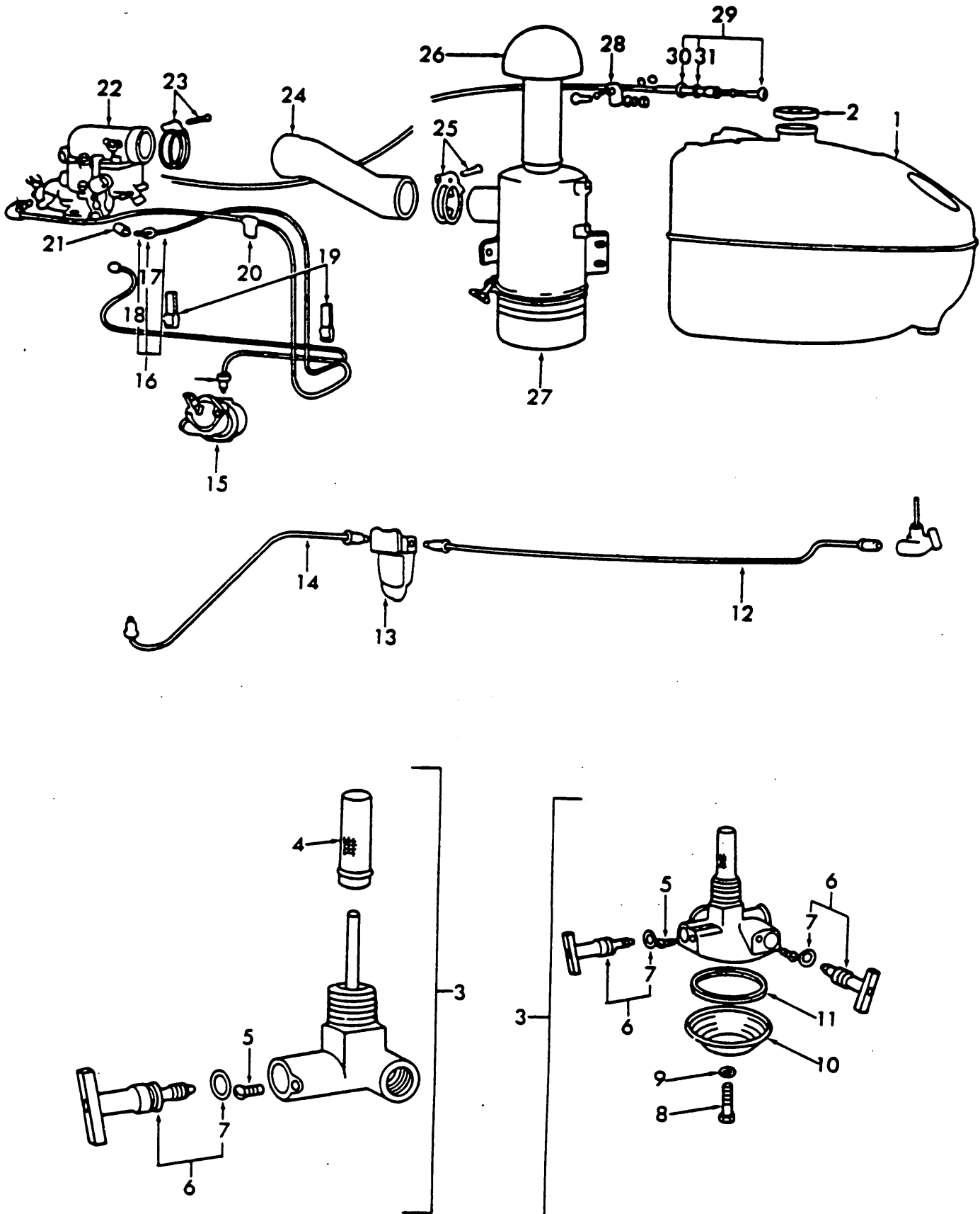
Fig. 60 - Fuel System - Petrol & Vapor
