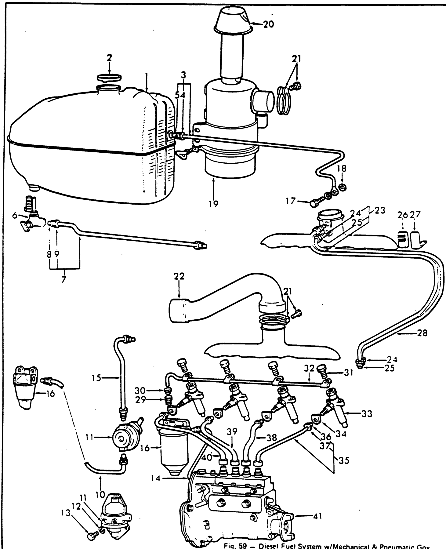
Fig. 59 — Diesel Fuel System w/Mechanical & Pneumatic Gov.
