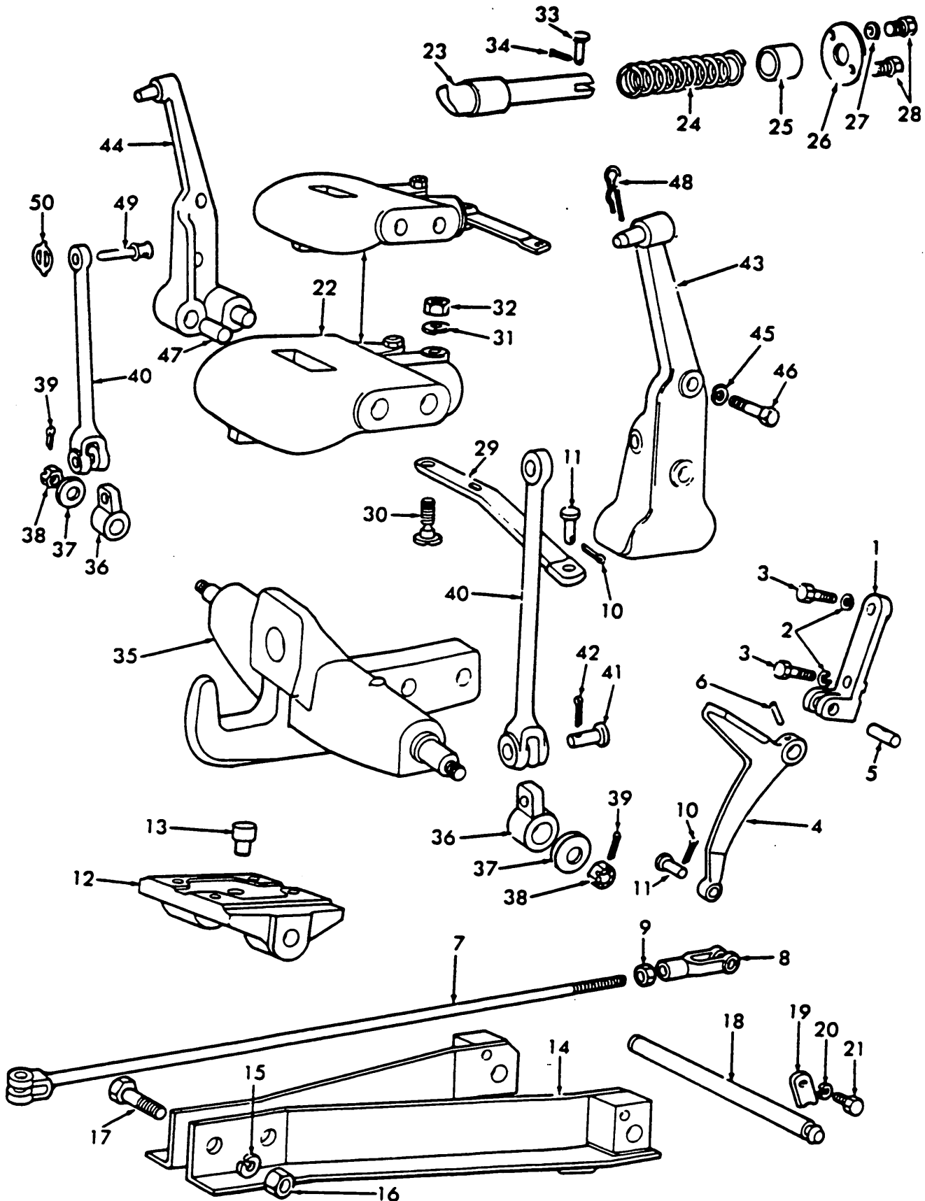
Fig. 33 - Automatic Hitch 52/11-60
