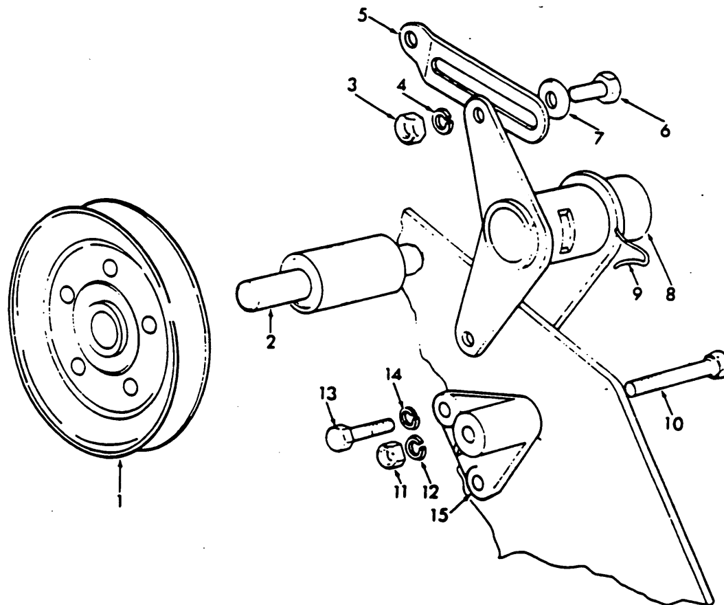
Fig. 58 — Cooling System Idler Pulley
