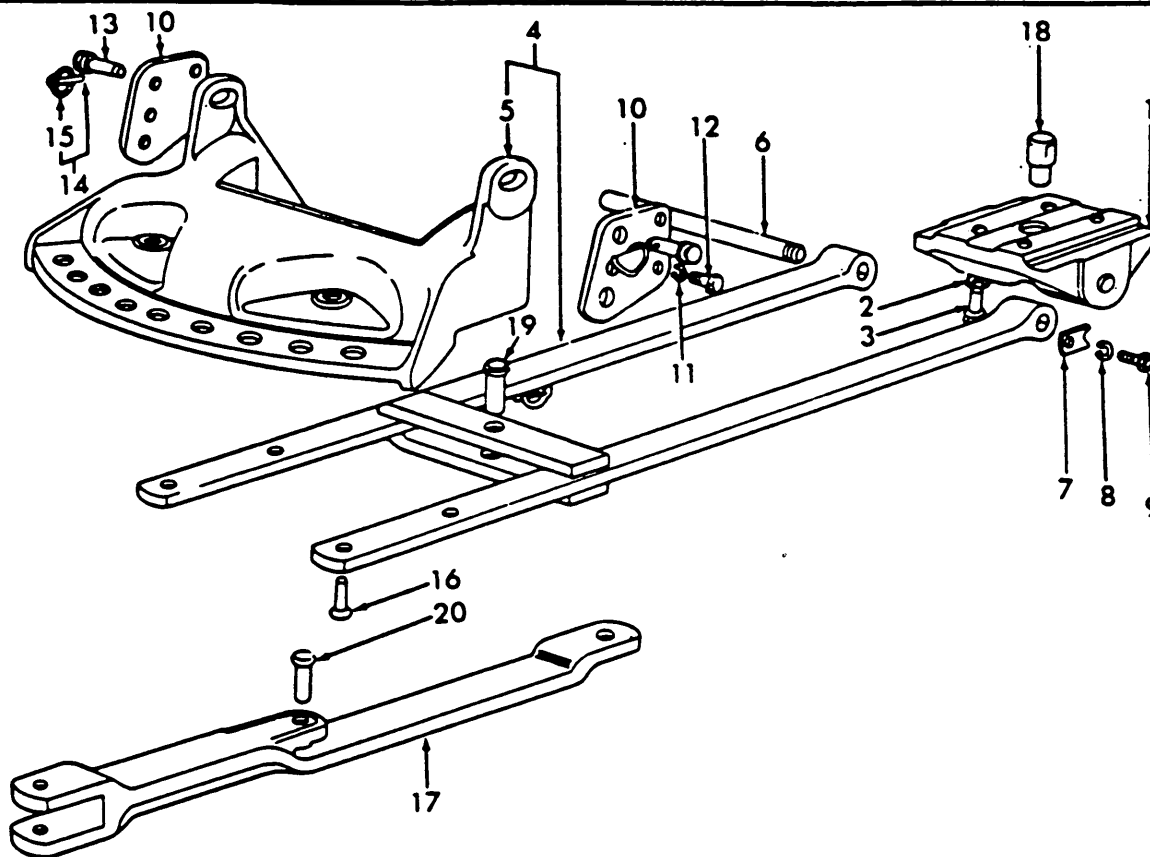
Fig. 37 - Swinging Drawbar
