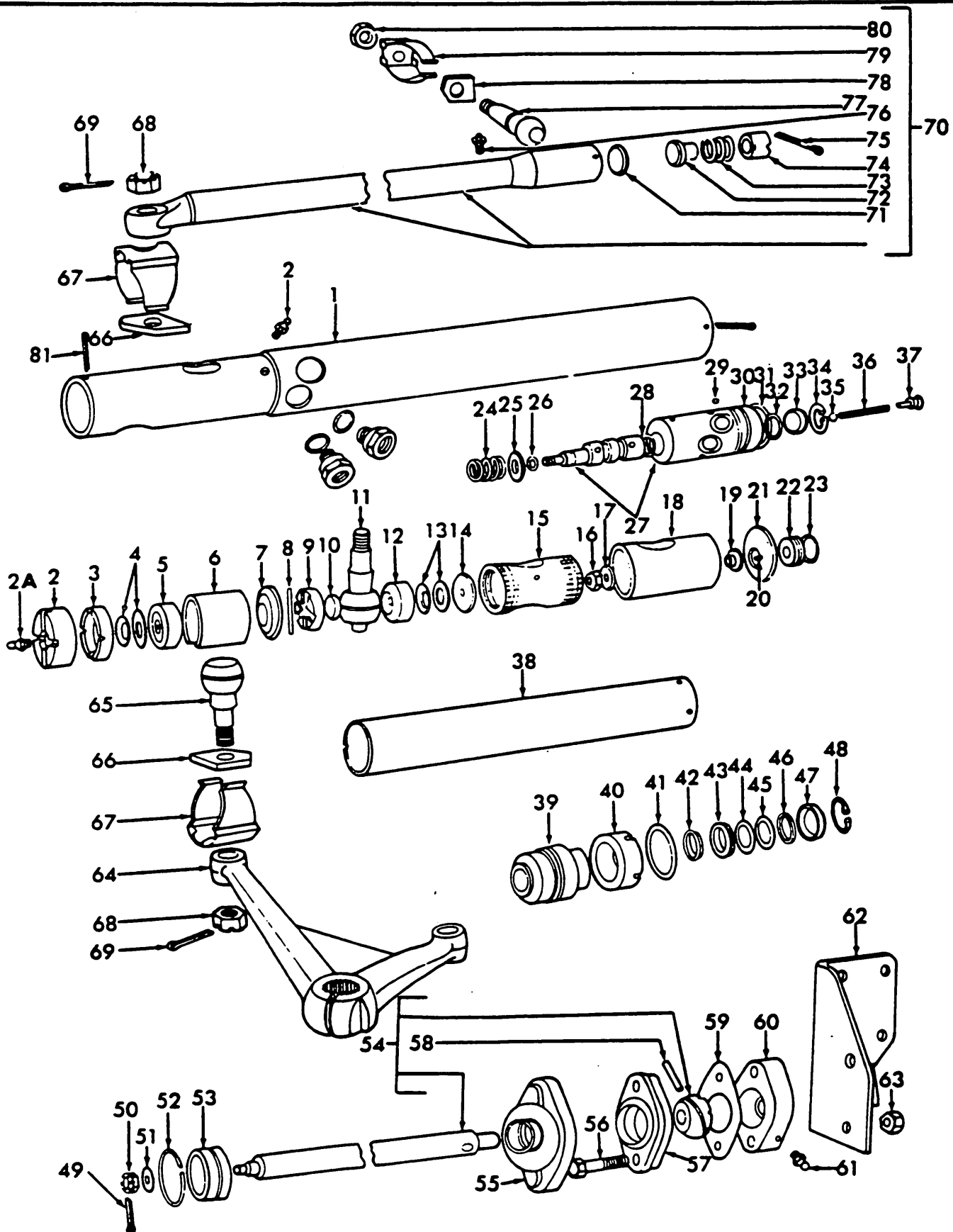
Fig. 15 - Ram Cylinder Unit - Power Steering
