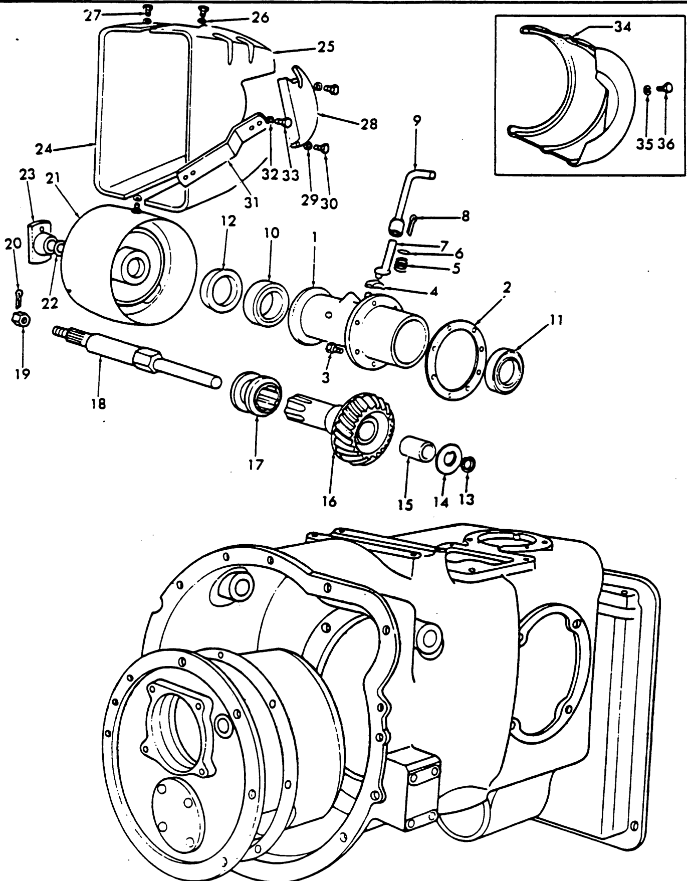
Fig. 55 -- Pulley & Drive Gear
