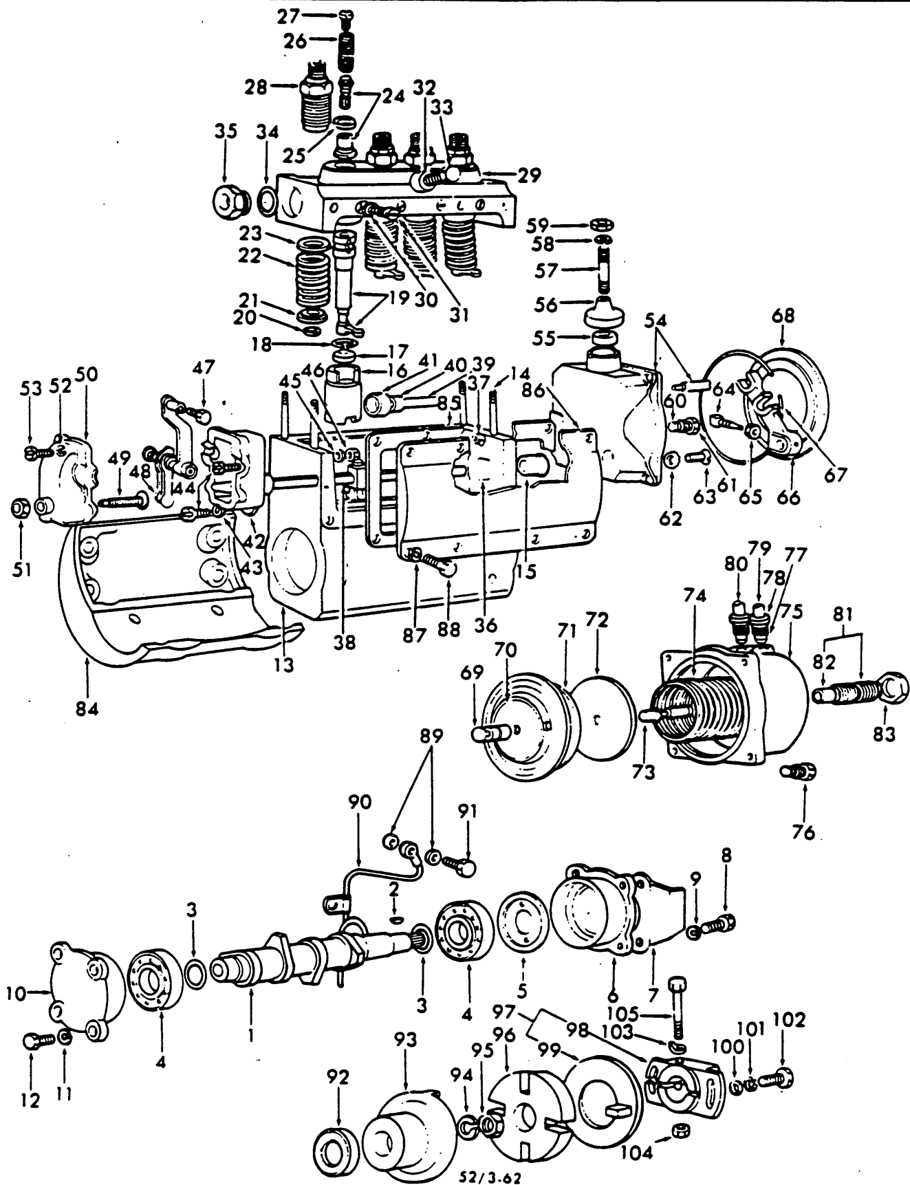
Fig. 69 - Fuel Injection Pump Assy. 52/3-62
