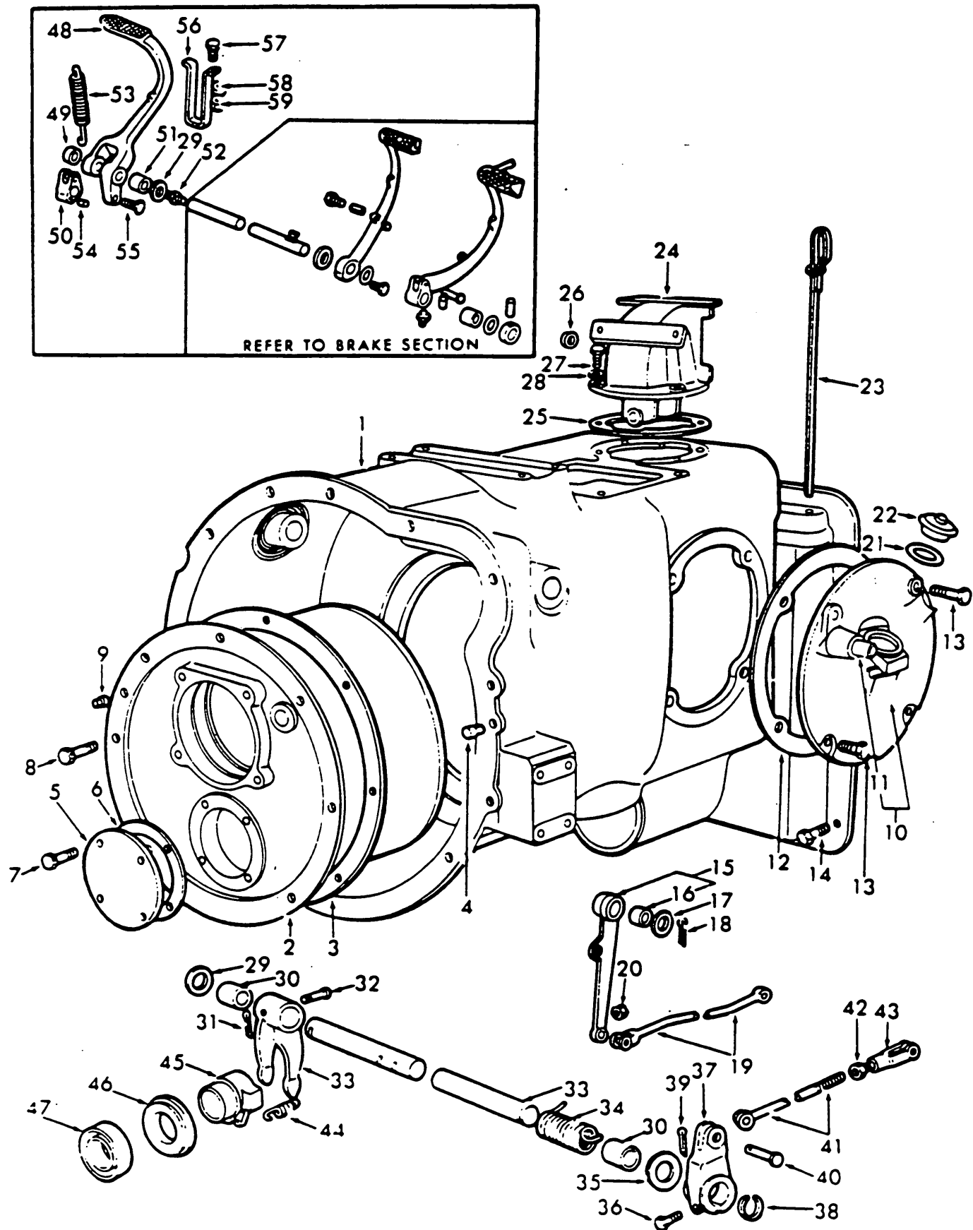
Fig. 50 - Transmission, Clutch & PTO
