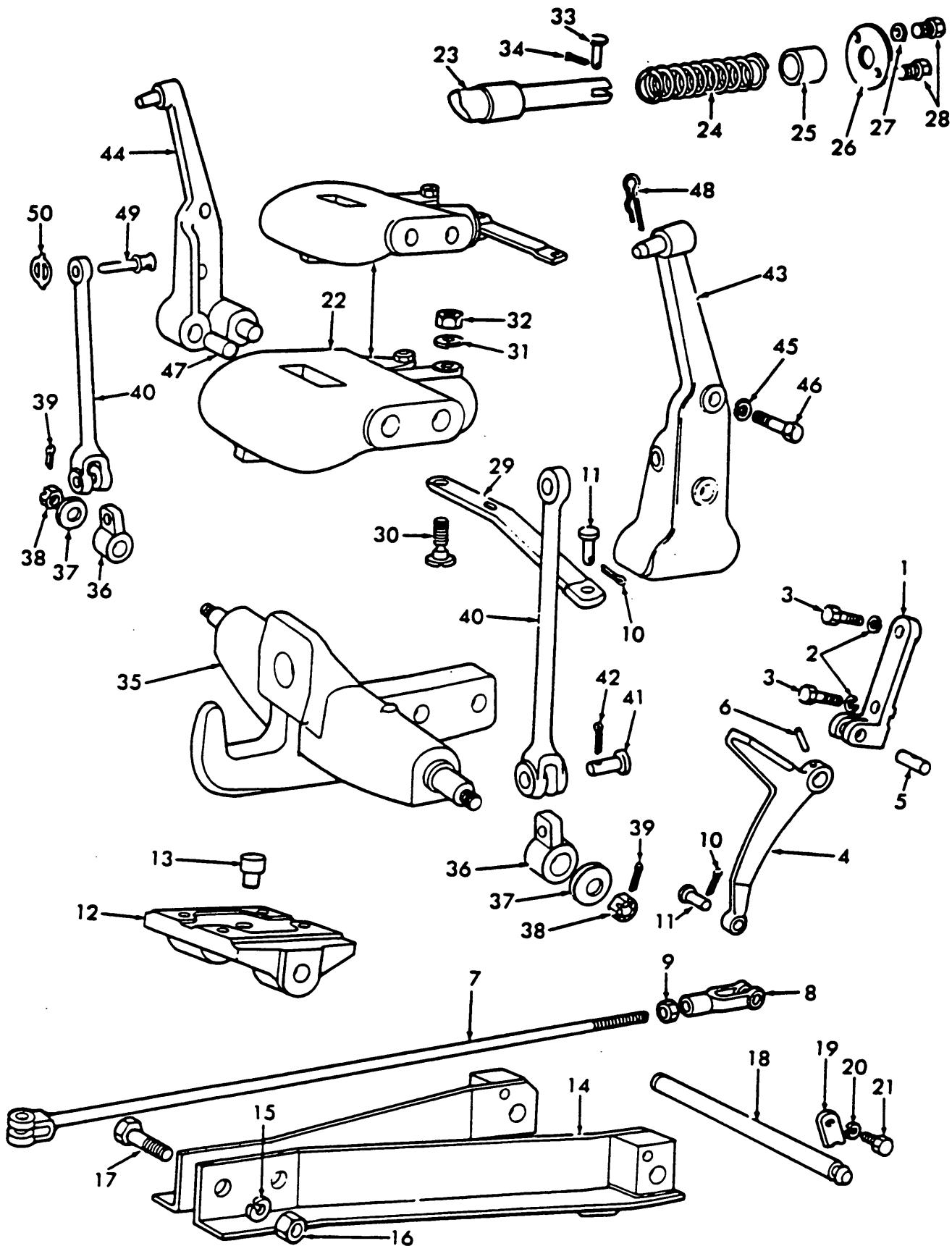
Fig. 33 - Automatic Hitch 52/11-60
