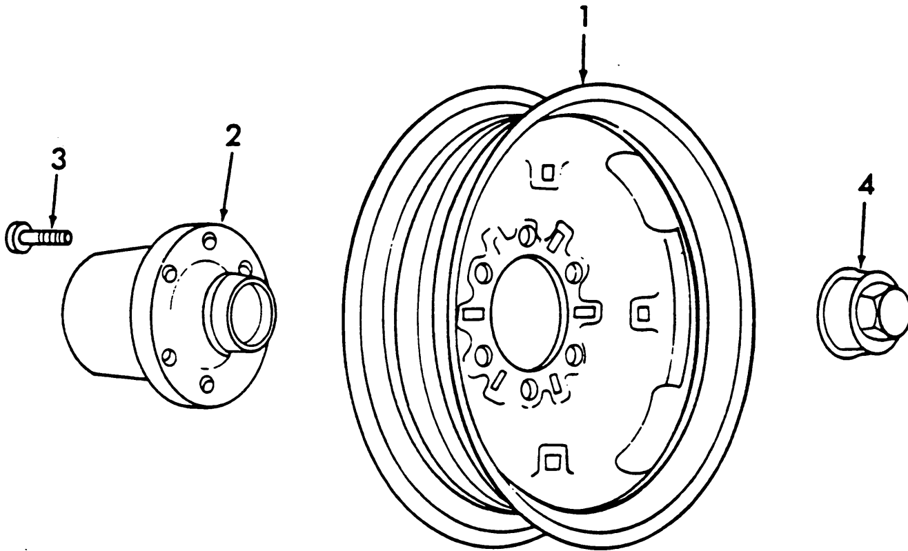
Fig. 1 - Front Wheels
