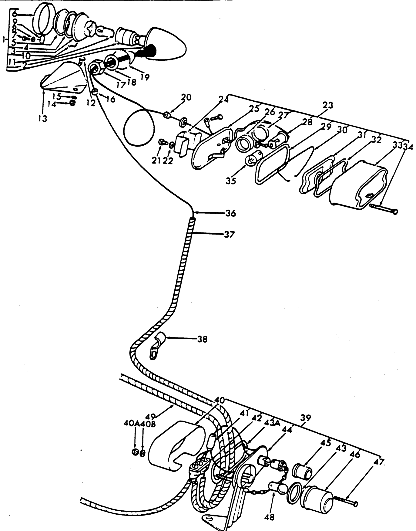
Fig. 79 - Side & Rear Lamps
