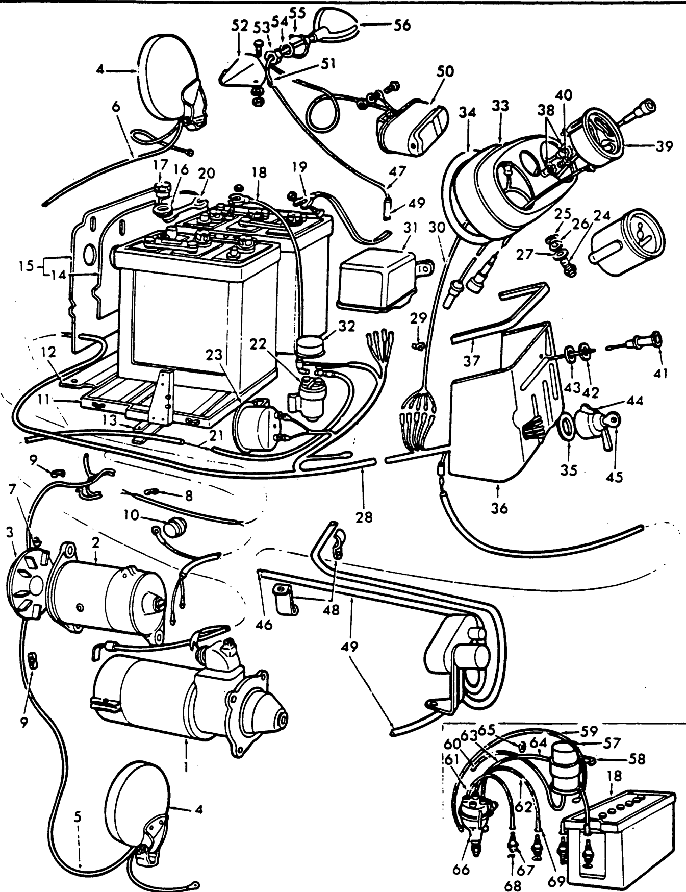
Fig. 77 - Electrical System
