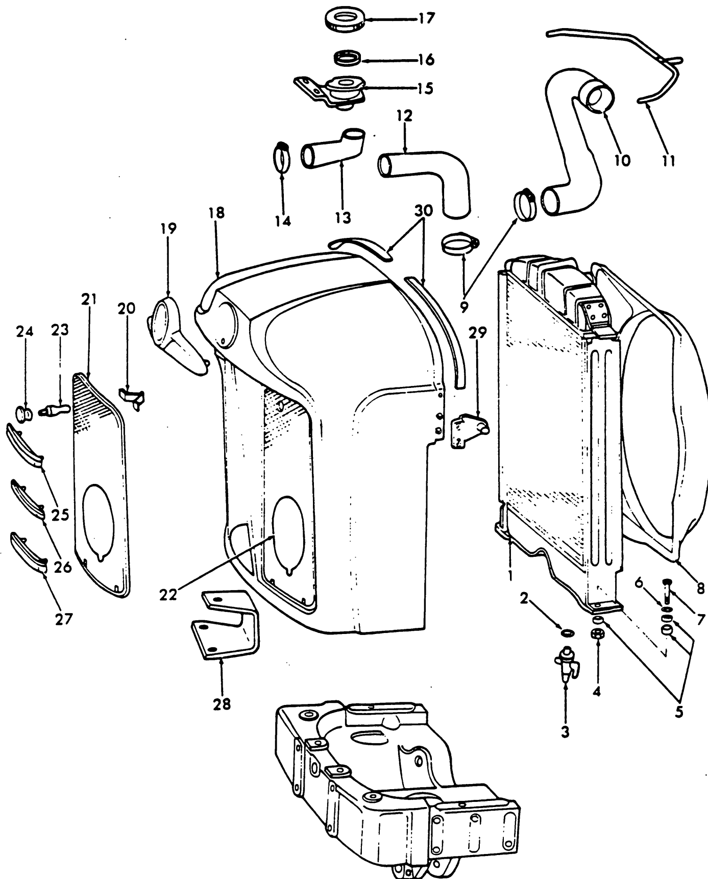
Fig. 56 - Cooling System
