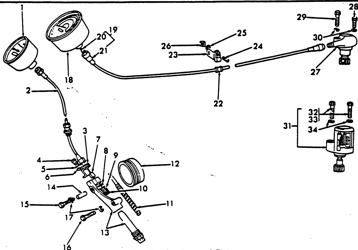
Fig. 87 — Speedometer & Tachometer
