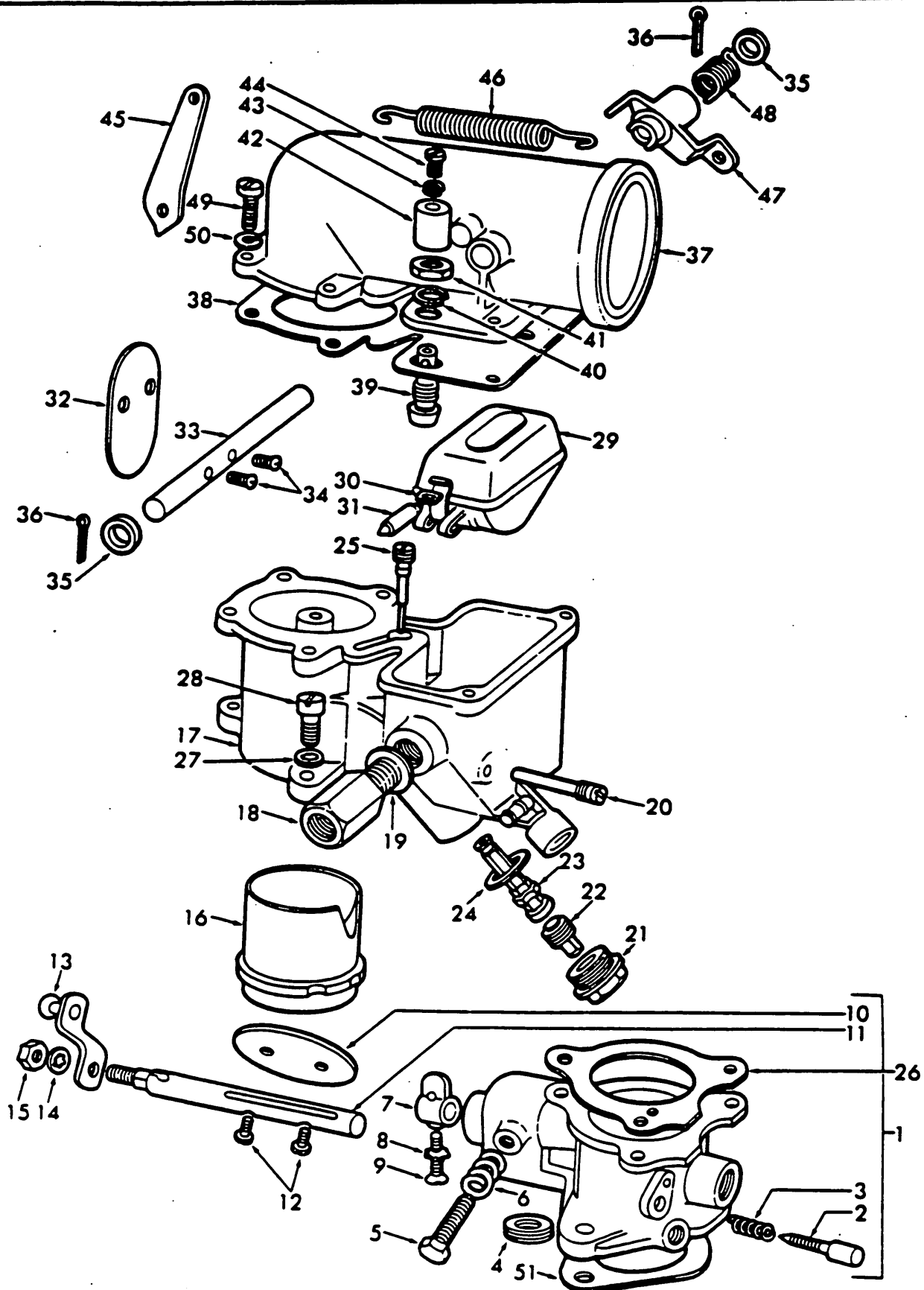
Fig. 67 - Fuel System Carburetor
