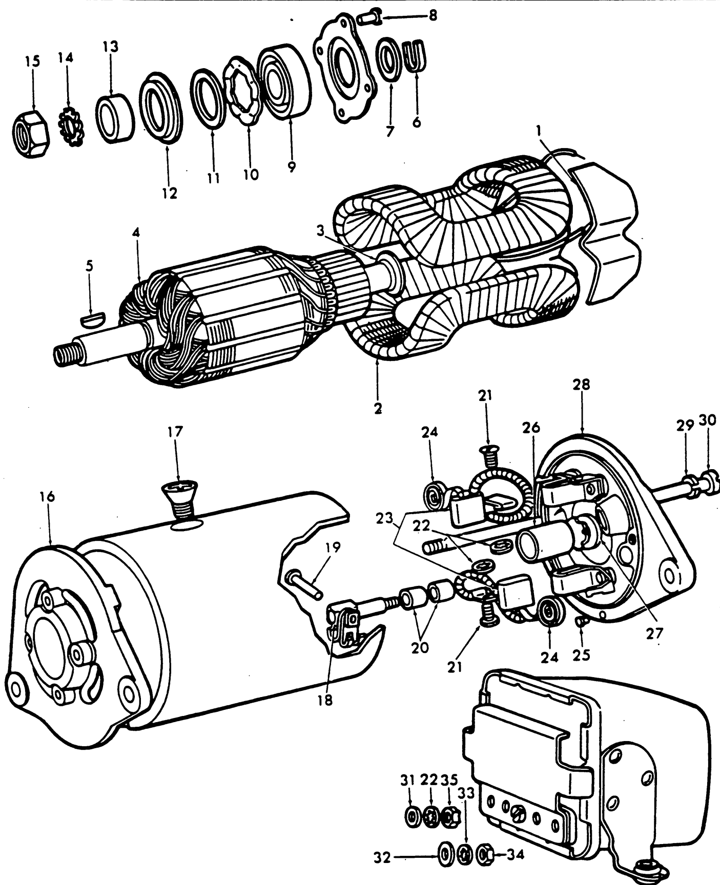
Fig. 86 - Generator & Regulator
