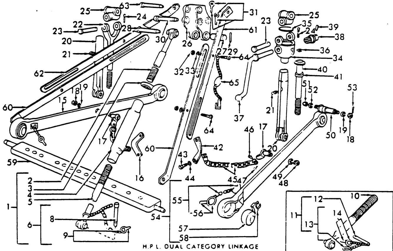
Fig. 12 Hyd. Lift Linkage
