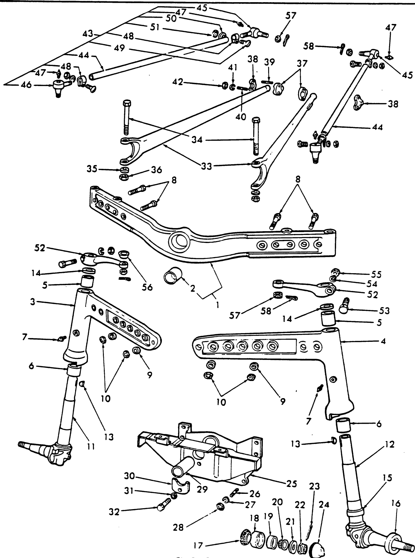
Fig. 5 Front Axle
