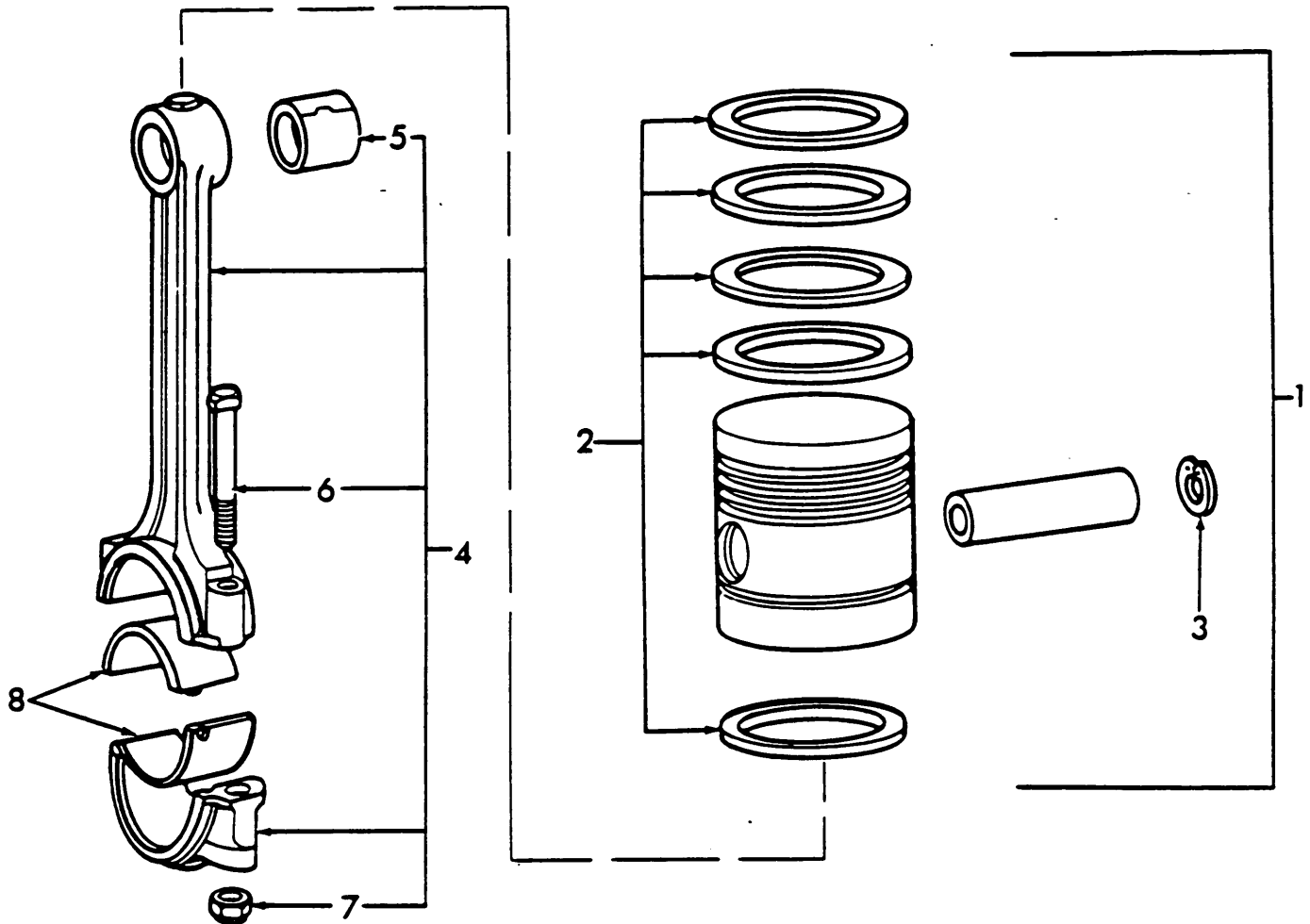
Fig. 22 Piston & Connecting Rods
