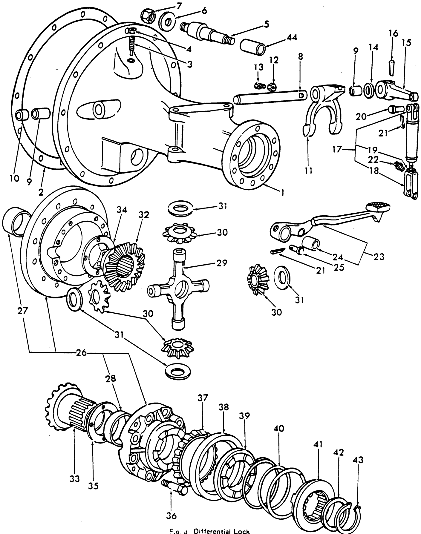
F.g. 3 Differential Lock
