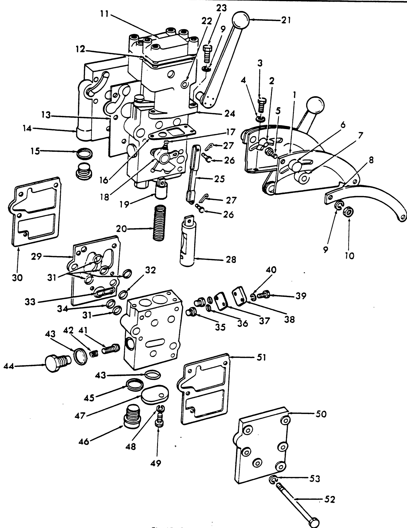
Fig. 17 Dual Auxiliary Valve
