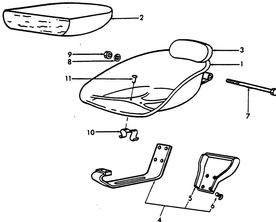
Fig. 54 Seat Assemblies
