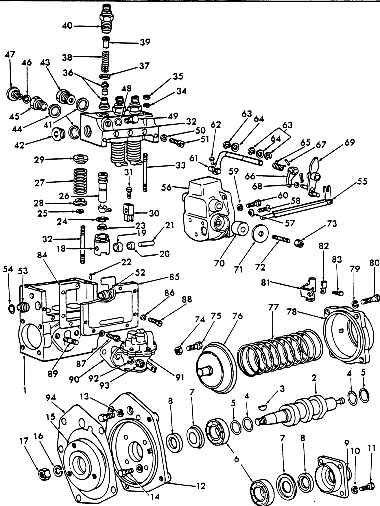
Fig. 42 Fuel Injection Pump w/Pneumatic Gov. 57/3-62
