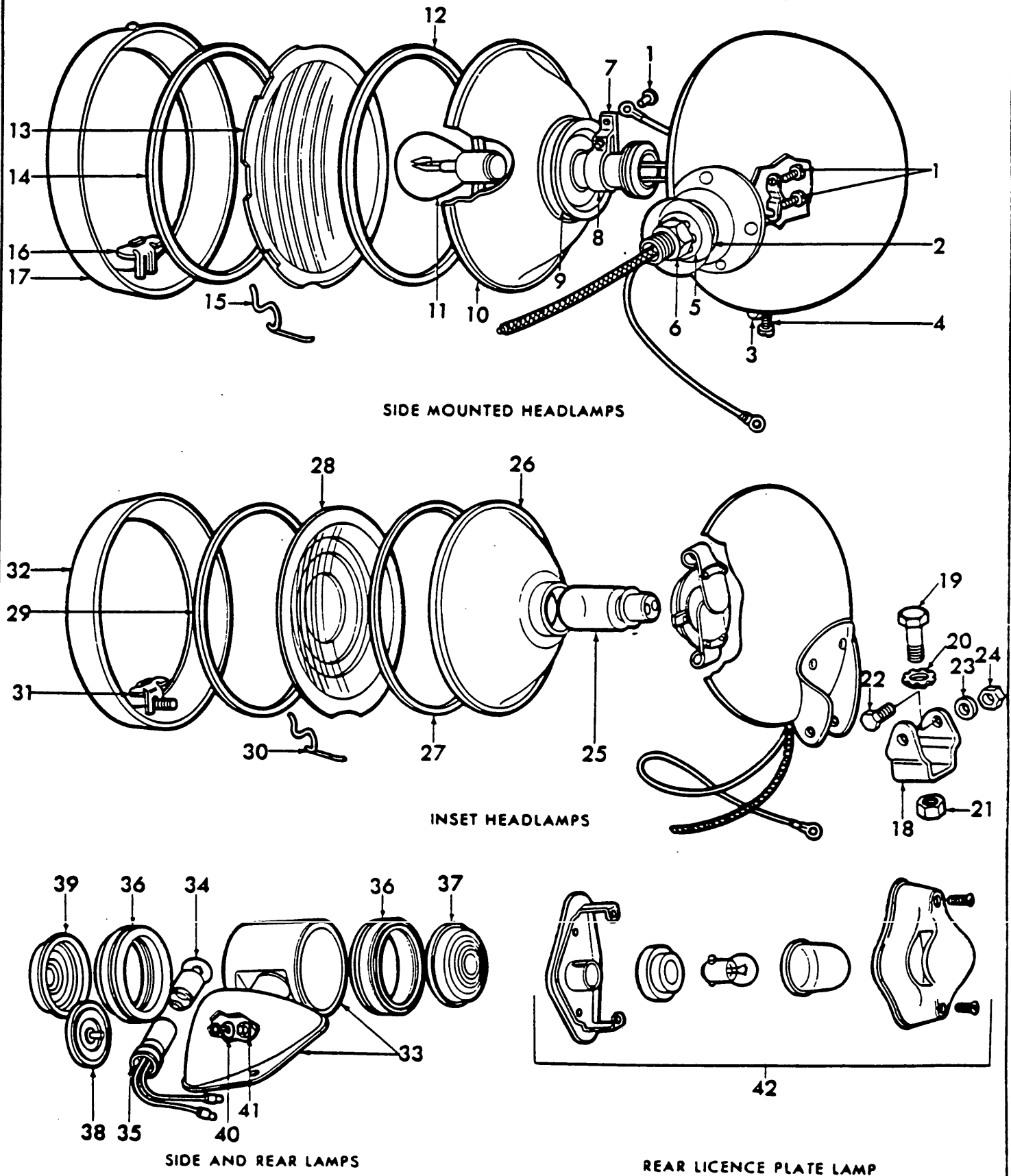
Fig. 47 Head & Rear Lamps
