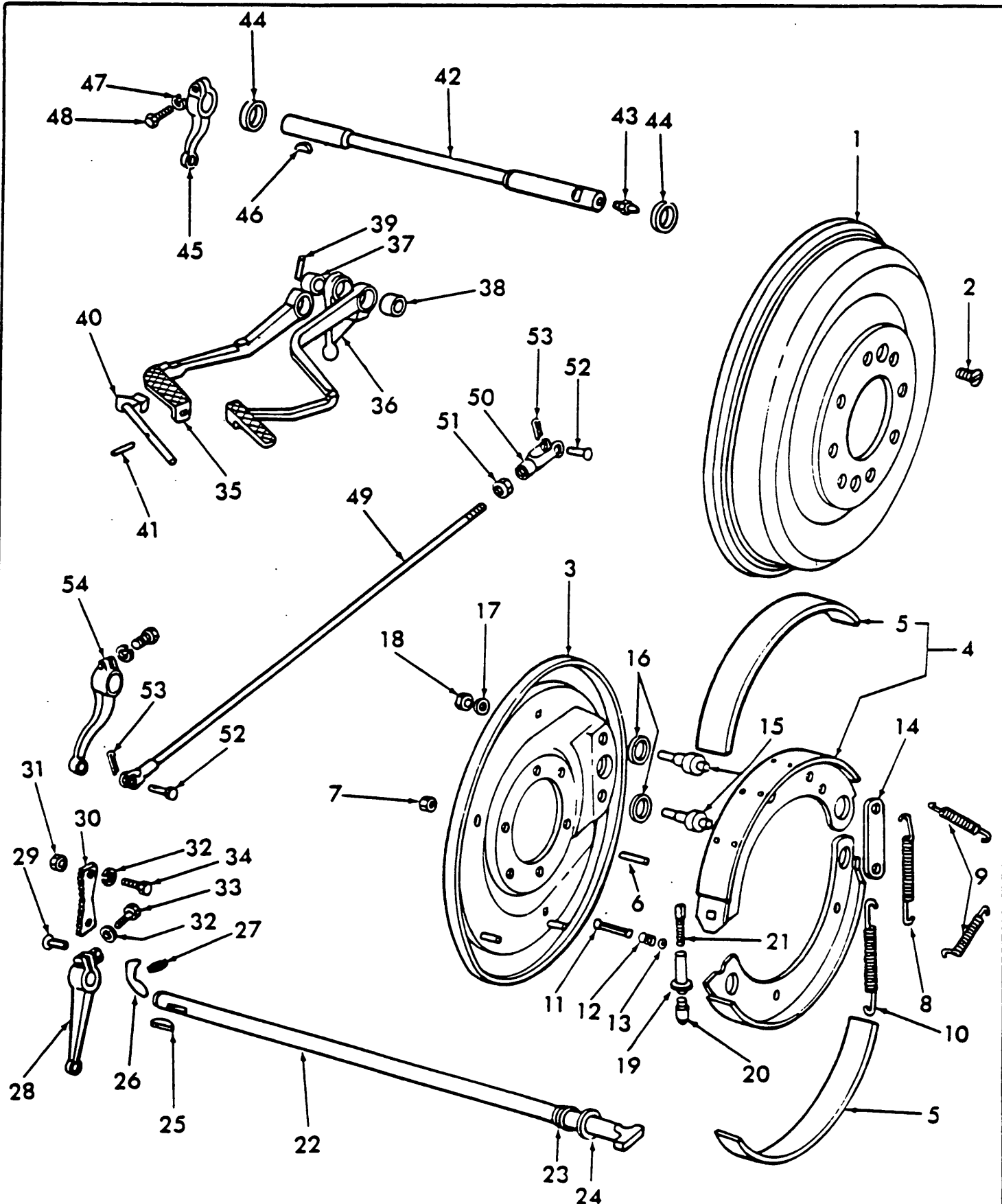
Fig. 2 Brakes
