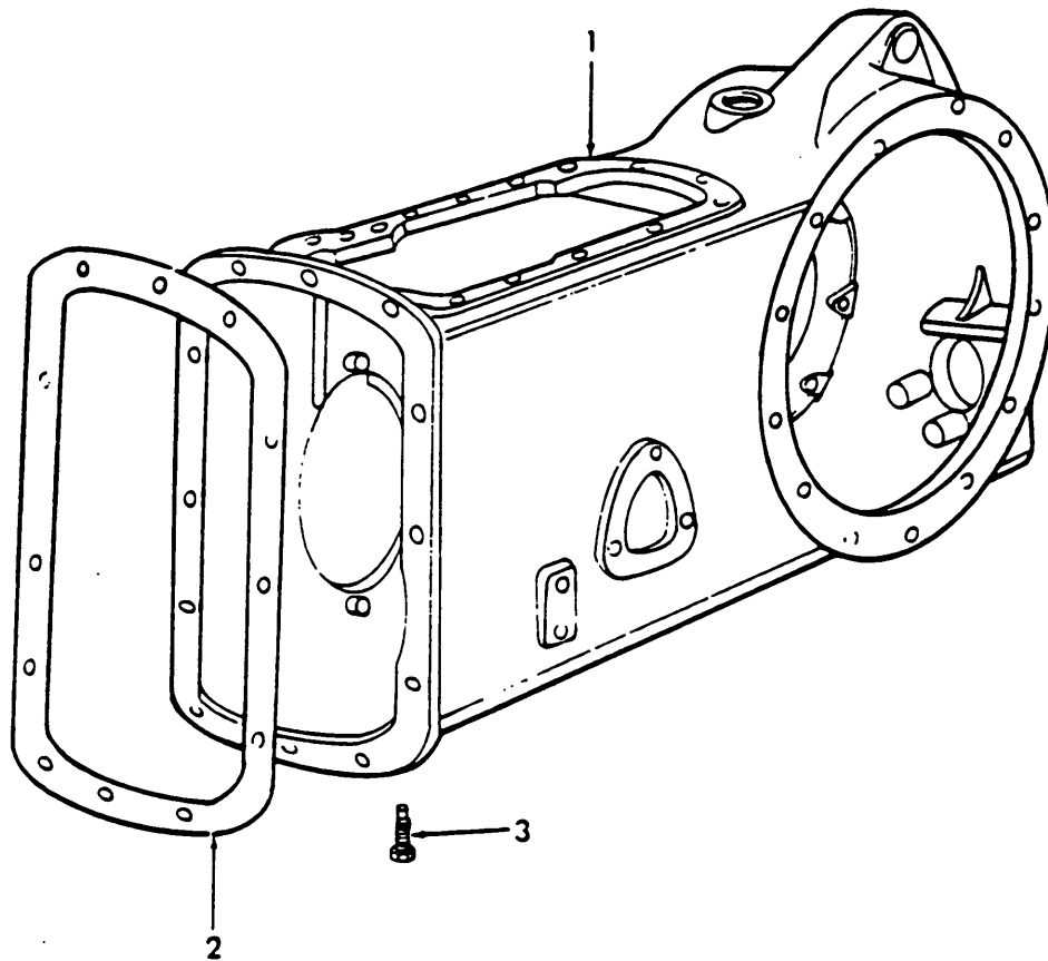
Fig. 9 Differential Housing
