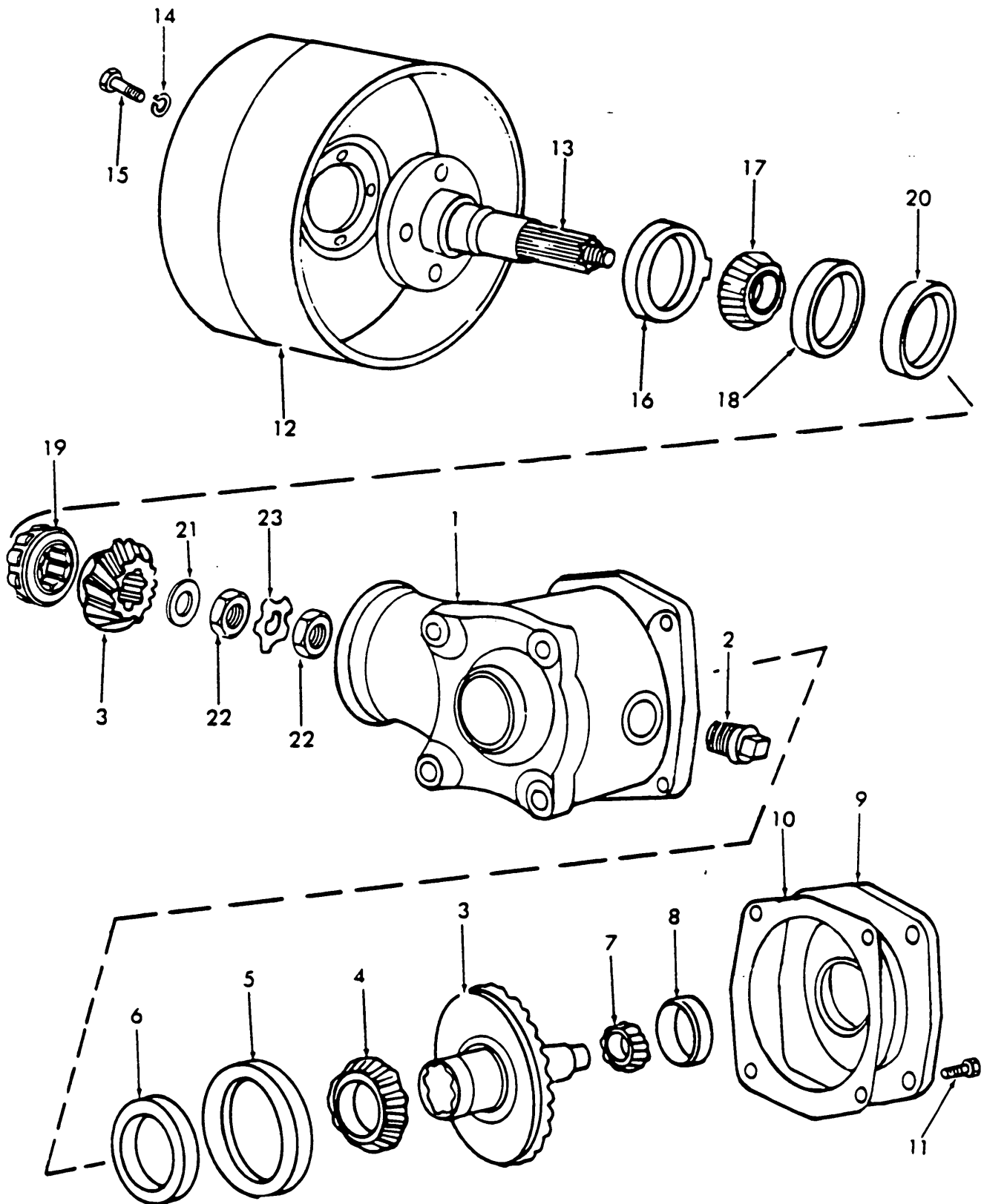
Fig. 33 Pulley Assy.
