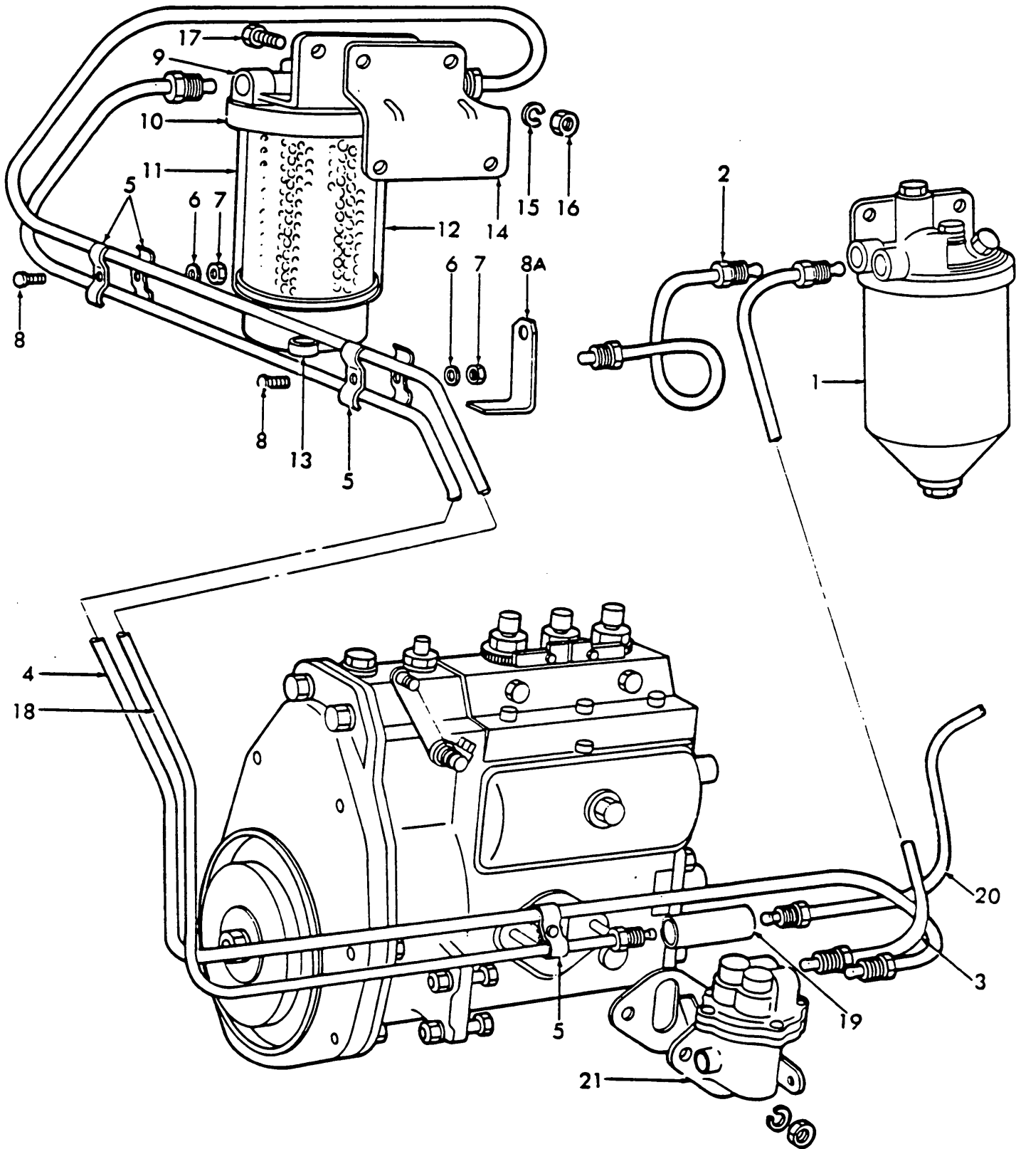
Fig. 39 Dual Fuel Oil Filters & Related Parts
