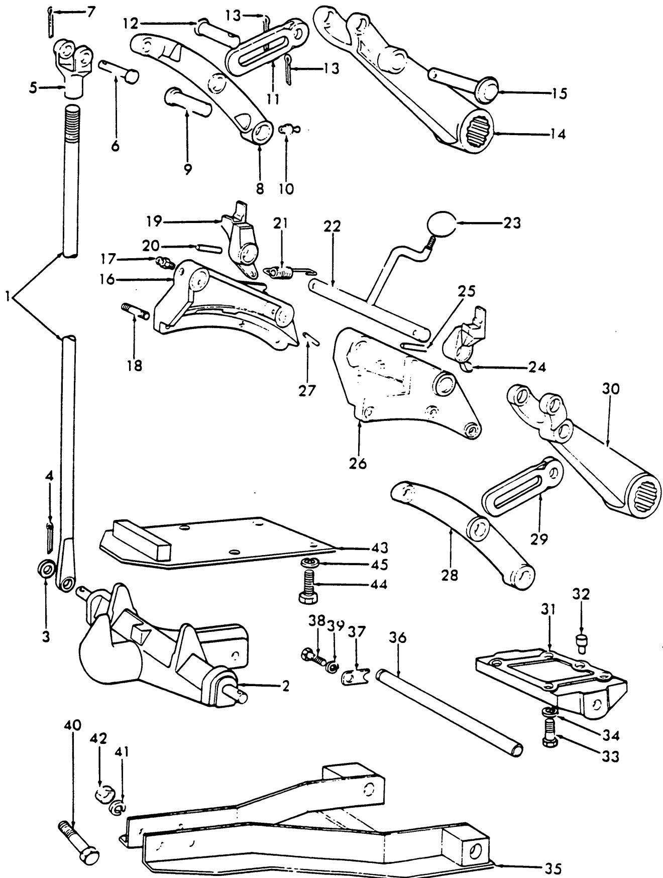
Fig. 15 Automatic Pick-Up Hitch
