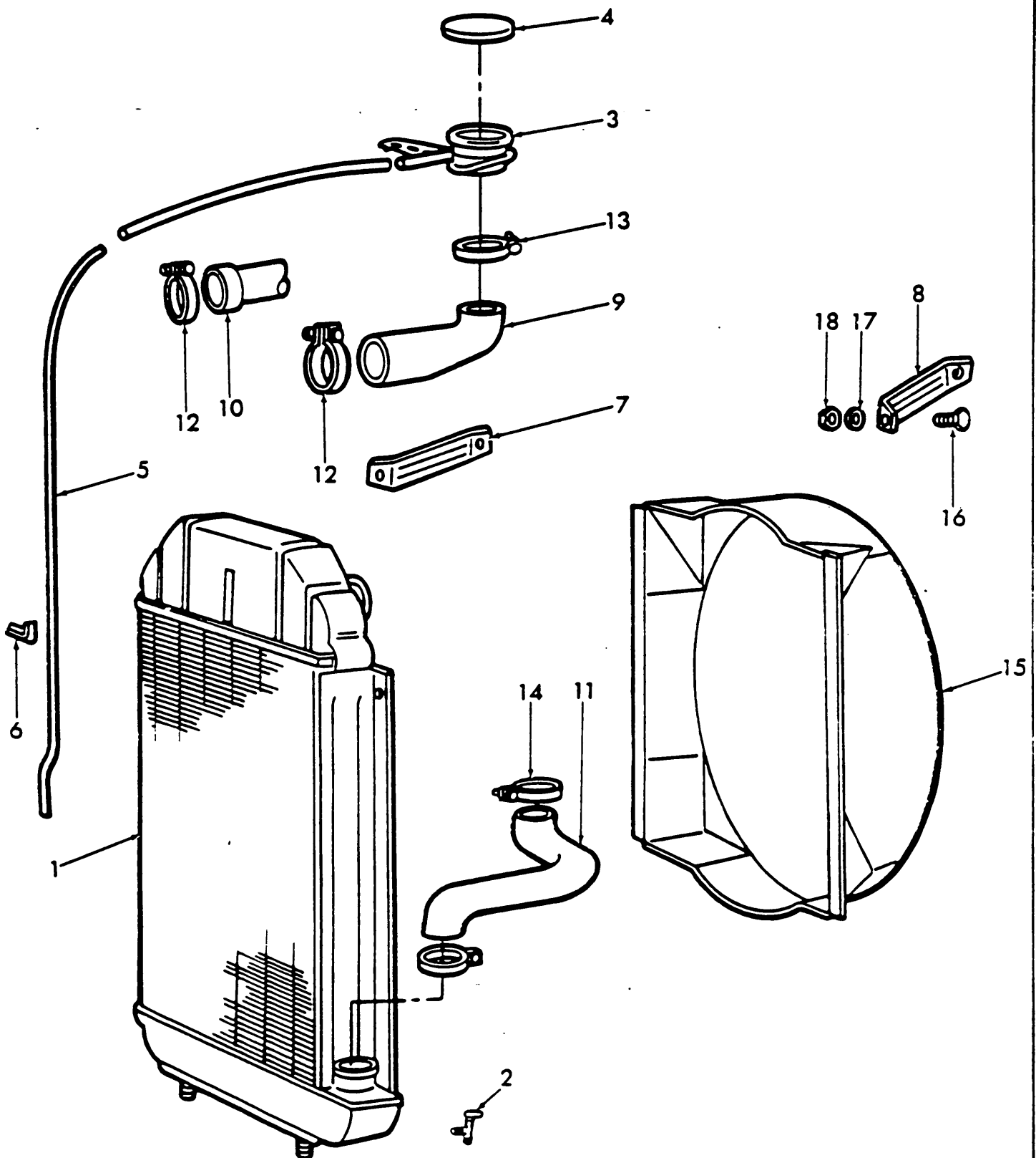
Fig. 35 Radiator & Related Parts
