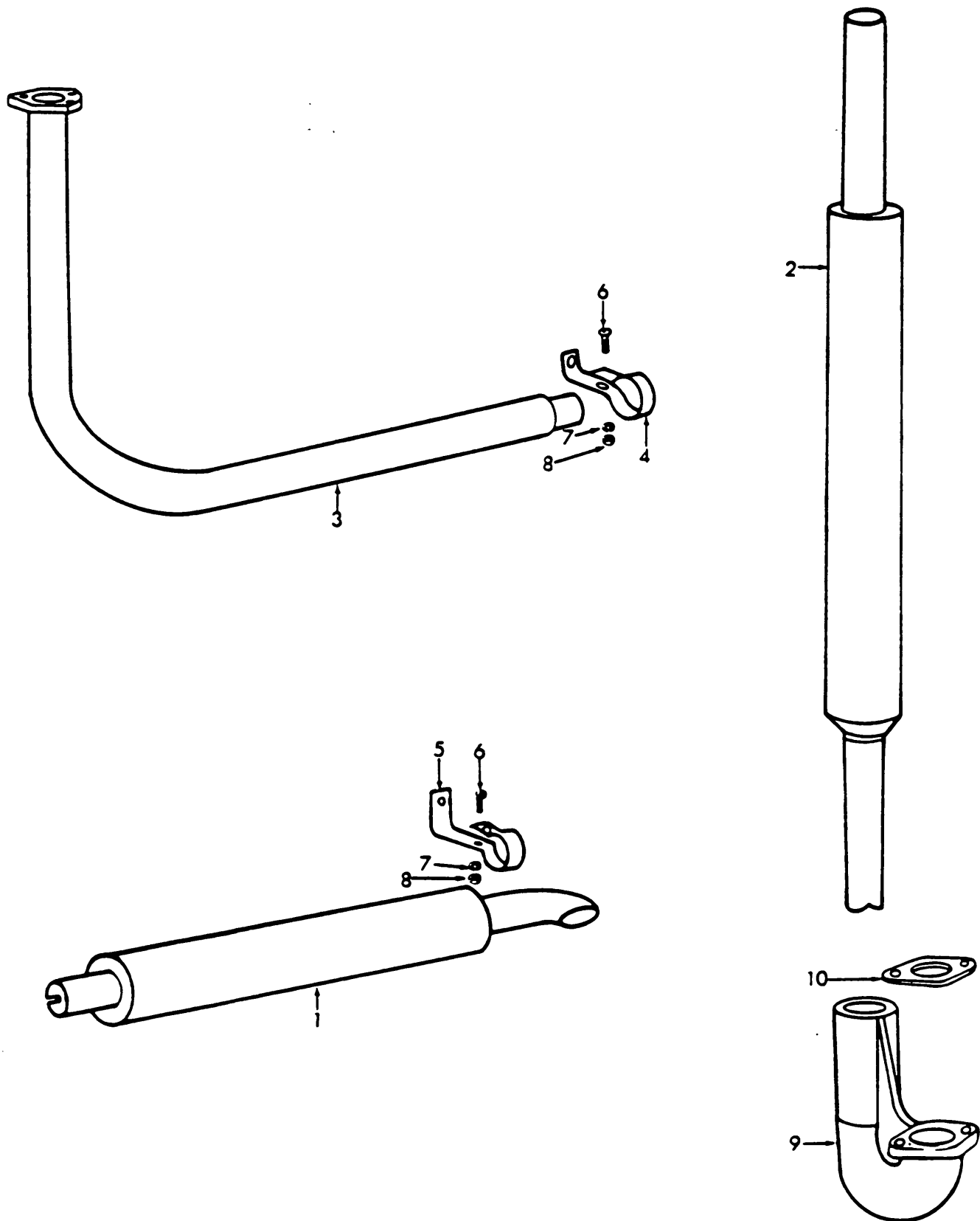
Fig. 26 Mufflers & Related Parts
