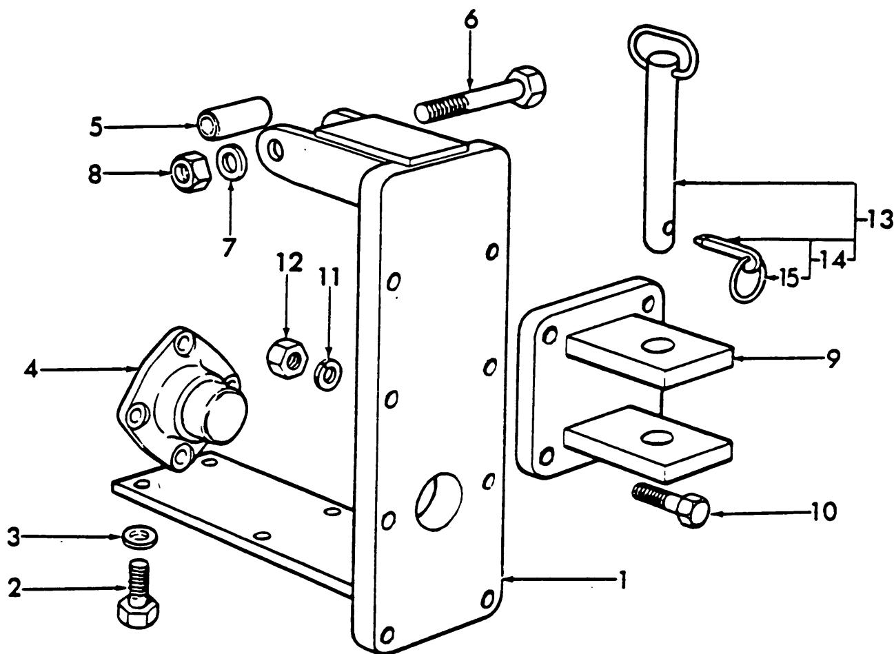
Fig. 57 Drawbar Bracket & Towing Hitch Assy.
