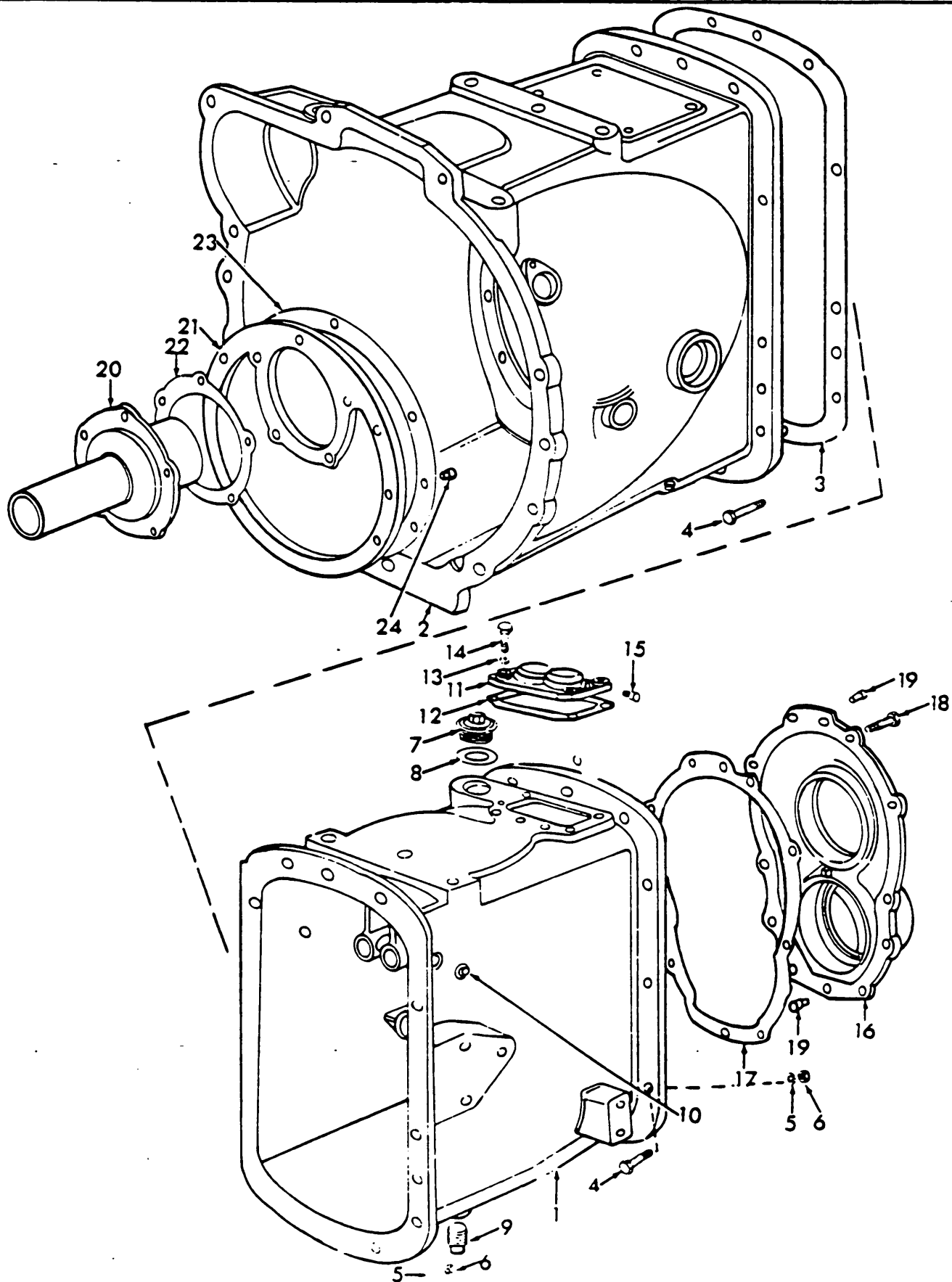
Fig. 27 Transmission & Clutch Housing
