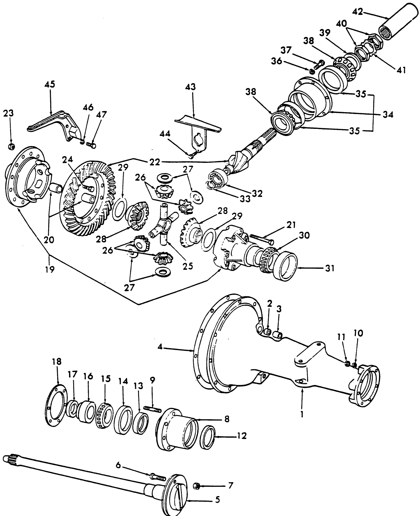
Fig. 7 Rear Axle & Differential
