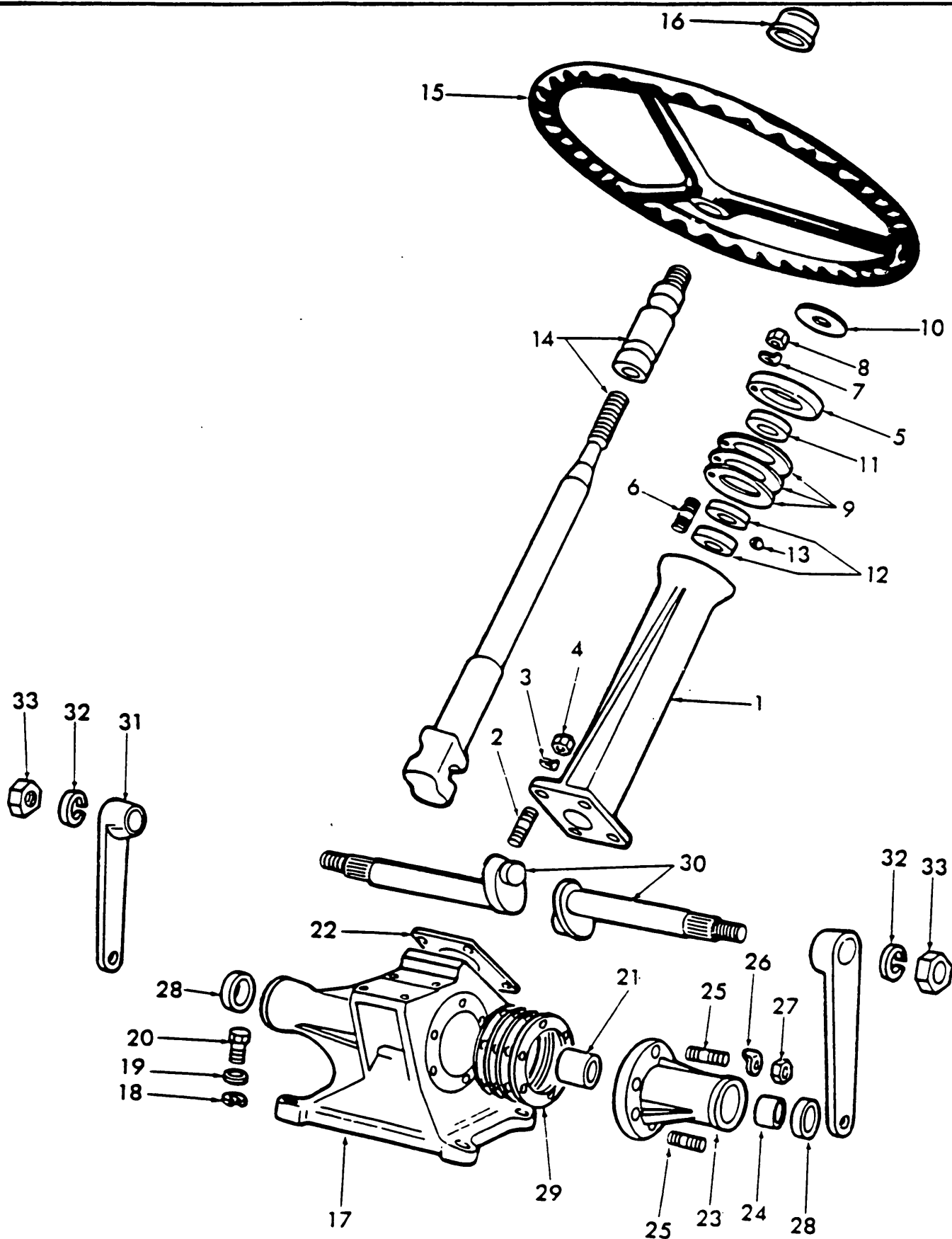
Fig. 6 Steering Gear
