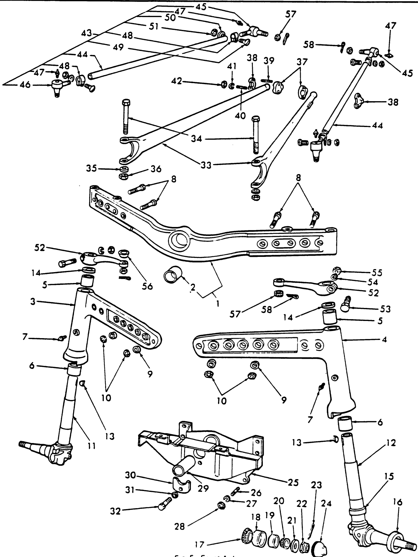
Fig. 5 Front Axle
