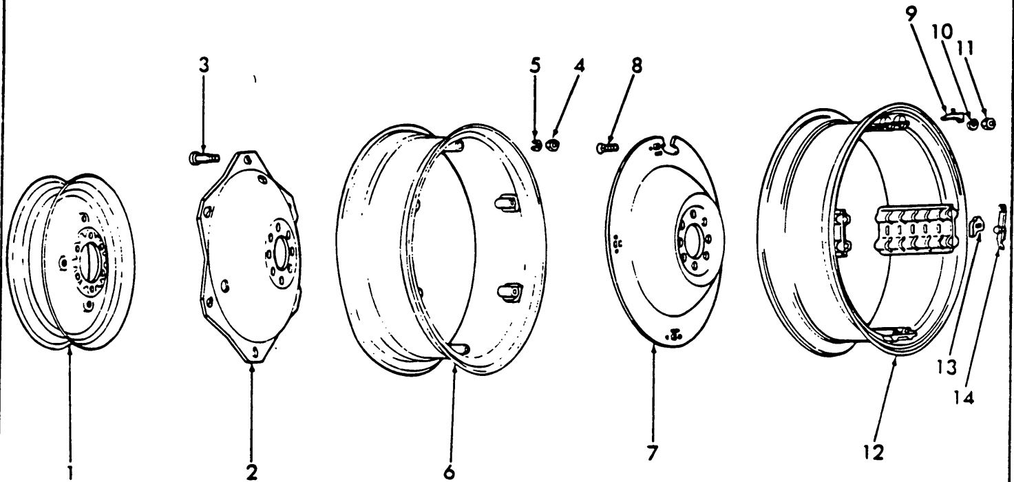
Fig. 1 Wheels & Weights
