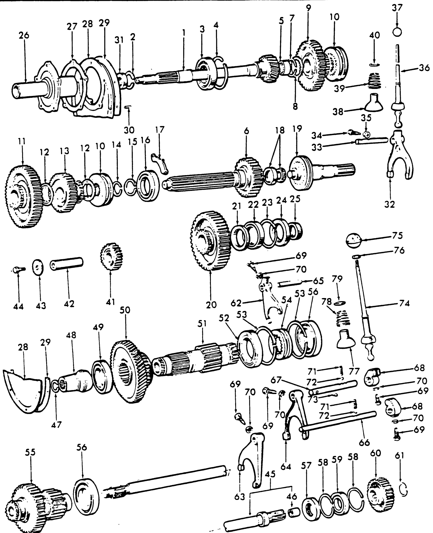
Fig. 25 Front Transmission Interior
