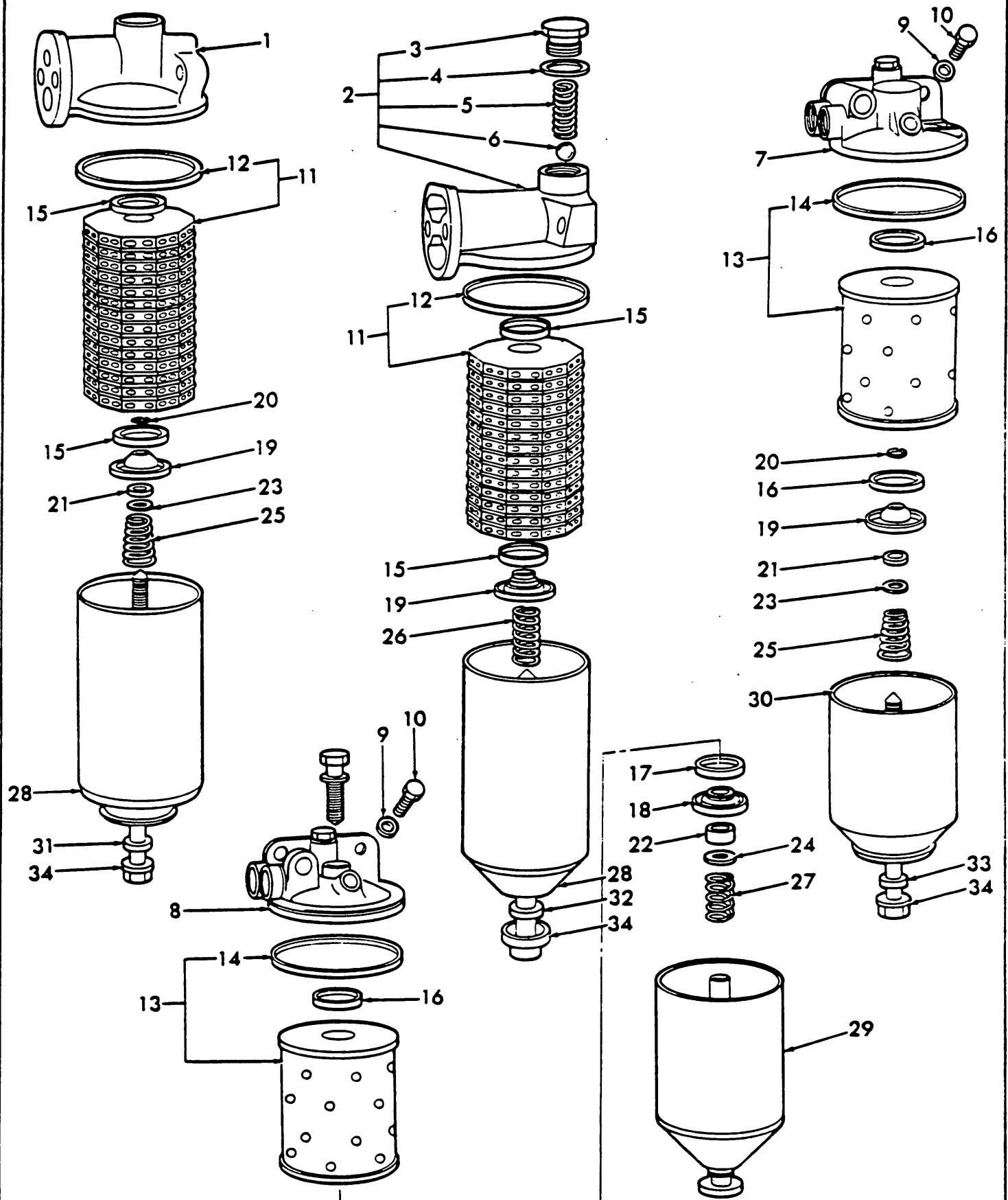
Fig. 38 Engine & Fuel Oil Filters
