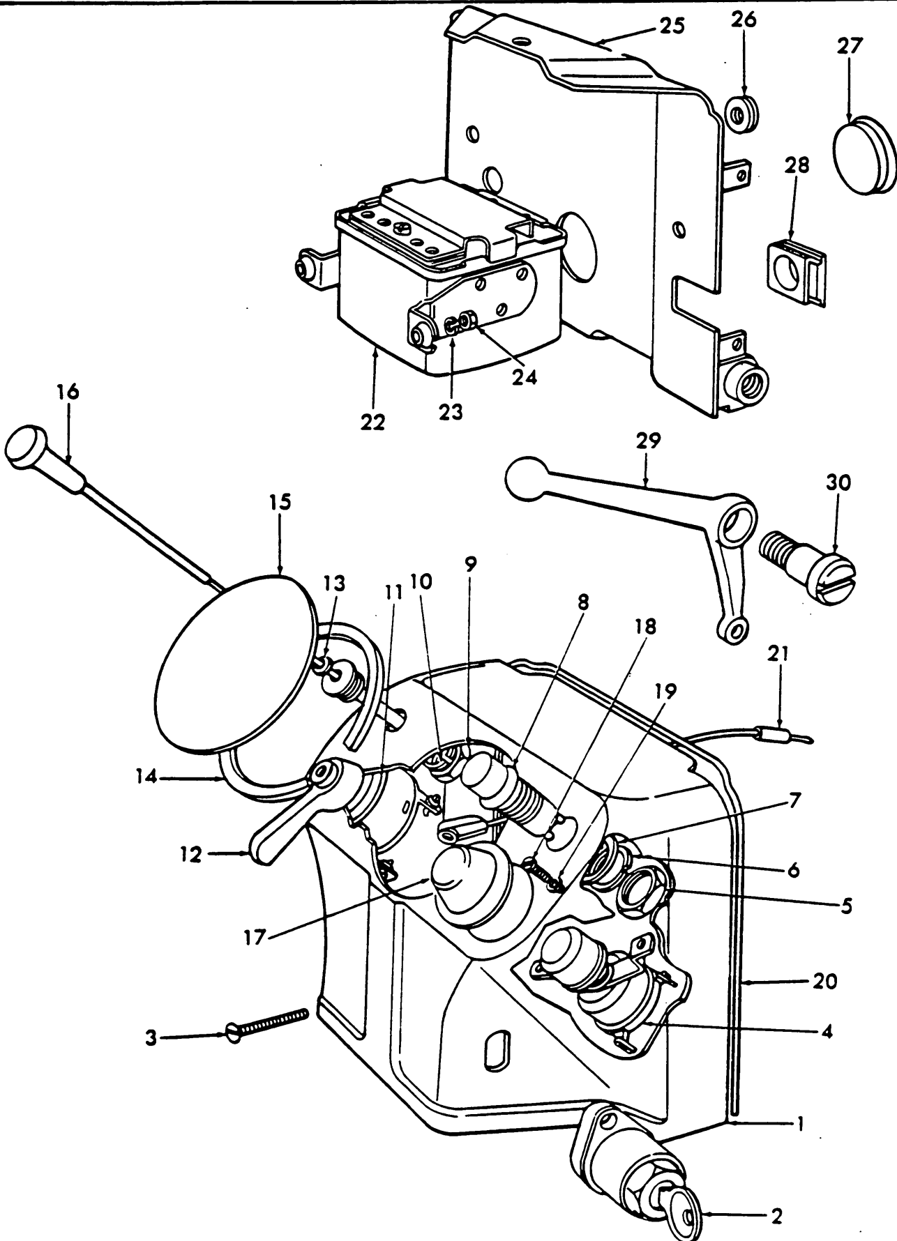
Fig. 52 Instrument Box
