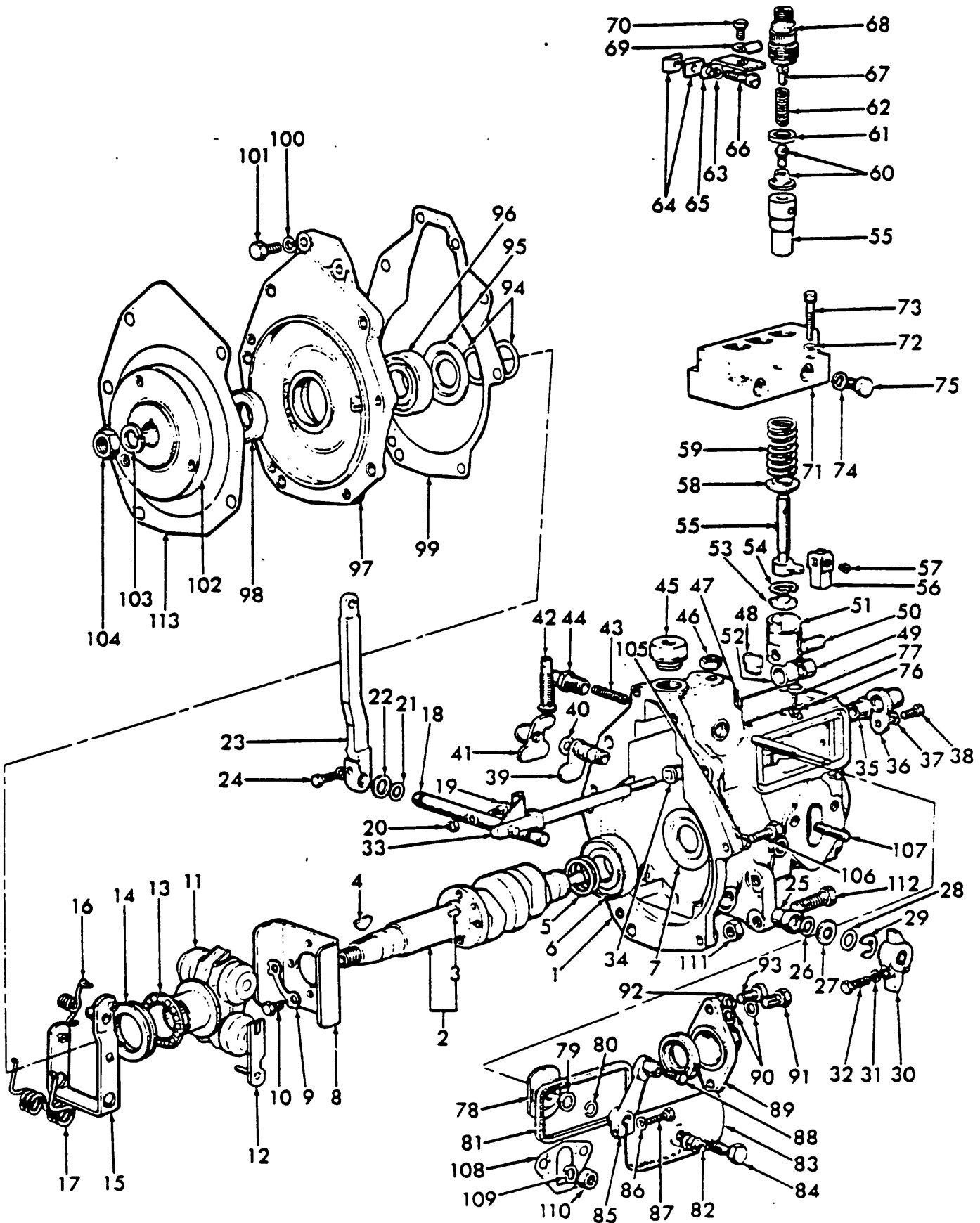
Fig. 43 Fuel Injection Pump w/Mechanical Governor
