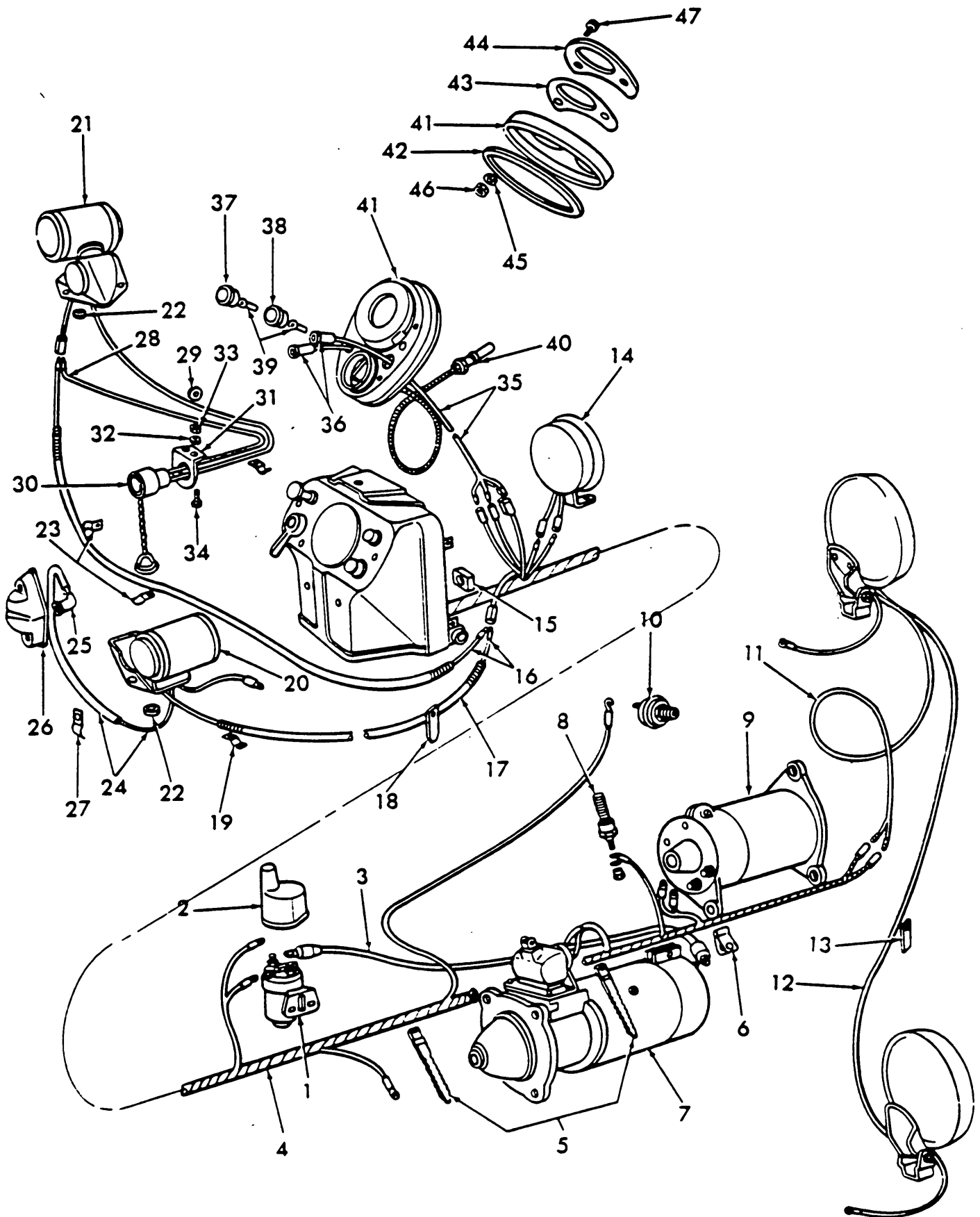
Fig. 46 Electrical System
