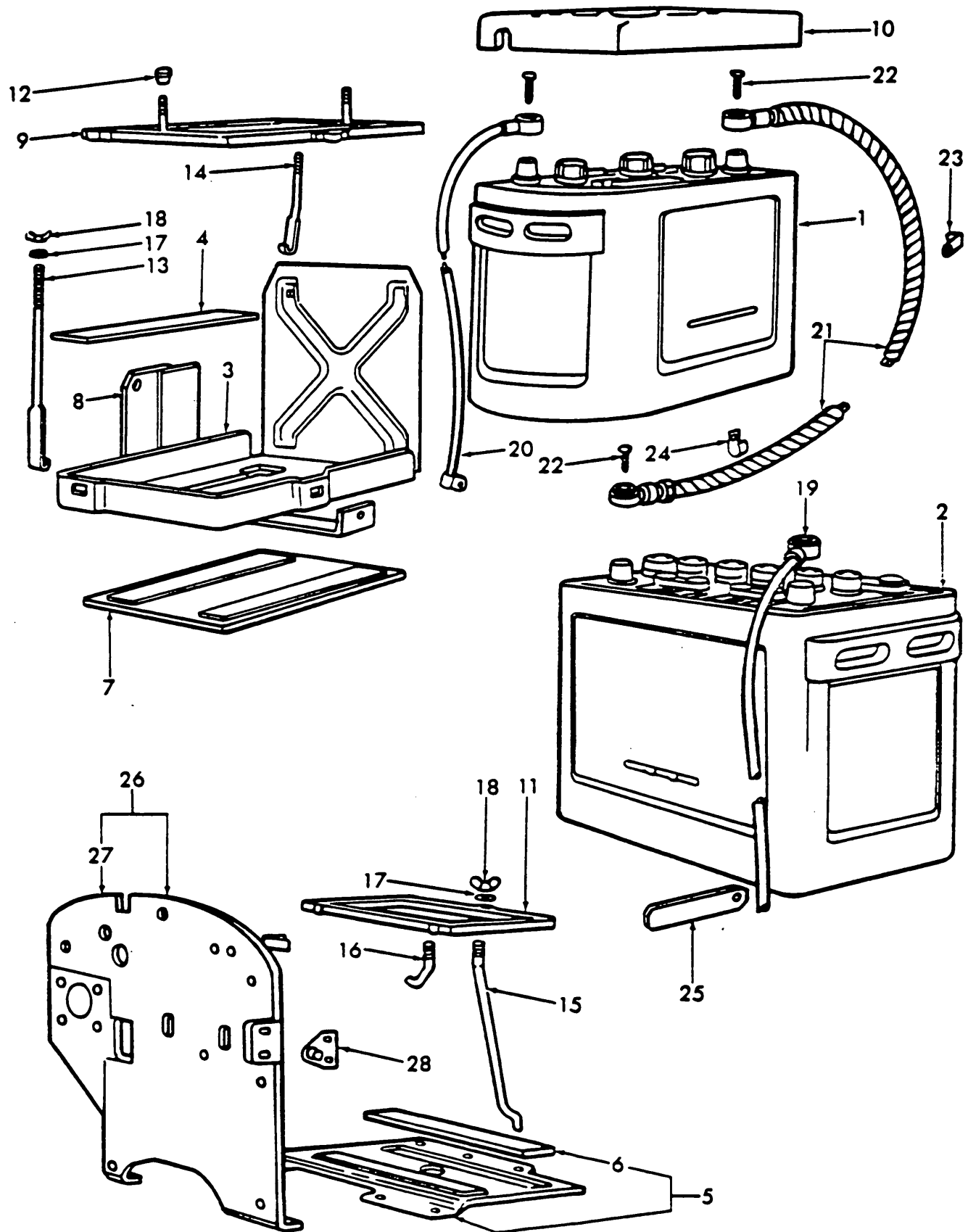
Fig. 48 Battery & Tray
