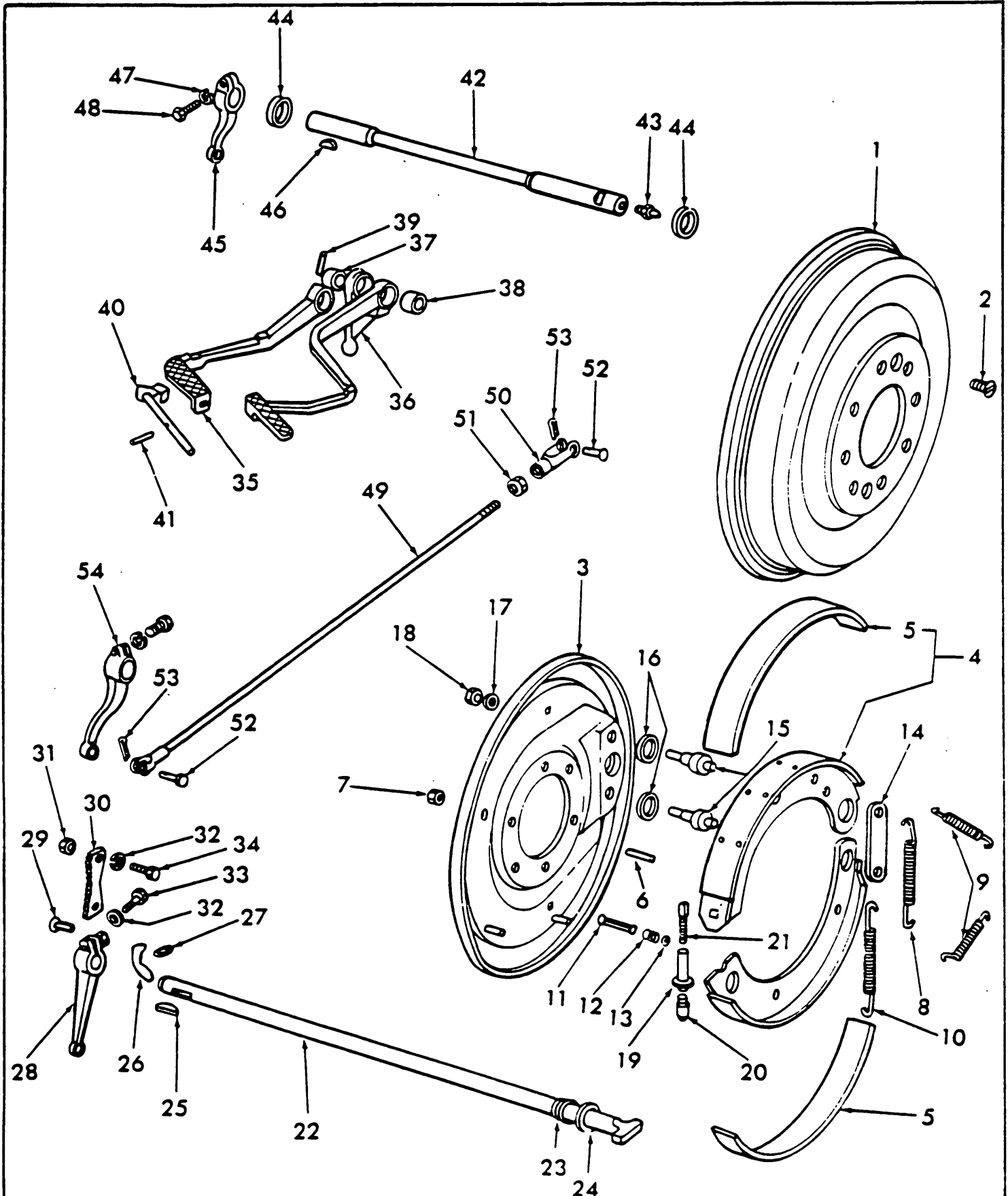
Fig. 2 Brakes
