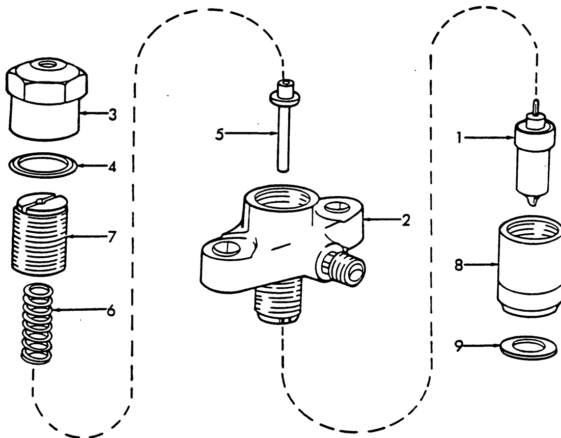
Fig. 44 Fuel Injector Assy.
