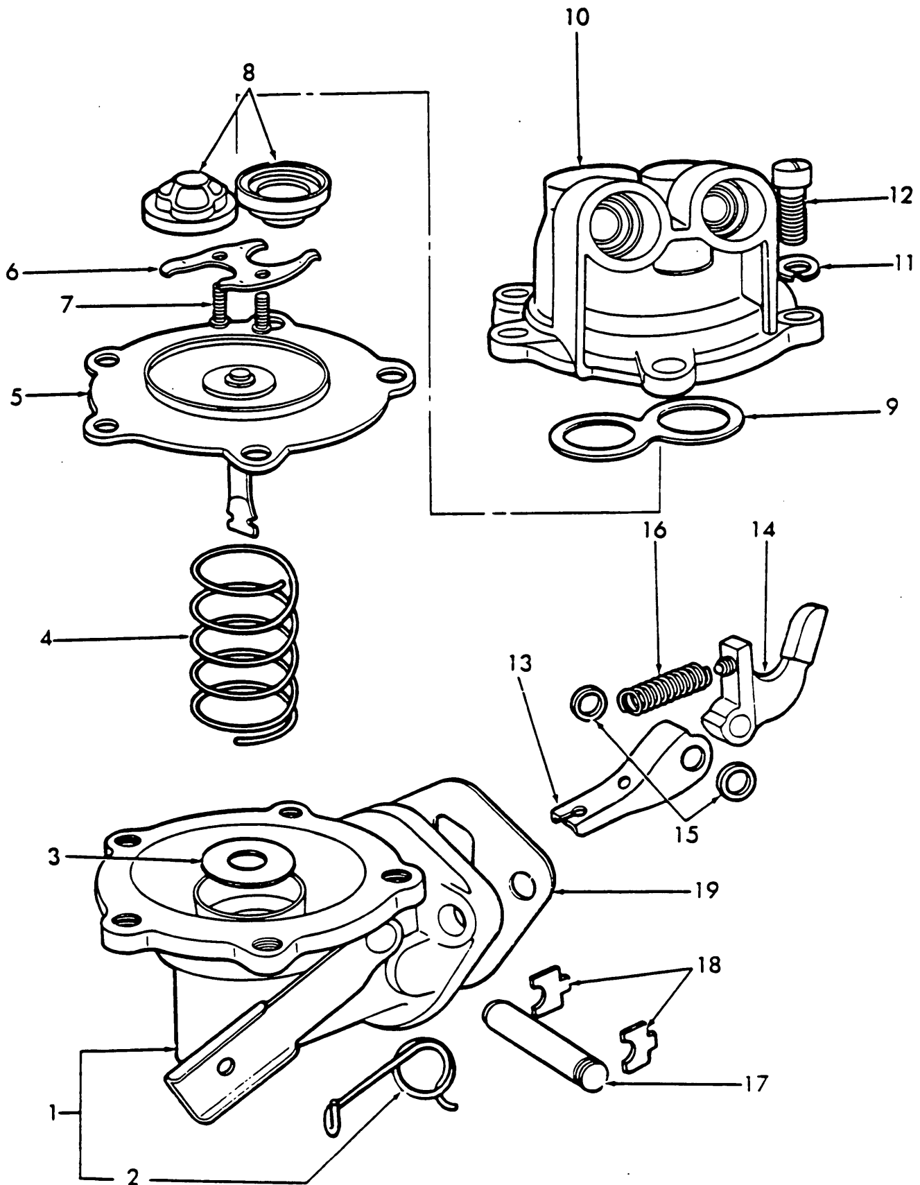
Fig. 45 Fuel Pump Assy.
