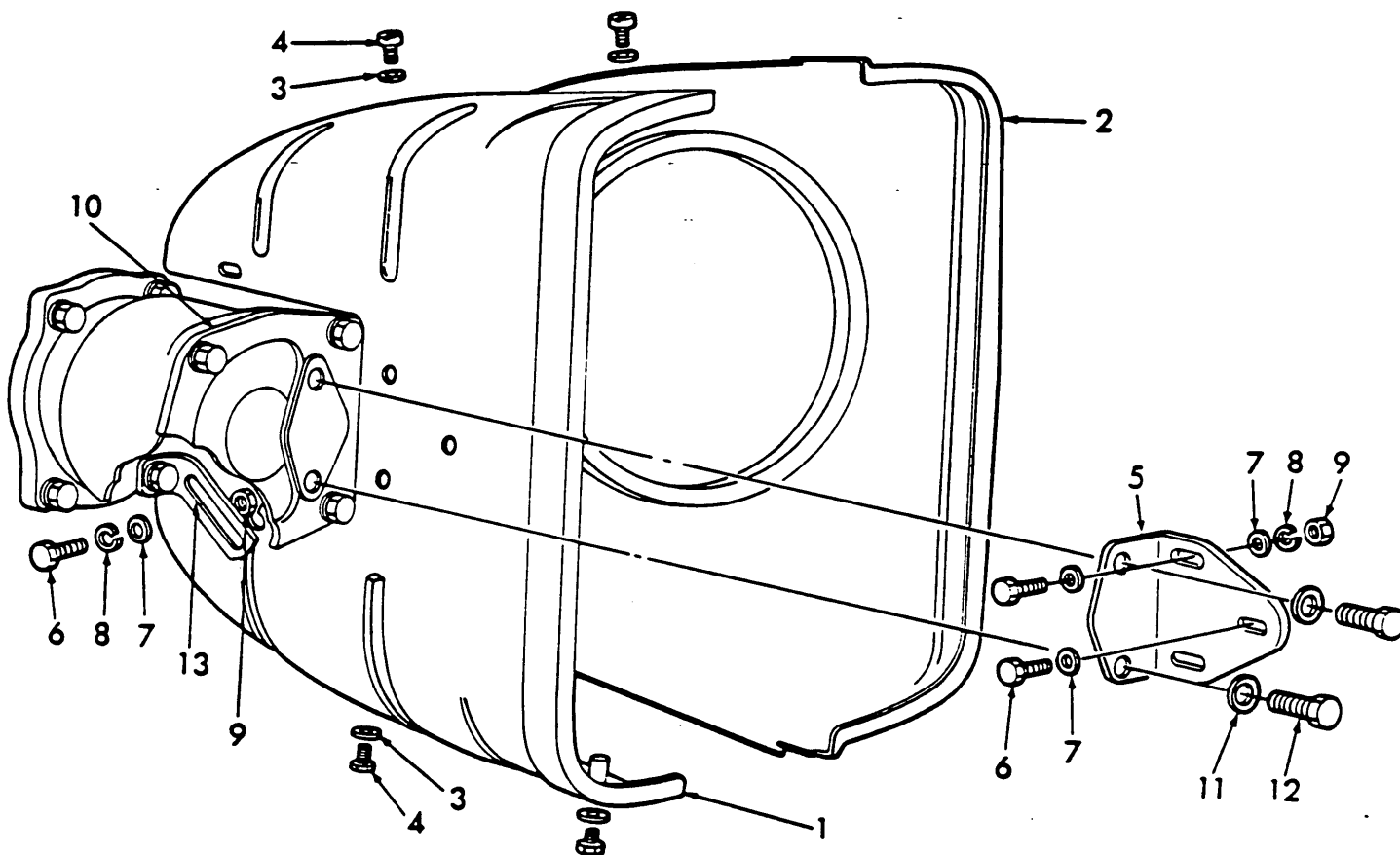
Fig. 34 Pulley Guard
